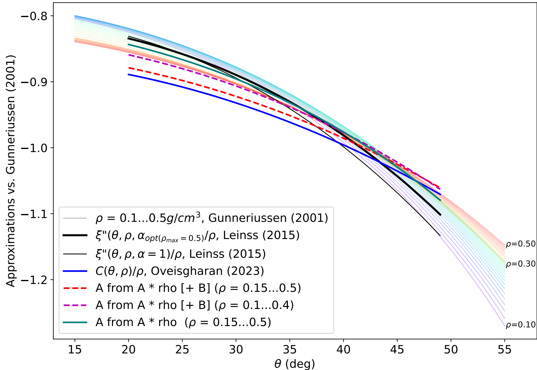
Gunneriussen (2001) ( \cos\theta - \sqrt{\varepsilon(\rho) - \sin^2(\theta)} ) and approximations divided by snow density \rho
