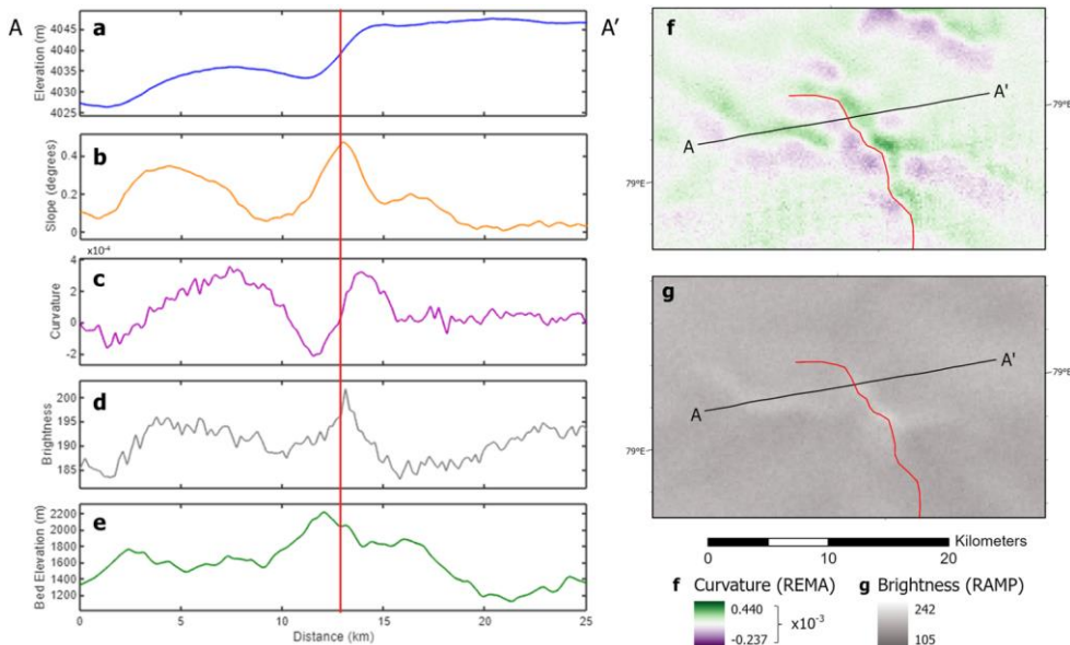
Figure 4 – Profile (A-A') across a typical ice surface feature (red line), demonstrating the correspondence between the location of a bed ridge and its surface expression in the two datasets used for mapping: a) Reference Elevation Model of Antarctica (REMA; Howat et al., 2019) surface elevation; b) REMA surface slope; c) and f) REMA surface mean curvature (second derivative); d) and g) RADARSAT-1 Antarctic Mapping Project version 2 (RAMP; Jezek et al., 2013) brightness (adjusted backscatter intensity); e) Radio Echo Sounding bed elevation, Antarctica's Gamburtsev Province (AGAP) survey (Bell et al., 2011; Ferraccioli et al., 2011; Corr et al., 2020).
