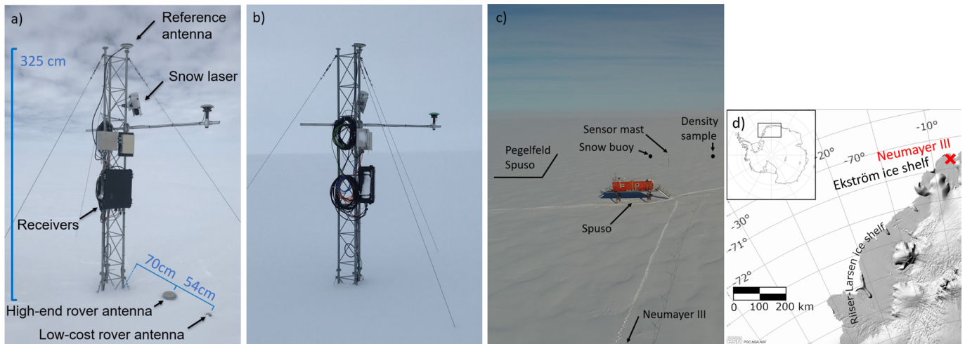
Figure 1. a) The GNSS-RR setup consists of one GNSS reference antenna and two GNSS rover antennas placed on the firn surface (21.11.2021). The rover antennas are physically connected to the sensor mast via a lateral boom (hidden below the snow surface). b) GNSS-RR setup with both rover antennas already covered by the accumulated snow (23.11.2021). c) Situation of the test site. d) Location of the test site at the Ekström ice shelf, Dronning Maud Land, Antarctica (modified from Jakobs et al., 2019).
