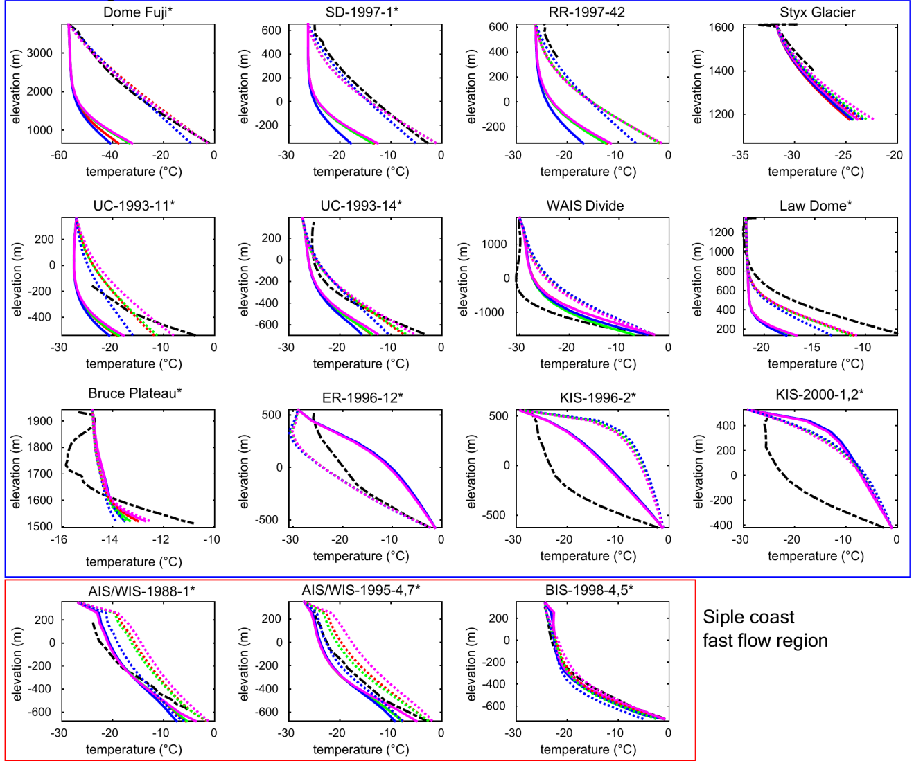
Figure 2. Observed and modeled vertical temperature profiles from eight different experiments at 15 borehole locations. Blue and red boxes indicate slow flow and Siple coast fast flow regions, respectively. The bottom elevation at each borehole is set with considering the ice thickness, as listed in Table 1. An asterisk on borehole name indicates that the drilling reaches the bed rock.
