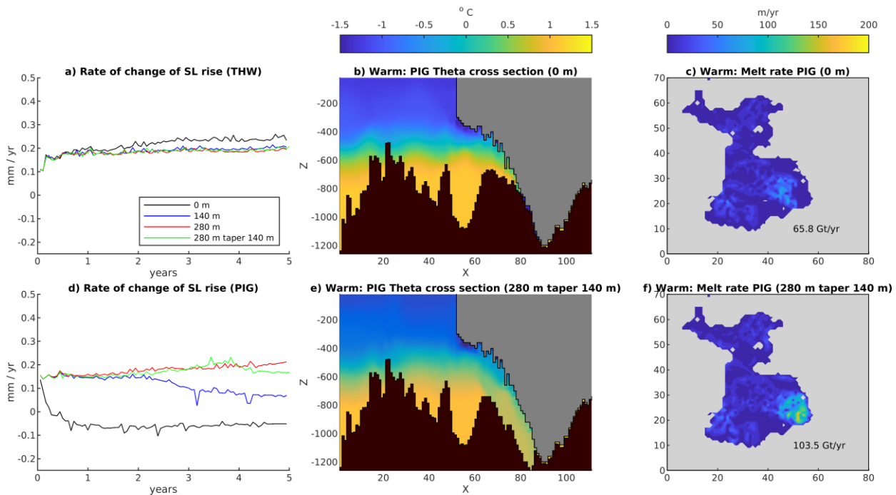
FIGURE B1: a) SLR rate of change for the Thwaites area for: zero deepening, 140 m deepening, 280 m deepening, 280 m deepening taper to 140 m over 6 km.. b) Cross-section through PIG Ice Shelf (taken along the green line shown in Figure 2a) showing initial potential
