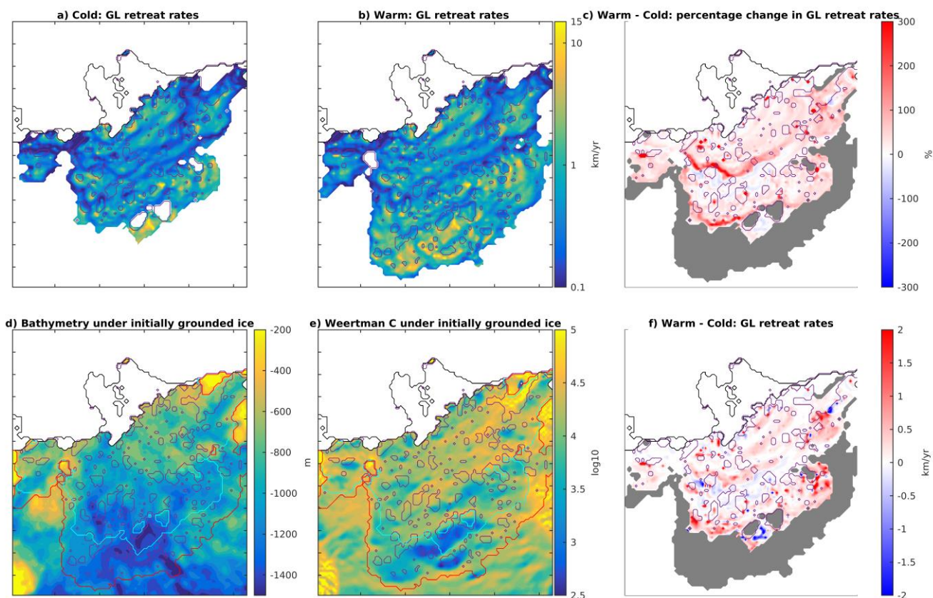
FIGURE 5: (a-b) Grounding line retreat rates over the 180 year simulations in the cold (a) and warm (b) indicated by colours, with colour bar shown in (b). In each the purple contours show the presence of isolated pinning points during the simulation. (c) Percentage change in grounding line retreat rates between the cold and warm cases (i.e., the percentage difference between those retreat rates shown in (a) and (b) respectively). (d-e) Bathymetry (d) and Weertman C coefficient (e) shown under initially grounded ice with final extents of the grounding line retreat in the warm (red) and cold (cyan) cases. (f) The difference in grounding line retreat rates between the cold and warm cases (colours) as well as final grounding line area (grey area). The area shown in each panel corresponds to that displayed as a black box in Figure 3.
