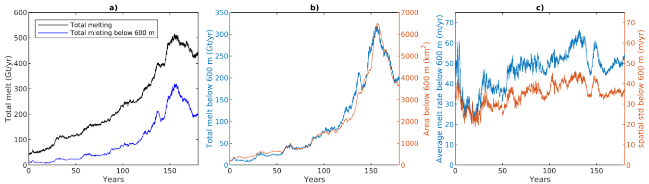
FIGURE 9: (a) Total melt flux from the full Thwaites Ice Shelf area (black) and from grid cells located below 600 m depth only (blue). (b) 435 Total melt flux from grid cells below 600 m and total ice area below 600 m. (c) Average melt rate on grid cells located below 600 m depth and spatial standard deviation of these melt rate values.
