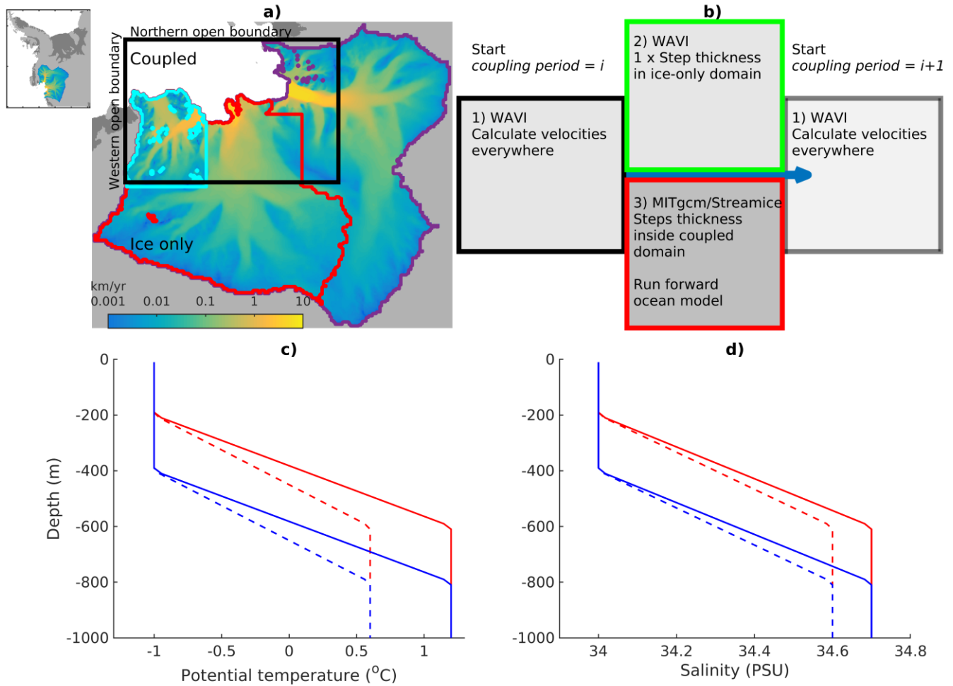
200 FIGURE 1: (a) Outline of the whole Amundsen Sea sector domain. The black box shows the outline of the coupled domain; the ice only domain is defined as everywhere outside of this box. The coloured regions represent the three regions used in analysis: PIG (purple), Thwaites (red), and Smith (cyan). These areas are edited by hand from the Zwally et al. (2012) basins. (b) A schematic diagram of the three grouped steps of the coupled model applied during one coupling period, which are repeated during the coupled simulations. (c) Potential temperature boundary conditions for the Northern (solid line) and Western (dashed line) boundaries for the warm (red) and cold (blue) cases. (d) as in 205 (c) but for salinity.
