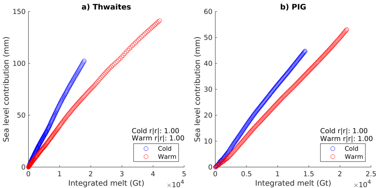
640 FIGURE C1: (a) Yearly points of sea level contribution plotted against integrated melt from the Thwaites area for the warm (red) and cold (blue) forced cases. (b) as in (a), but for the PIG area. In both, correlation coefficients are shown for the warm and cold cases.
