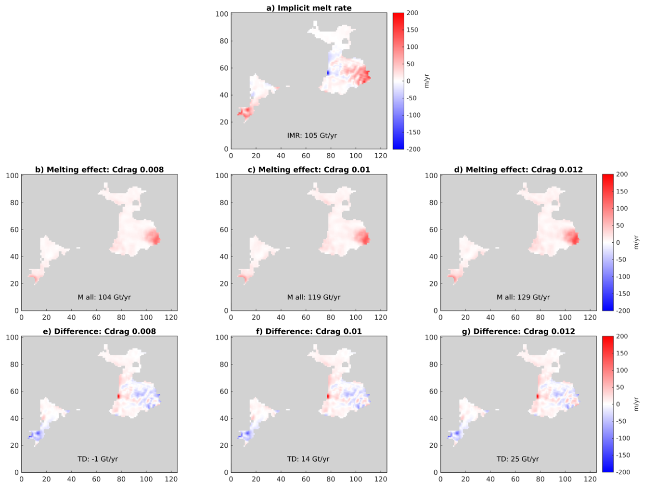
595 FIGURE A1: Area shown for PIG and Thwaites ice shelves. a) Initial implicit melt rate from the WAVI ice sheet model. b) Initial ice shelf melt rate from the MITgcm model for different values of the ice shelf melting drag coefficient as follows (and labelled): 0.008 (b), 0.01 (c), and 0.012 (d).. (e-g) Difference between initial implicit melt rate and initial ice shelf melting for the MITgcm model melt rates shown in panels (e)-(g) respectively.
