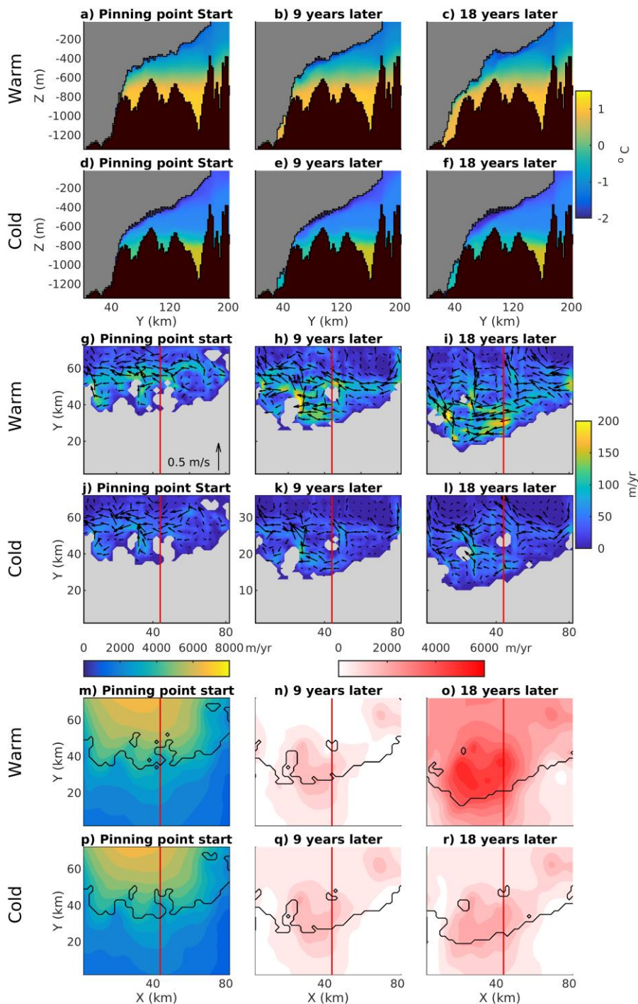
385 FIGURE 7: Evolution of conditions as grounding line retreats over pinning points. Snapshots every 9 years starting from the date of group 'c' pinning point formation in the warm and cold cases (118 and 144 years respectively). (a-c) Cross section through the Thwaites Ice Shelf, taken along the red line in (g) extended to ice front, for warm case. (d-f) Same as (a-c) but for cold case. (g-i) Melt rates for warm case, with
