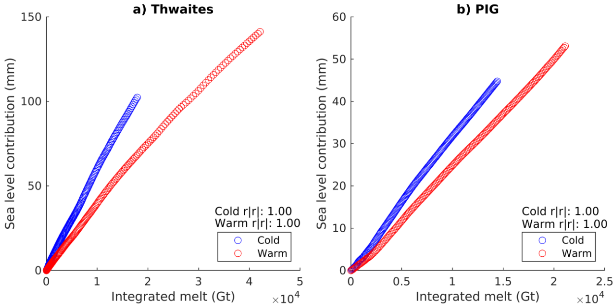
FIGURE DE1: (a) Yearly points of sea level contribution plotted against integrated melt from the Thwaites area for the warm (red) and cold (blue) forced cases. (b) as in (a), but for the PIG area. In both, correlation coefficients are shown for the warm and cold cases.
