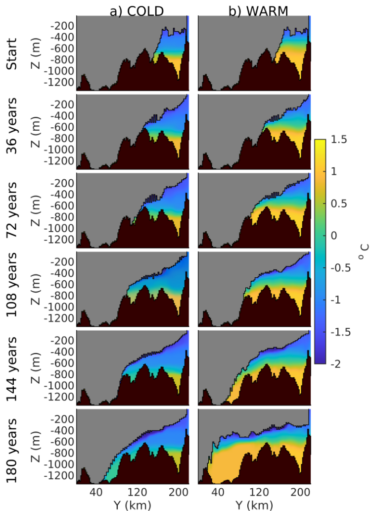
420 FIGURE 8: Cross sections of potential temperature beneath Thwaites Ice Shelf for cold (left) and warm (right) cases, taken every 36 years, 425 along the same section as shown in Figure 7 and Figure 2i, j, which is, represented in Figure 2a as the red line.
