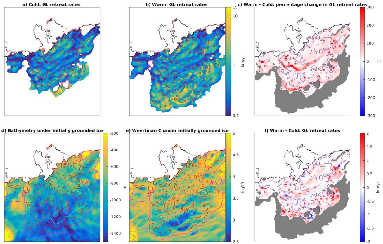
FIGURE 5: (a-b) Grounding line retreat rates over the 180 year simulations in the cold (a) and warm (b) indicated by colours, with colour bar shown in (b). In each the redpurple contours in (a, b, d, e) and the purple contours in (c, f) show the presence of isolated pinning points during the simulation. (c) Percentage change in grounding line retreat rates between the cold and warm cases (i.e., the percentage difference between those retreat rates shown in (a) and (b) respectively). (d-e) Bathymetry (d) and Weertman C coefficient (e) shown under initially grounded ice with final extents of the grounding line retreat in the warm ( magentared ) and cold (cyan) cases. (f) The difference in grounding line retreat rates between the cold and warm cases (colours) as well as final grounding line area (grey area). The area shown in each panel corresponds to that displayed as a black box in Figure 3.
