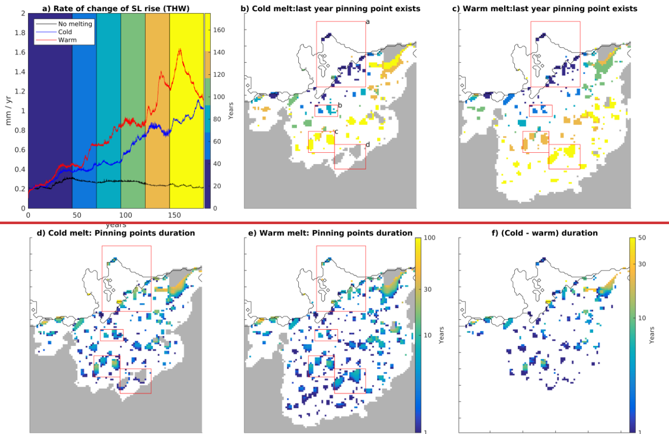
FIGURE 6: (a) SLR contribution rates for Thwaites area for warm (red), cold (blue) and no melt (black) cases. The background colour indicates the time in the simulation according to bands of 25 years, with a longer starting (ending) band of 45 (35) years. (b) Colours indicate the band of the final year that pinning point cells exists for cold melt case, according to the colours shown in (a). Note that only pinning points that exist for over 1 year are shown. Red labelled boxes refer to groups of pinning points discussed in the text. (c) Same as (b) but for warm case. (d-e) Pinning point duration, taken as the time from isolation to ungrounding, for cold (d) and warm (e) cases. (f) Difference in pinning point duration between cold and warm cases (i.e. the difference the data shown in d and e), where pinning point locations match. In (b)-(e), grey regions indicate areas which do not become ungrounded during the simulation. The area shown in Figures b-f is shown with a black box in Figure 3.
