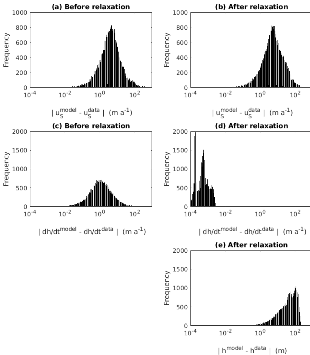
Figure R4: Histograms of the absolute difference between the initial model state and satellite observations on a logarithmic scale. For surface ice speed: (a) before relaxation, (b) after relaxation. For rates of elevation change: (c) before relaxation, (d) after relaxation. For grounded ice thickness: (e) after relaxation, with the model matching observed ice thickness before relaxation by design. Data sets used: ice thickness from Bedmachine V3 (Morlighem et al., 2020; Morlighem, 2022), surface ice speed from Measure 2014/2015 (Mouginot et al., 2017a; Mouginot et al., 2017b), rate of elevation change from Smith et al. (2020).
