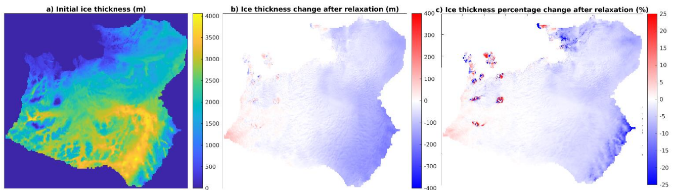
Figure R5: a) Initial ice thickness from the BedmachineV3 dataset (Morlighem et al., 2020; Morlighem, 2022) before relaxation. b) Changes in ice thickness from relaxation step. c) Percentage changes in ice thickness after relaxation step. Both plots shown for the full ice domain.
