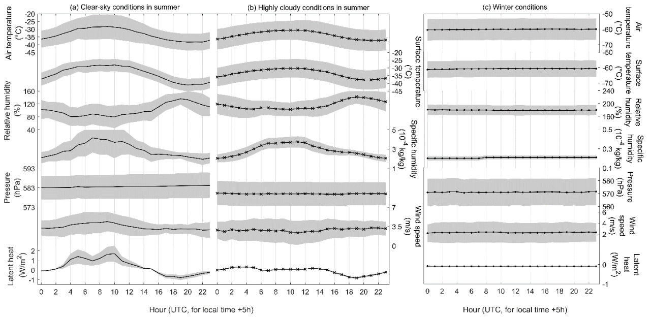
750 Figure 2: Stacks of diurnal cycles of meteorological parameters and the calculated latent heat under summer clear-sky conditions (a), summer highly cloudy conditions (b), and winter conditions (c) at Dome A. The hourly air temperature, relative humidity, air pressure and wind speed data were averaged from the AWS observations on the selected days. The diurnal variations in the other three parameters were calculated based on hourly observations. In each panel, the solid line with marks represents the average and the gray shadow represents the standard deviation ( \pm 1\sigma ).
