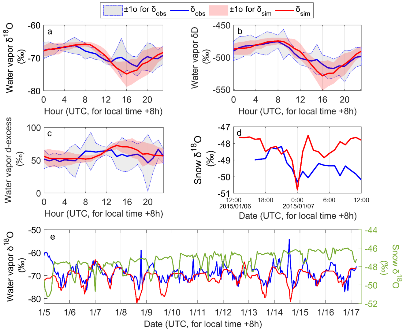
755 Figure 3: Modeled variations in water vapor and snow isotopic compositions at Dome C along with the observations. (a) Diurnal variations in water vapor \delta^{18}\text{O} , (b) diurnal variations in water vapor \delta\text{D} , (c) diurnal variations in water vapor d-excess, (d) diurnal variations in snow isotopes during 6-7 January 2015, and (e) continuous variations in water vapor and snow \delta^{18}\text{O} during 5-16 January 2015. In all panels, the blue solid line represents the observations ( \delta_{\text{obs}} ) with the light gray shaded area as the uncertainties ( \pm 1\sigma ). The red solid line and the light red shaded area depict the simulation ( \delta_{\text{sim}} ) and corresponding uncertainties ( \pm 1\sigma ), respectively. 760 In panel (e), the green solid line represents the modeled snow \delta^{18}\text{O} . Note that snow \delta^{18}\text{O} observations at Dome C are available only from 6 to 7 January 2015 (Casado et al., 2018). The method for uncertainty estimation can be found in supplementary (Texts S2).
