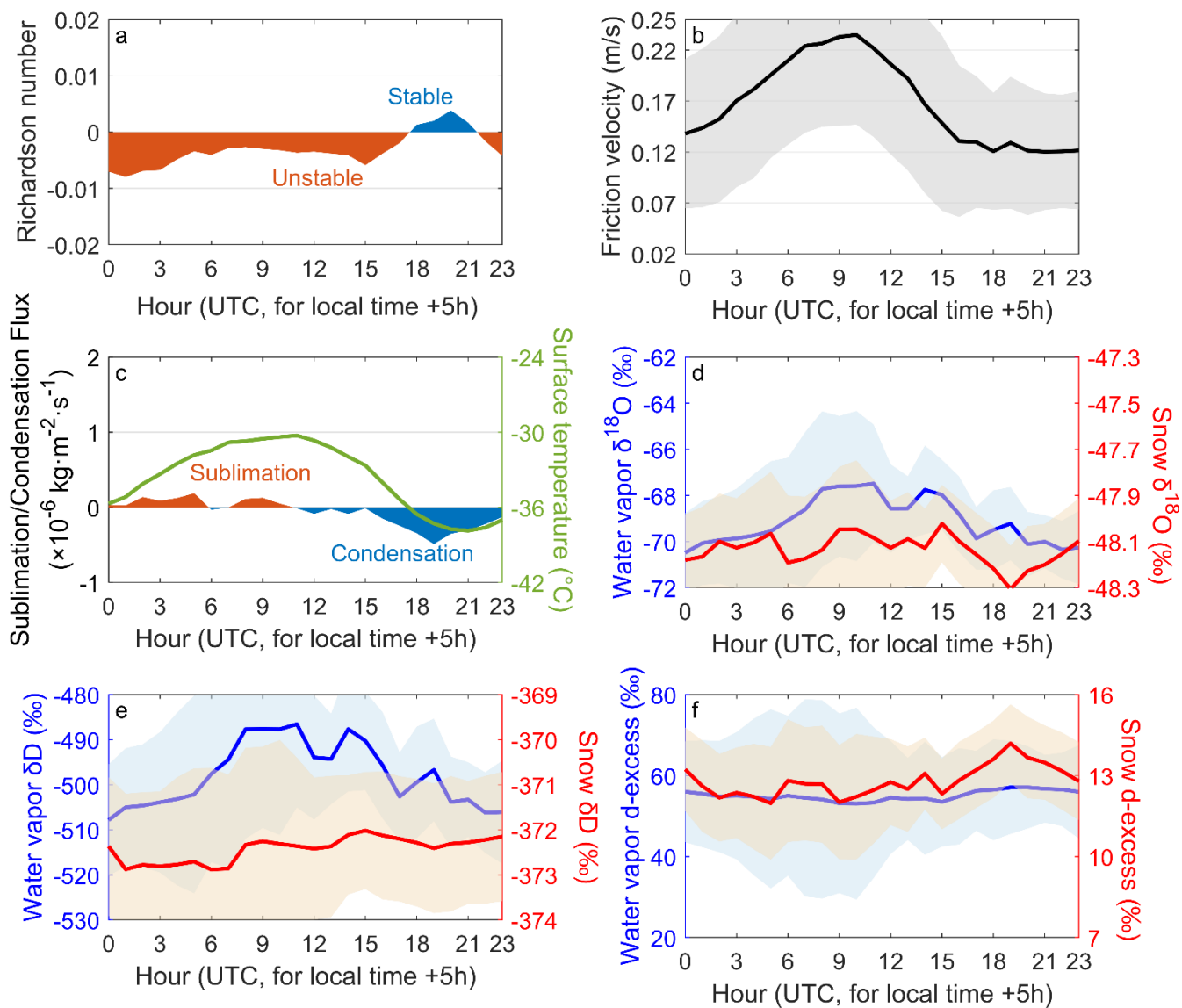
770 Figure 5: Same as Figure 4 but for Dome A under highly cloudy conditions in summer.
