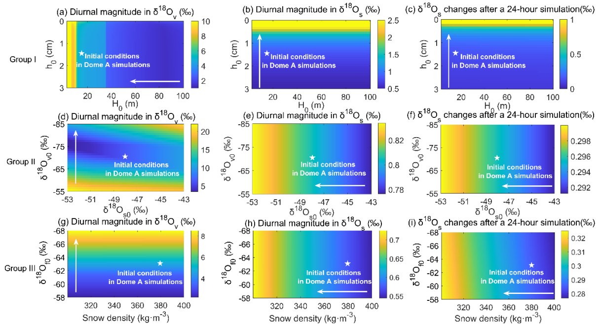
785 Figure 8: Sensitivity of the modeled results to changes in initial conditions. Panels 8a-8c display the modeled magnitude of \delta^{18}\text{O} diurnal variations in water vapor ( \delta^{18}\text{O}_v ), the modeled magnitude of \delta^{18}\text{O} diurnal variations in surface snow ( \delta^{18}\text{O}_s ), and \delta^{18}\text{O}_s differences between the ending and starting values varying with different surface snow thicknesses ( h_0 ) and boundary layer heights ( H_0 ). Panels 8d-8f show the sensitivities of the simulated results to changes in initial water vapor ( \delta^{18}\text{O}_{v0} ) and surface snow isotopic composition ( \delta^{18}\text{O}_{s0} ), respectively. Panels 8g-8i are the same as 8d-8f, but show the sensitivities to changes in the water vapor isotopic composition of free atmosphere ( \delta^{18}\text{O}_{f0} ) and snow density ( \rho_s ). In each subpanel, the white star indicates the initial conditions used in the Dome A simulations with summer clear-sky conditions. The white arrows correspond to the direction of the simulated results with the higher sensitivity. 790
