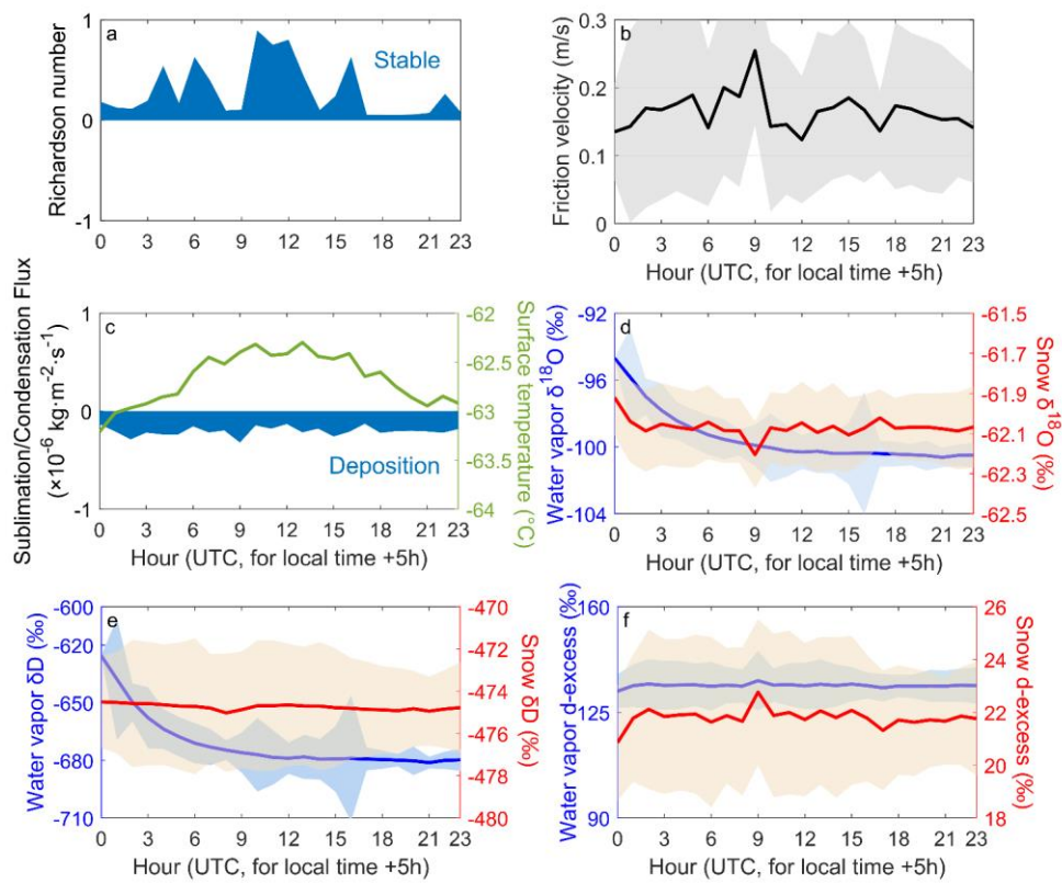
835 Figure 6: Same as Figure 4 but for Dome A under winter conditions.
