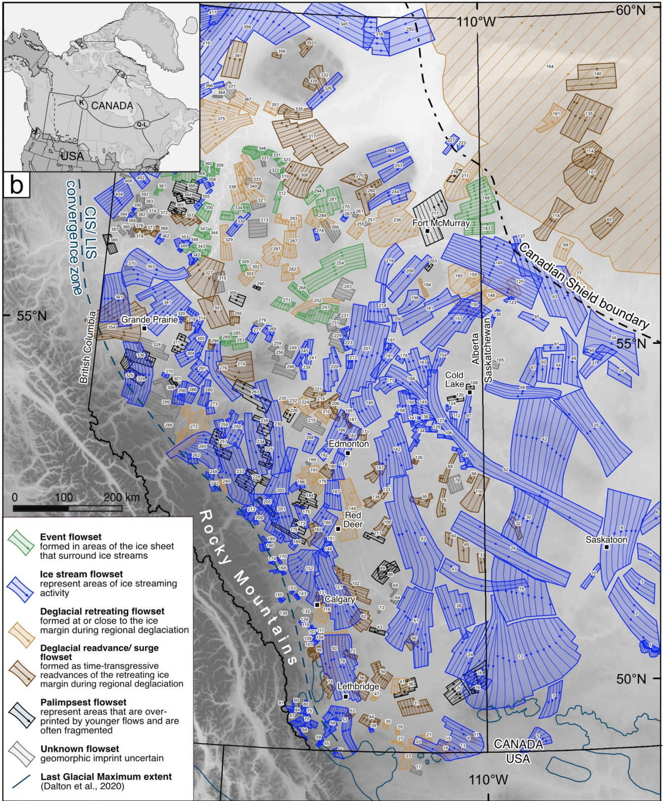
Figure 3: (a) Location of previous flowset mapping. (b) Flowset map of the southwestern Laurentide Ice Sheet (available as a supplementary .kml file). Digital elevation model (DEM) from the Shuttle Radar Topographic Mission (SRTM) provided by the USGS EROS Archive (EROS Centre, 2018). Last Glacial Maximum ice extent from Dalton et al. (2020).
