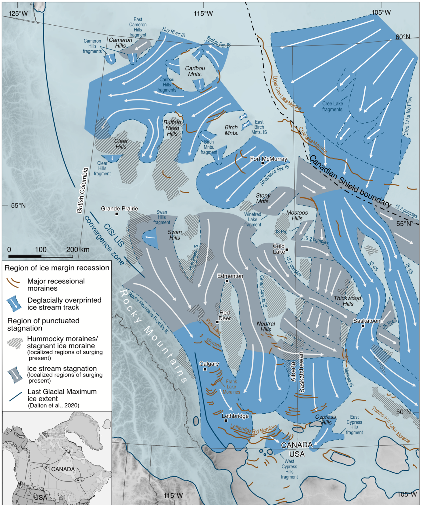
Figure 5: Regional geomorphic imprint of the distribution of ice sheet active retreat and punctuated stagnation across the southwestern Laurentide Ice Sheet. Digital elevation model (DEM) from the Shuttle Radar Topographic Mission (SRTM) provided by the USGS EROS Archive (EROS Centre, 2018). Last Glacial Maximum ice extent from Dalton et al. (2020).
