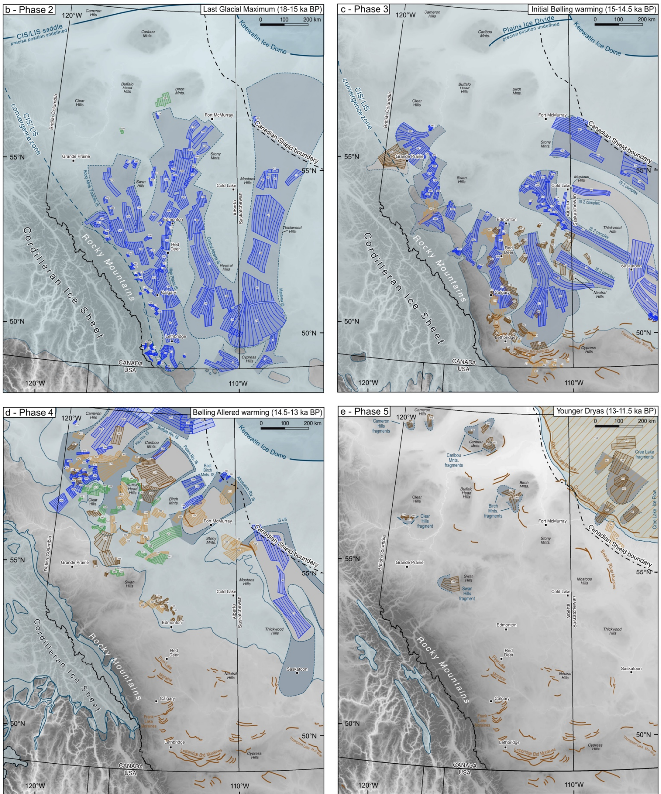
Figure 4: Deglacial ice flow dynamics of the southwestern Laurentide Ice Sheet. This reconstruction presents a comprehensive synthesis, collating pre-existing ice stream mapping with ice streams presented in this study. Timing of ice retreat and associated ice flow reorganizations are constrained using the deglacial chronology of Norris et al. (2022). Digital
