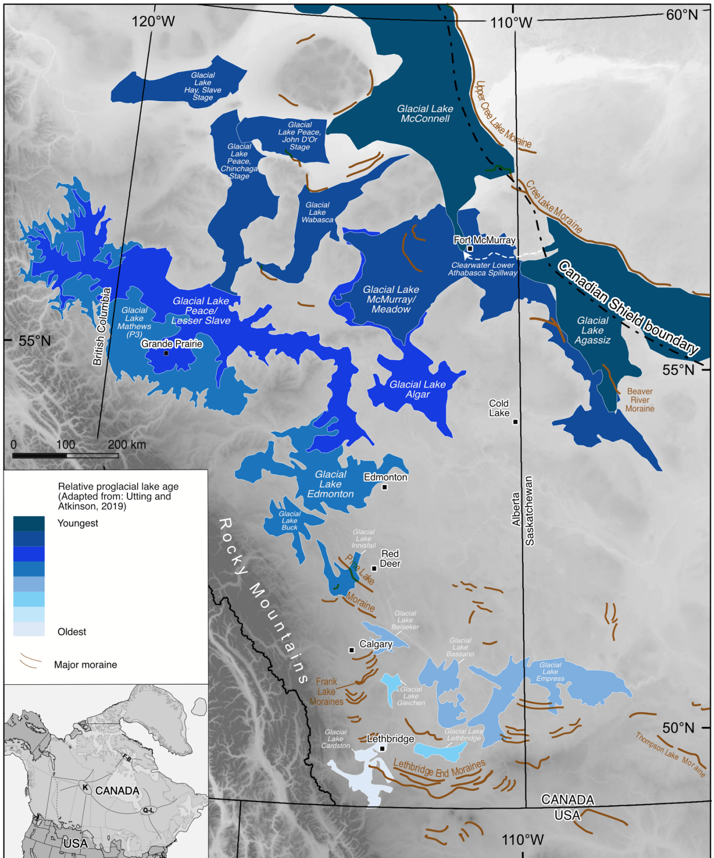
Figure 6: Distribution of reconstructed proglacial lakes associated with the retreat of the southwestern Laurentide Ice Sheet, classified by relative age adapted from Utting and Atkinson (2019). Digital elevation model (DEM) from the Shuttle
