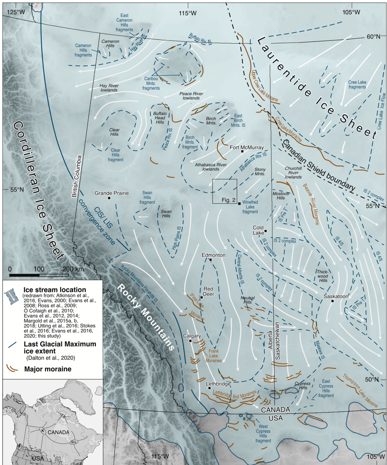
Figure 1: Regional ice-flow imprint of the southwestern sector of the Laurentide Ice Sheet. Digital elevation model (DEM) from the Shuttle Radar Topographic Mission (SRTM) provided by the USGS EROS Archive (EROS Centre, 2018). Last Glacial Maximum ice extent from Dalton et al. (2020).
