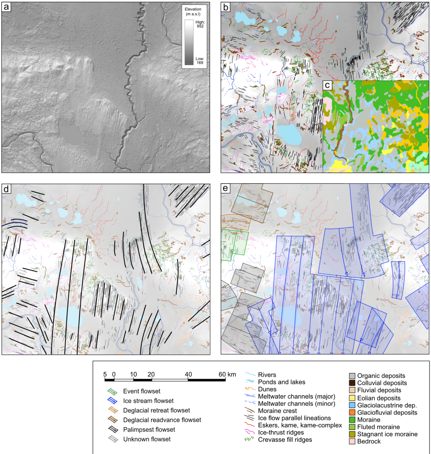
Figure 2: Classification of glacial geomorphology into flowsets. (a) Imagery displaying the onset zone of the Central Alberta Ice Stream. (b) Area of corresponding geomorphological mapping (Atkinson et al., 2018) and, (c) surficial geology (Fenton et al., 2013) (d). Simplification of the geomorphic imprint into flowlines, and (e) flowsets. Flowsets were categorized as either ‘ice stream’, ‘deglacial retreat’, ‘deglacial readvance’ ‘event’ ‘palimpsest’ or ‘unknown’ after Kleman (2006). See Figure 1 for the location of Figure 2 panel. Digital elevation model (DEM) from the Shuttle Radar Topographic Mission (SRTM) provided by the USGS EROS Archive (EROS Centre, 2018).
