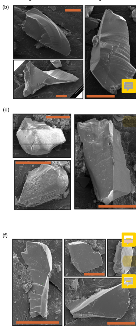
Figure 7. Visualization of grain shape evolution. (a), (c), and (e) show grain circularity for supra-englacial reference material in comparison to glacial-marine diamicton, till, and meltwater plume deposits from a neighboring glacial system. SEM images of (b) cryoconite, (d) basal fringe debris, and (f) basal ice debris show highly fractured and elongated grains that are less common following subglacial transport. Note that in (c) the middle violin includes samples from ice-proximal diamicton from offshore Pine Island and Thwaites glaciers, as well as subglacial till samples from Pine Island Glacier (Table A1). Scale bar in (b), (d), and (f) is 20 microns.
