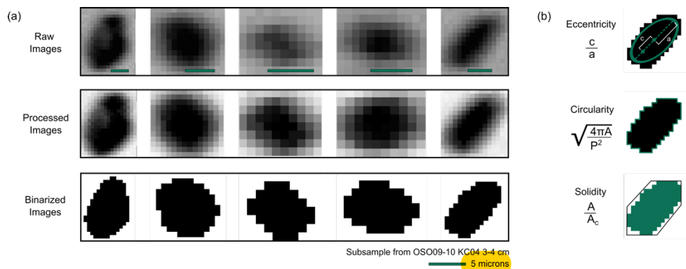
Figure 2. Workflow for automated grain shape analysis. (a) Raw images captured by the Betersizer S3 Plus, images post-processing, and in binarized forms. (b) Metrics and associated equations calculated for each grain. c = distance between ellipse foci and center; a = length of semi-major axis; A = area, P = perimeter, A_c = area of the convex that encompasses the grain.
