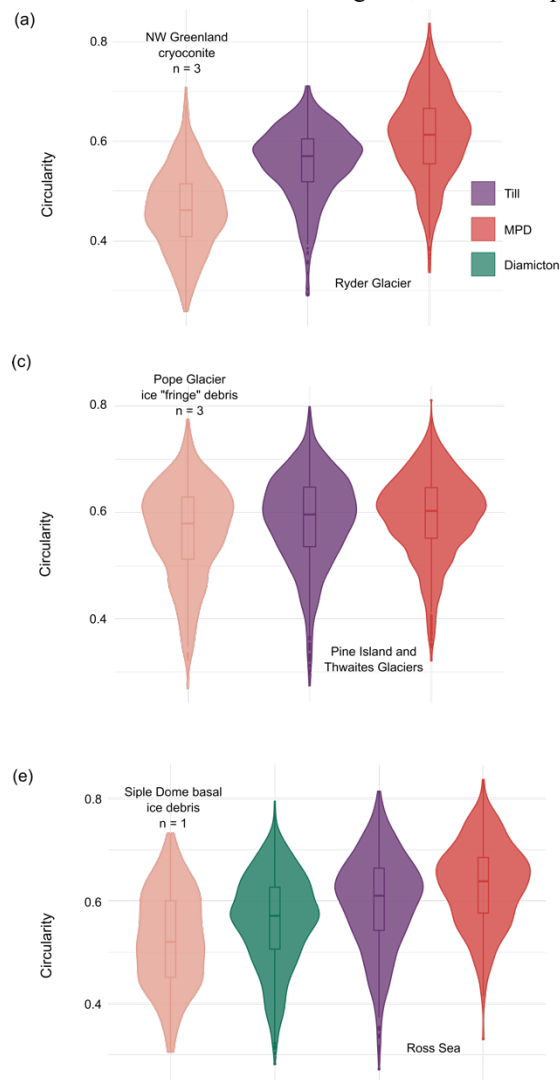
Figure 7. Visualization of grain shape evolution. (a), (c), and (e) show grain circularity for supra-englacial reference material in comparison to glacial-marine diamicton, till, and meltwater plume deposits from a neighboring glacial system. SEM images of (b) cryoconite, (d) basal fringe debris, and (f) basal ice debris show highly fractured and elongated grains that are less common following subglacial transport. Note that in (c) the middle violin includes samples from ice-proximal diamicton from offshore Pine Island and Thwaites glaciers, as well as subglacial till samples from Pine Island Glacier (Table A1). Scale bar in (b), (d), and (f) is 20 microns.
