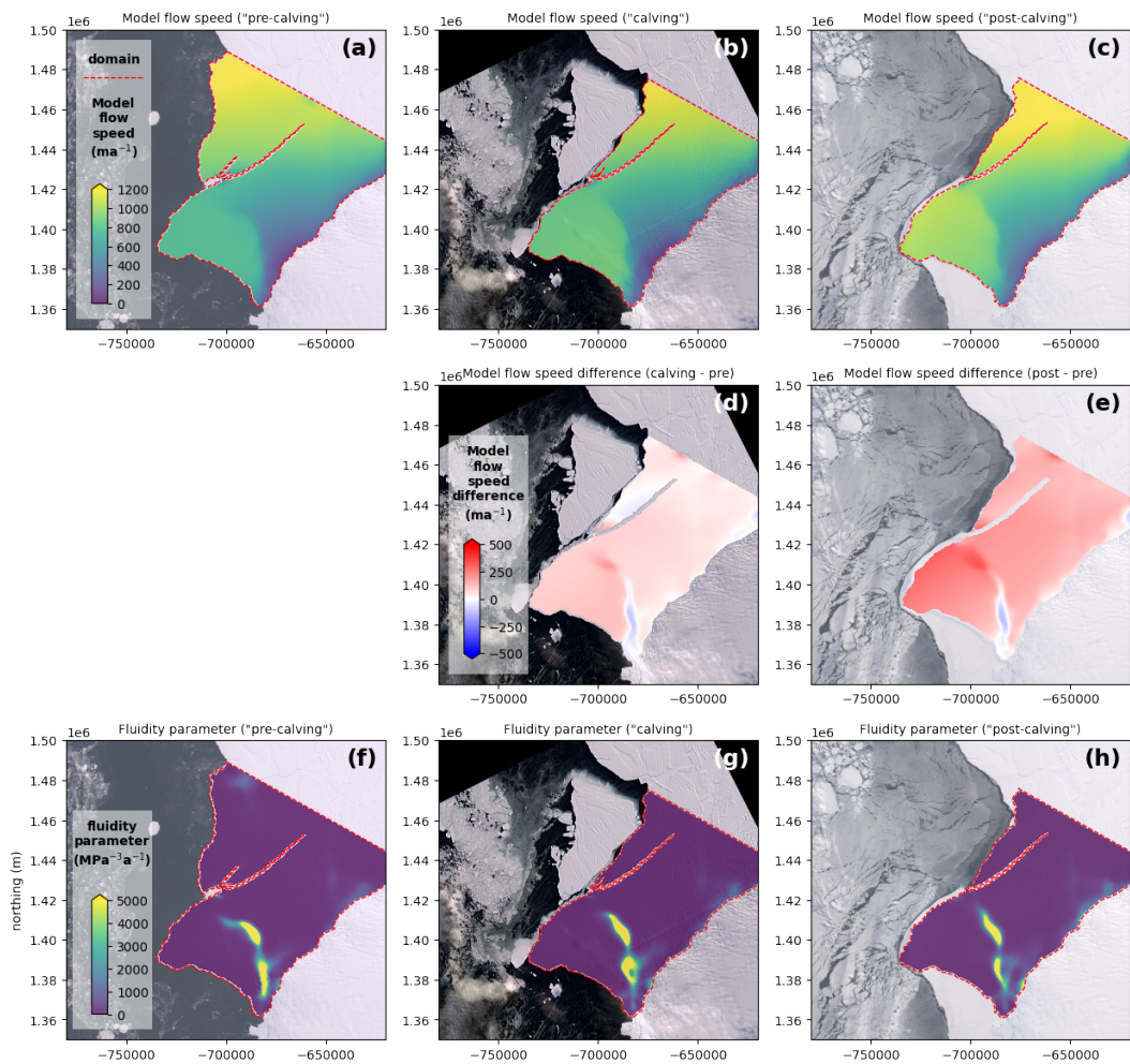
Figure 17. icepack model outputs. (a–c) Modeled ice flow speed. (d, e) Modeled ice flow speed change compared to prior to calving from NR. (f–h) Modeled fluidity parameter.
