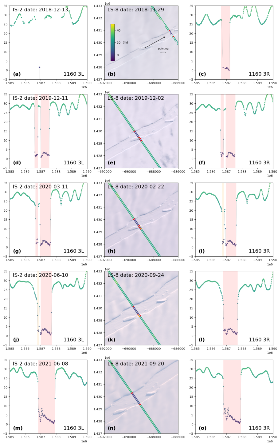
Figure 9. Example detections used in Fig. 4a and c along RGT 1160 3LR. High confidence rift measurements are shown in light red, lower confidence measurements in light orange. Note the ICESat-2 pointing error on 2018-12-13.
