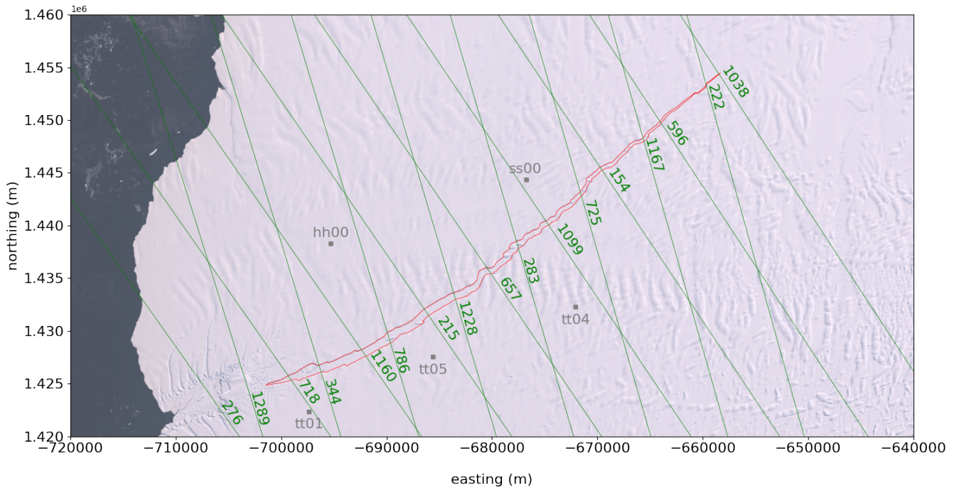
Figure 2. Centers of the nadir beam pair of 17 reference ground tracks (green, numbered), along Halloween Crack (red), on a Landsat-8 OLI image from 2020-02-20. Gray squares show the 2018-02-15 locations of the four GNSS receivers used in this study (the “western pair”: hh00 and tt05, and the “eastern pair”: ss00 and tt04) and unused GNSS receiver tt01.
