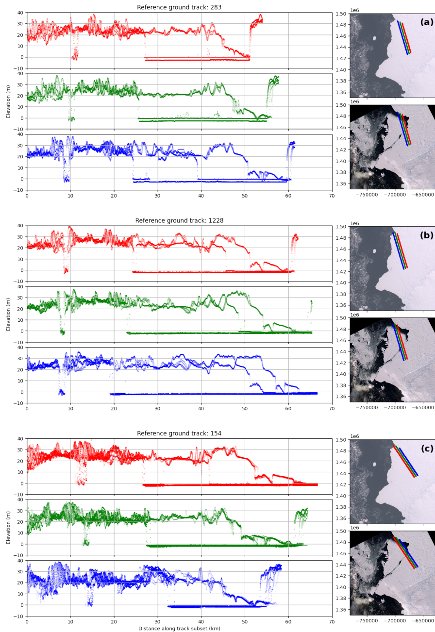
Figure 18. Cycle 5 to 15 SlideRule ICESat-2 elevations along RGTs which cross the calving fronts before and after calving from NR, for (a) RGT 283 (b) RGT 1228 (c) RGT 154. Red, green and blue denote different beam pairs, with strong and weak beams within each pair combined. Cycles are denoted by different color intensity, with intensity increasing with time.
