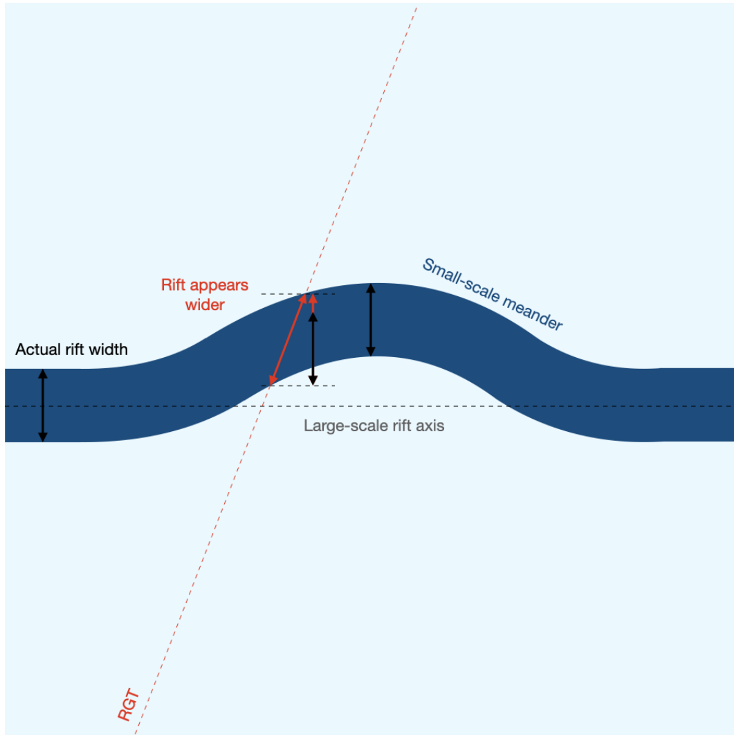
Figure 6. Schematic demonstrating the effect of small-scale meanders, caused by rift propagation between meteoric ice blocks (De Rydt et al., 2018; King et al., 2018), on rift width measurement. This is the situation for HC between the eastern pair of GNSS receivers, and may account for the occasional overestimation of rift width in Fig. 5. Red arrows show the measured rift width along the RGT and component perpendicular to the large-scale rift axis, compared to the actual rift width (black arrows).
