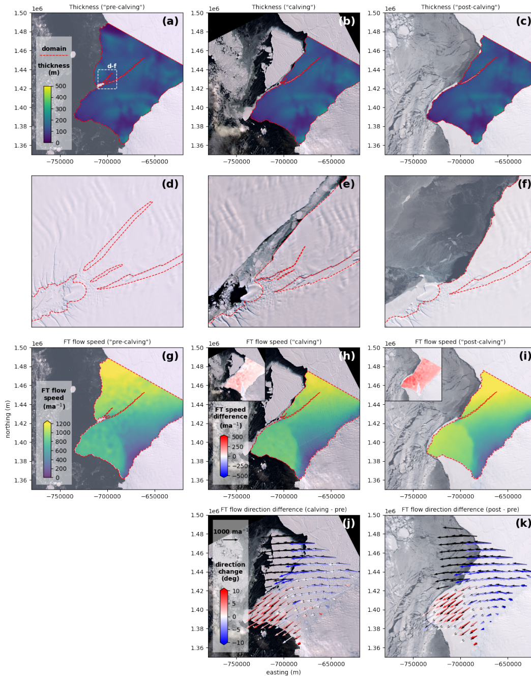
Figure 16. icepack model inputs. (a–c) Ice shelf thickness DEM cropped to the “pre-calving”, “calving” and “post-calving” domains (dashed red lines). Dashed white box in a show the location of d–f. (d–f) Fractures in the vicinity of McDonald Ice Rumples in the 3 domains. d includes the ~13 km-long beginning of North Rift. (g–i) Ice flow speed from feature tracking of Sentinel-1 SAR scene pairs. Insets show ice flow speed change compared to prior to calving from NR, demonstrating an increase in ice flow speed. (j, k) Ice flow direction and magnitude change compared to prior to calving. Black arrows show “pre-calving” velocity, colored arrows show “calving” (j) and “post-calving” (k) velocity, highlighting acceleration and angular change in flow direction (red shows clockwise redirection of flow, blue shows anti-clockwise redirection of flow).
