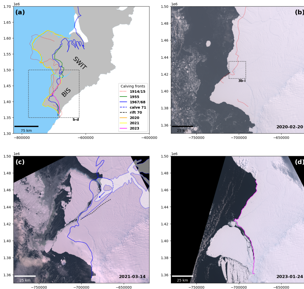
Figure 2. (a) Ice front position of BIS and SWIT between 1914/15 and 2023 from satellite imagery and Thomas (1973). (b) The 2020 front (Landsat-8 image courtesy of U.S. Geological Survey) compared to the 1914/15 (red) position from HMS Endurance (digitised from Thomas, 1973). Dashed box shows the location of imagery subsets in Fig. 3b-i. (c) Iceberg calving (A-74) from NR and HC position in February 2021 (Copernicus Sentinel-2 data [2021]), compared to 1967/68 front (blue), rift (dashed black) and area which calved in 1971 (dashed blue) (all digitised from Thomas, 1973)). White area shows parts of the 1967/68 shelf composed of sea ice. Blue arrow shows a potential partial rift. (d) Iceberg calving (A-81) from Chasm 1 on 2023-01-22 (Copernicus Sentinel-2 data [2023]).
