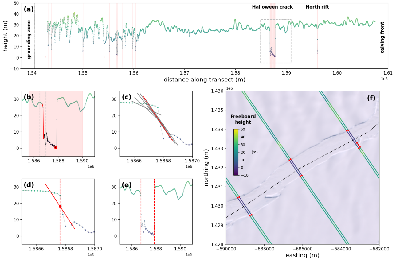
Figure 4. Example rift detection and measurement along RGT 215 1L on 2021-01-07. (a) ICESat-2 ATL06 transect with potential rifts shown as light red bars. Dashed box around HC shows the extent of b and e. (b) Expanded search area (light red box) centered on the lowest point in the rift (red circle). The mostly likely rift wall (red) is selected from the possibilities (black). Dashed box shows the extent of c and d. (c) The steepest section of the rift wall (red line) is selected from measurements of slope along 200 m sections (gray lines). (d) The location of the rift wall (dashed red line) is defined as the average location of points in steepest section (red line). (e) The process is repeated for the opposite rift wall. (f) Rift detections (red circles) along the six beams of RGT 215 overlaid on a Landsat-8 image from the same day. The dashed line traces the manually-defined large-scale rift axis, which does not follow all small-scale variability in the rift, and is used to convert oblique measurements of apparent width in ICESat-2 RGT geometry to estimated rift width perpendicular to the large-scale rift axis. The same elevation colorbar is used throughout.
