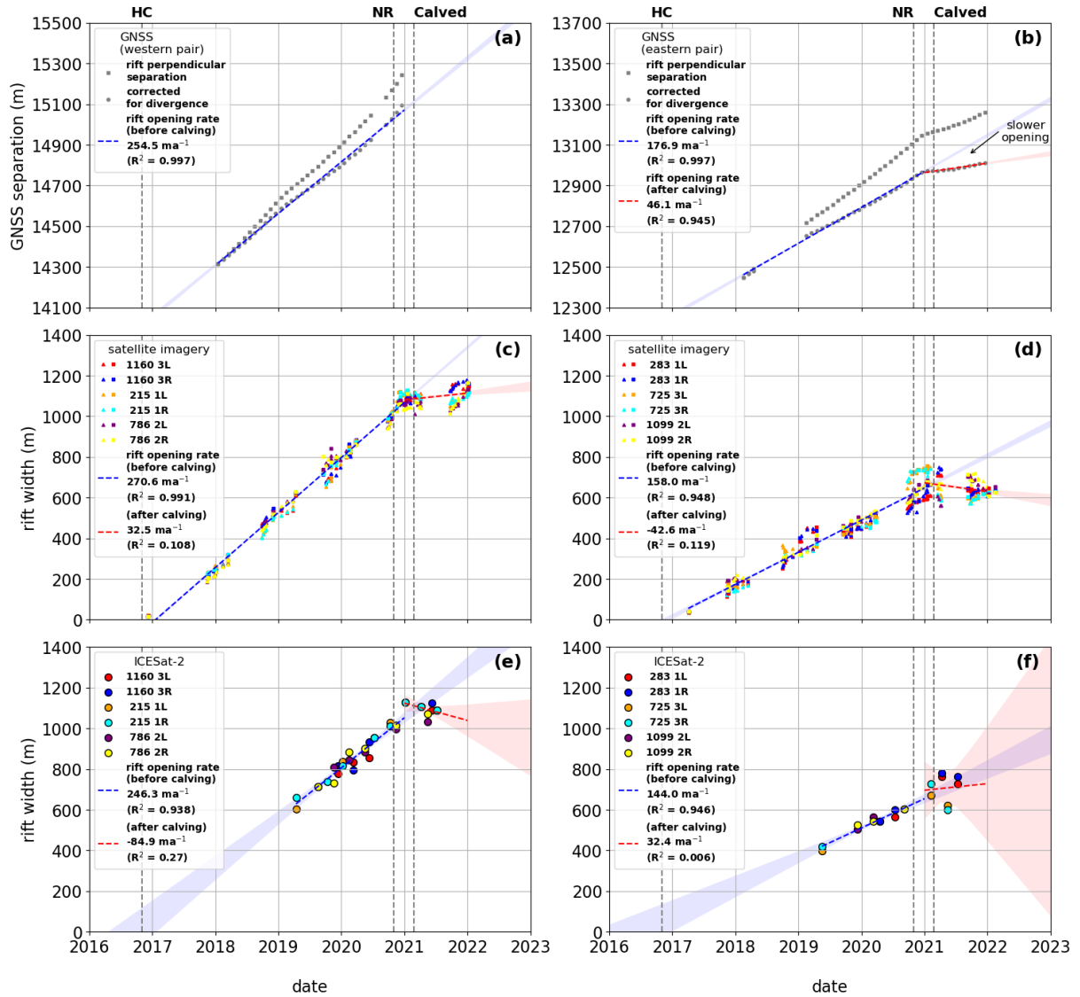
Figure 7. Independent estimates from the three datasets of the rates of HC opening in the vicinity of the GNSS pairs before and after calving from NR. (a, b) Time series of the component of the separation of the pairs of GNSS receivers perpendicular to the local rift axis (gray squares) and corrected for divergence (gray circles). (c) Combined time series of HC width from WorldView-1-3 (squares) and Landsat-8 (triangles) for RGT 215 1LR, RGT 1160 3LR, and RGT 786 2LR. (d) As c for RGT 283 1LR, RGT 725 3LR and RGT 1099 2LR. (e) Combined time series of HC width from ICESat-2 (circles) for RGT 215 1LR, RGT 1160 3LR, and RGT 786 2LR. (f) as e for RGT 283 1LR, RGT 725 3LR and RGT 1099 2LR. Point colors in c and e correspond to Figs. 1c and 5, point colors in d and f correspond to Figs. 1d and 6. Dashed lines show rates of HC opening before (blue) and after (red) 2021-01-01 using a linear fit. Light blue and red regions show corresponding 95 % confidence intervals.
