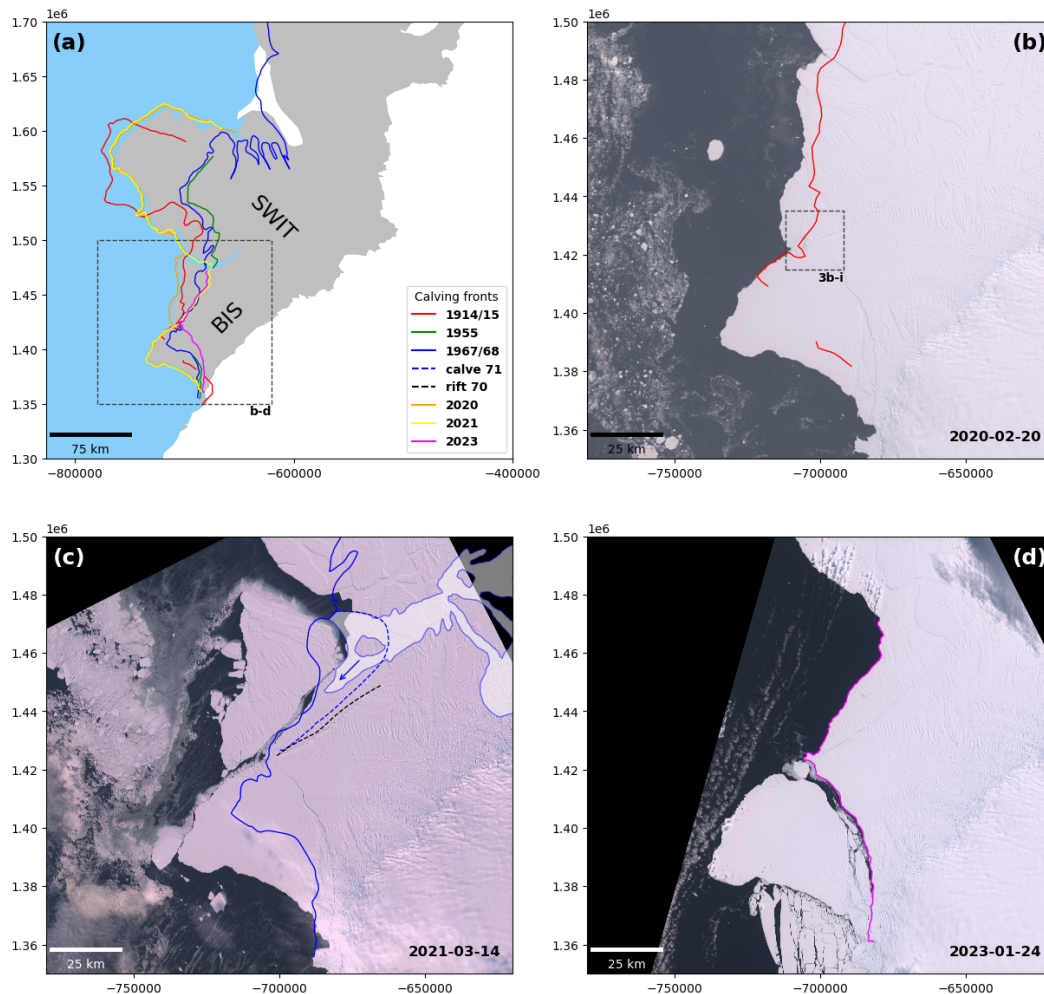
Figure 2. (a) Ice front position of BIS and SWIT between 1914/15 and 2023 from satellite imagery and Thomas (1973). (b) The 2020 front (Landsat-8 image) compared to the 1914/15 (red) position from HMS Endurance (digitised from Thomas, 1973). Dashed box shows the location of imagery subsets in Fig. 3b-i. (c) Iceberg calving (A-74) from NR and HC position in February 2021 (Copernicus Sentinel-2 data [2021]), compared to 1967/68 front (blue), rift (dashed black) and area which calved in 1971 (dashed blue) (all digitised from Thomas, 1973)). White area shows parts of the 1967/68 shelf composed of sea ice. Blue arrow shows a potential partial rift. (d) Iceberg calving (A-81) from Chasm 1 on 2023-01-22 (Copernicus Sentinel-2 data [2023]).
