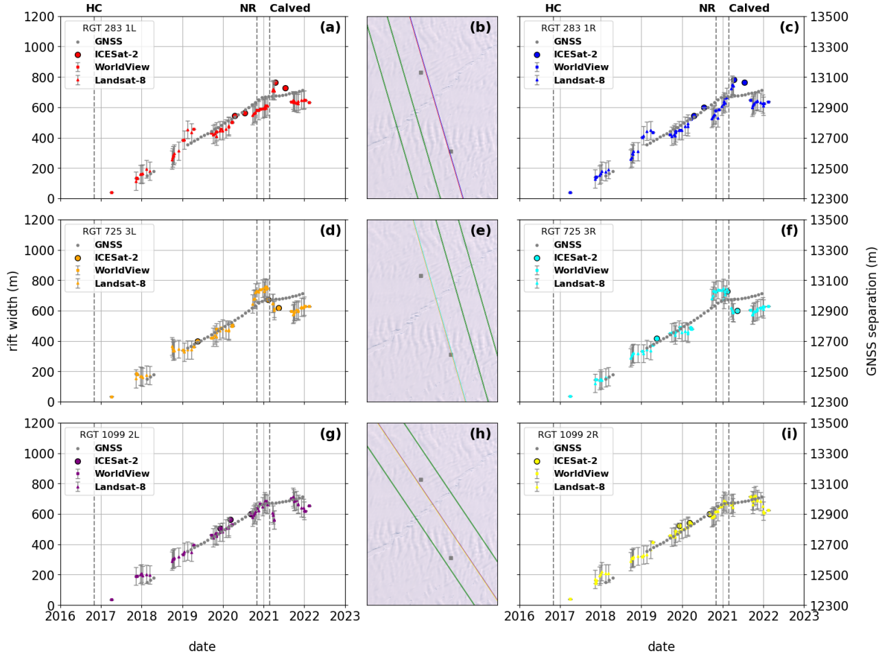
Figure 6. As Fig. 5 for (a–c) RGT 283 1LR, (d–f) RGT 725 3LR and (g–i) RGT 1099 2LR. Colors correspond to the beam colors in Fig. 1d.
