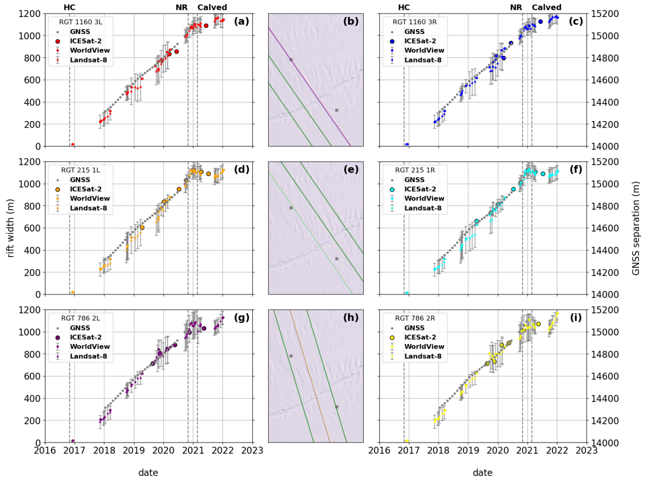
Figure 5. Time series of HC actual widths from the application of the rift measurement algorithm to ICESat-2 ATL06 data (circles), digitization on WorldView-1-3 (squares) and Landsat-8 (triangles) satellite imagery, and the component of the separation of the western pair of GNSS receivers (Fig. 1c) perpendicular to the local rift axis and corrected for divergence (gray circles) for (a–c) RGT 1160 3LR, (d–f) RGT 215 1LR and (g–i) RGT 786 2LR. Colors correspond to the beam colors in Fig. 1c. Error bars on WorldView-1-3 and Landsat-8 points denote a two pixel margin for digitization error, and therefore are twice as large where an ice block bisects the rift. Dashed lines denote the timing of the first observation of Halloween Crack ( HC ), the observation of North Rift propagation ( NR ), and the calving of an iceberg from North Rift ( Calved ). ICESat-2 derived widths from passes with large satellite pointing errors were excluded from this analysis.
