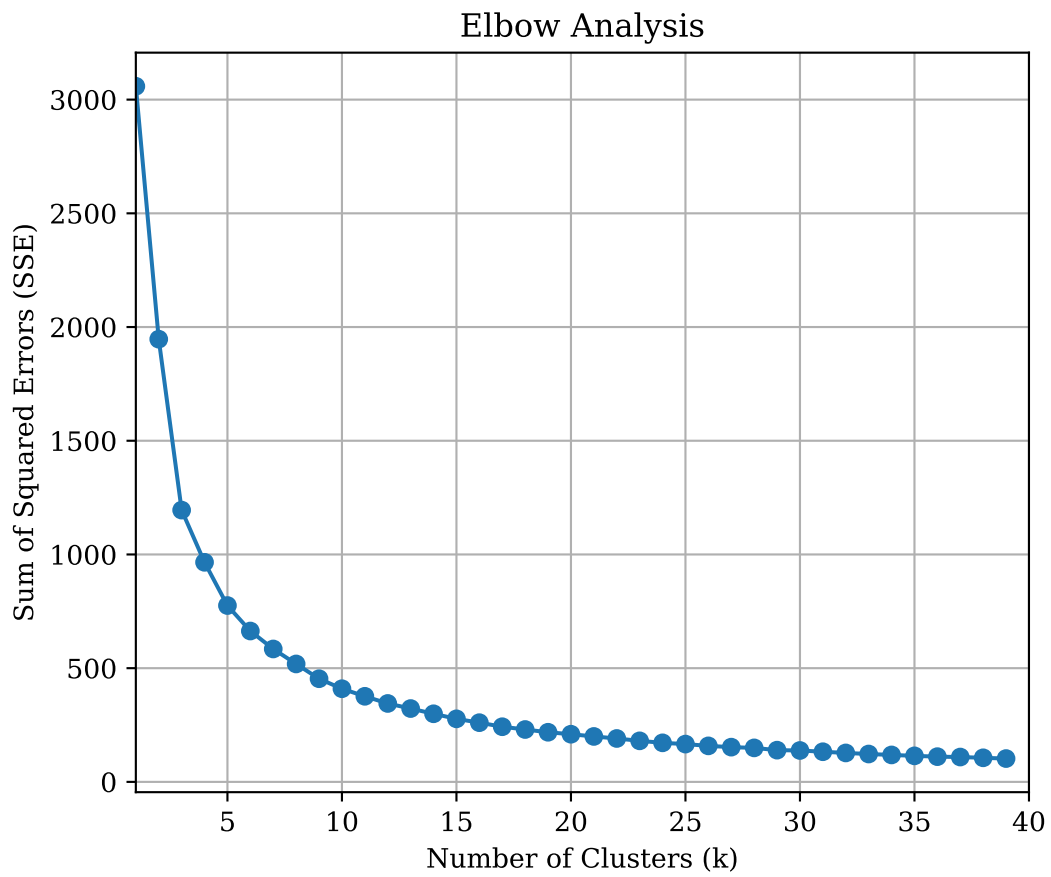
Figure S1. Elbow analysis using different cluster numbers (K) in the K-means algorithm.
