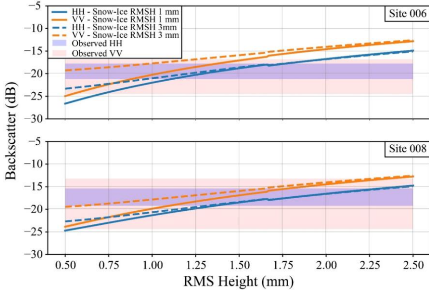
Figure 5. Modelled backscatter for dry snow conditions (IOPI). For the simulations shown only RMS height of the ice-water interface was varied, all other parameters were held constant. Site 006 shows results where no snow ice was found during the field campaign and site 008 shows results where snow ice was found. The shaded parts of the figure represent the minimum/maximum range for the different polarizations.
