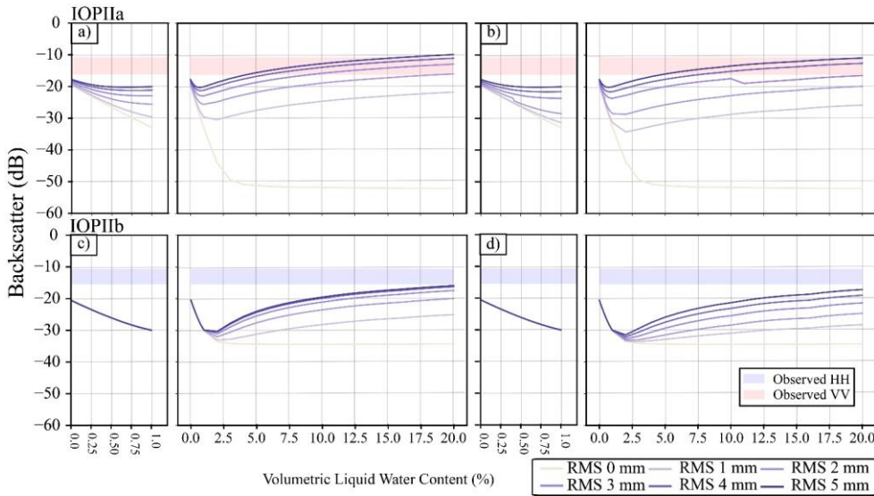
505 Figure 8. Modelled backscatter for site 005 representing IOPIIa, water in the top layer of the snowpack, and IOPIIb, water in the lower layer of the snowpack. For IOPIIa simulations RMSH at the air-snow interface were changed and for IOPIIb RMSH at the interface between snow layers were changed. The different lines represent different values for the RMSH at the top of the snowpack (air-snow interface). The blue and red boxes show the observed backscatter from Sentinel-1. The shaded parts of the figure represent the minimum/maximum range for the different polarizations.
