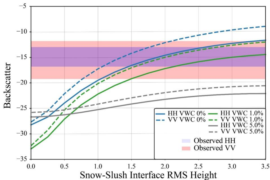
525 Figure 9. Modelled backscatter for site 006 where there is a 0.04 m layer of slush between the lowest snow bottom of the snowpack and the ice surface. All other properties are held constant except the RMSH of the interface between the lowest snow layer and the slush layer. The VWC of the lowest 0.04 m of snow was varied between 0 and 5% The blue and red boxes show the observed backscatter from Sentinel-1. The shaded parts of the figure represent the minimum/maximum range for the different polarizations.
