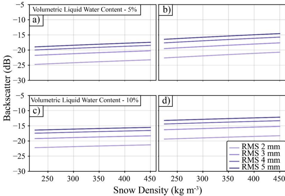
485 Figure 7. Modelled backscatter for site 005 where all layers of the snowpack have the same volumetric liquid water content, the RMSH of the ice-water interface is set to 1 mm and the RMSH of the snow-ice interface is set to 2 mm. The scenario was run for different volumetric liquid water content values and a range of densities. a) and c) show modelled HH results and b) and d) show modelled VV results.
