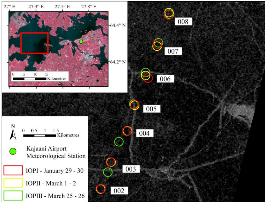
195 Figure 1. In Situ data collection locations on Lake Oulujärvi during the 2020-2021 ice season. The Sentinel-1 image shown was acquired January 29 aligning with IOPI. The area of high backscatter on the east side of the image is an island. Linear features with high backscatter are ice ridges or deformations in the surface. The green dot in the inset map indicates the location of the Kajaani Airport meteorological station. This figure contains Copernicus Sentinel-1 data (2021), processed by ESA. Landsat-8 Level-2 image courtesy of the U.S. Geological Survey.
