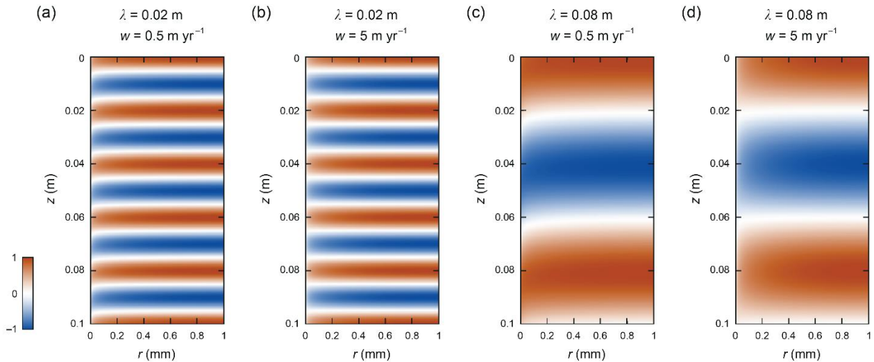
Figure 5. Patterns of \delta computed for T = -52 \text{ }^\circ\text{C} at (a) \lambda = 0.02 \text{ m} , w = 0.5 \text{ m yr}^{-1} , (b) \lambda = 0.02 \text{ m} , w = 5 \text{ m yr}^{-1} , (c) \lambda = 0.08 \text{ m} , w = 0.5 \text{ m yr}^{-1} , and (d) \lambda = 0.08 \text{ m} , w = 5 \text{ m yr}^{-1} . The enhancement factors are f = 3.68, 4.27, 14.7 and 51.9 , respectively.
