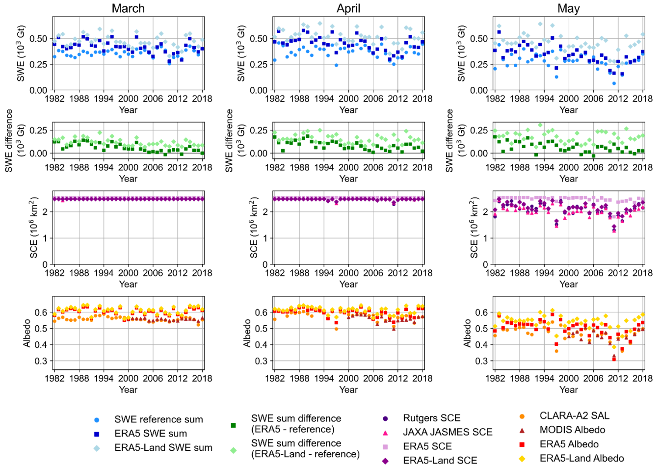
Figure 11. Timeseries in Western Siberia in (left) March, (middle) April, and (right) May for SWE sum (top row), the difference in SWE sum (second row), SCE (third row), and albedo (bottom row). The area is marked in Figs. 8 and 9.
