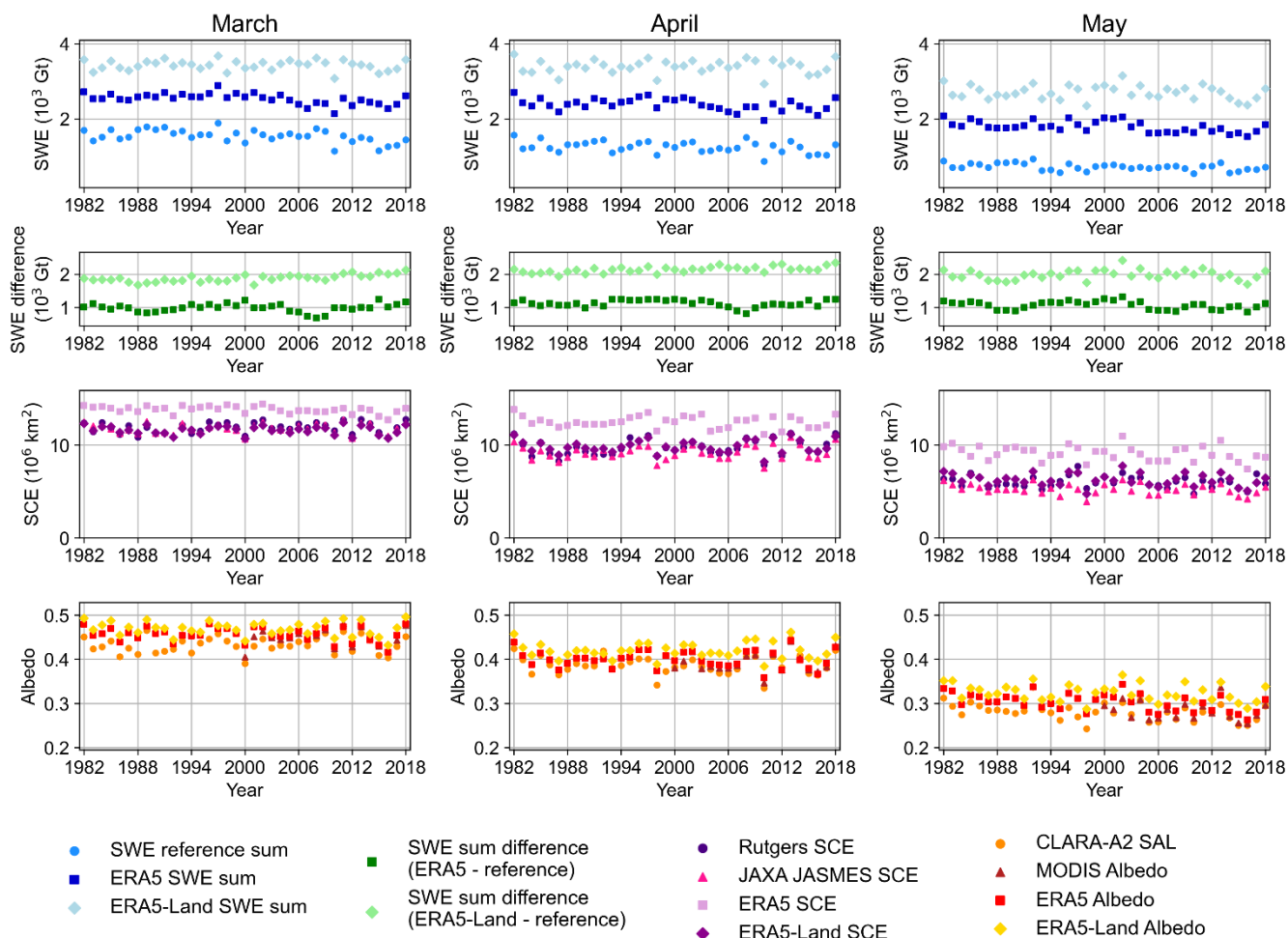
365 Figure 5. Timeseries in North America in (left) March, (middle) April, and (right) May for SWE sum (top row), the difference in SWE sum (second row), SCE (third row), and albedo (bottom row).
