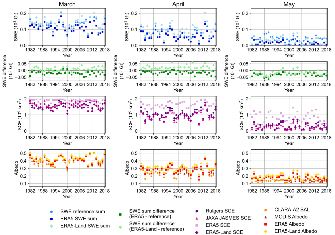
Figure 12. Timeseries in Canadian Prairies in (left) March, (middle) April, and (right) May for SWE sum (top row), the difference in SWE sum (second row), SCE (third row), and albedo (bottom row). The area is marked in Figs. 8 and 9.
