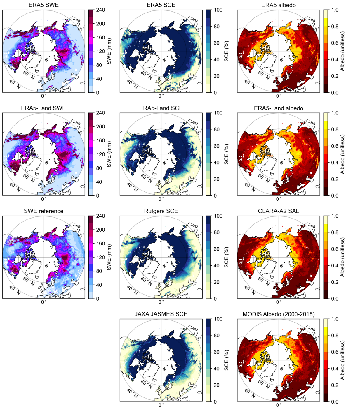
290 Figure 1. Mean values in April 1982-2018 for each of the datasets (MODIS 2000-2018).
