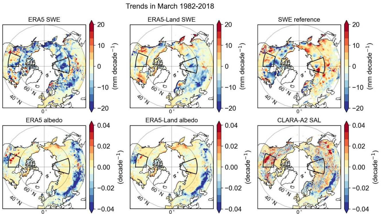
Figure 9. (top row) SWE trends in March 1982-2018. (bottom row) Albedo trends in March 1982-2018.
