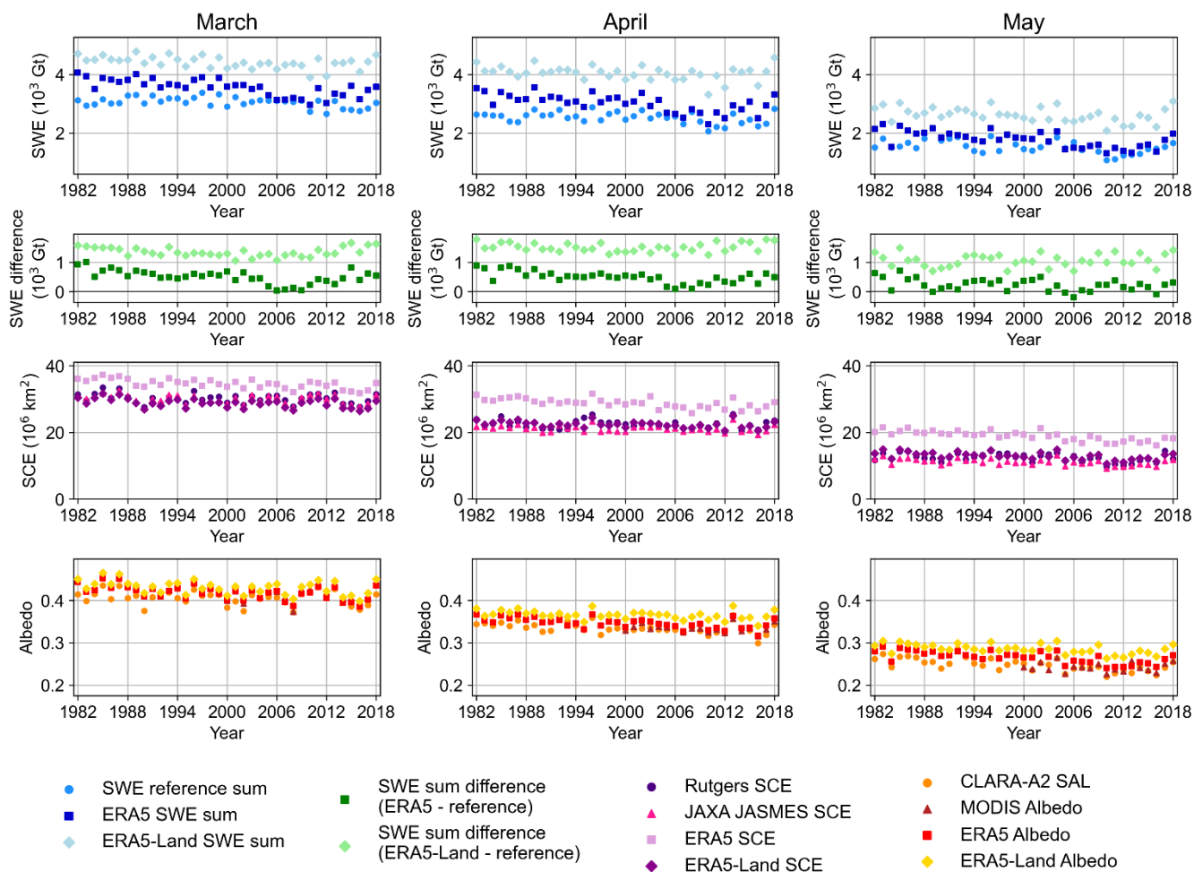
305 Figure 3. Timeseries in the non-mountainous regions in (left) March, (middle) April, and (right) May for SWE sum (top row), difference in SWE sum (second row), SCE (third row), and albedo (bottom row).
