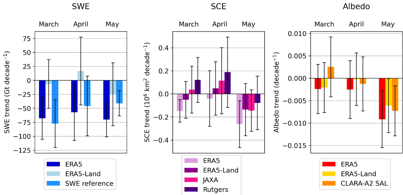
Figure 6. Trends in North America in 1982-2018. The error bars represent the 95% confidence intervals.
