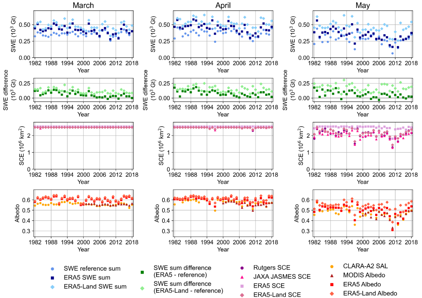
Figure 10. Timeseries in Western Siberia in (left) March, (middle) April, and (right) May for SWE sum (top row), the difference in SWE sum (second row), SCE (third row), and albedo (bottom row). The area is marked in Figs. 8 and 9.
