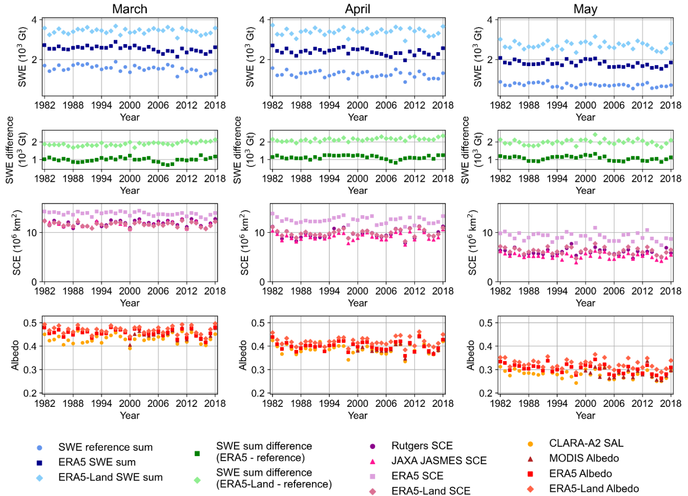
Figure 4. Timeseries in North America in (left) March, (middle) April, and (right) May for SWE sum (top row), the difference in SWE sum (second row), SCE (third row), and albedo (bottom row).
