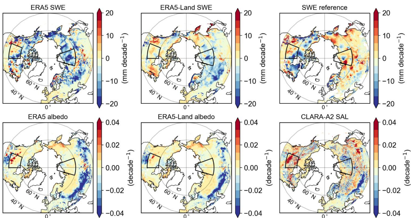
430 Figure 8. (top row) SWE trends in March 1982-2018. (bottom row) Albedo trends in March 1982-2018.
