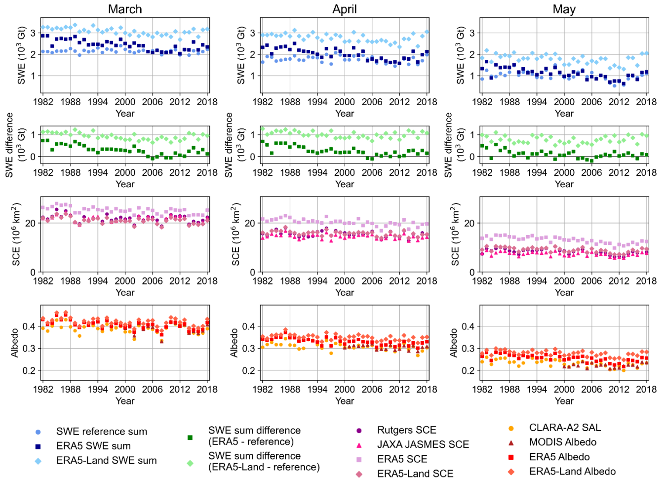
Figure 5. Timeseries in Eurasia in (left) March, (middle) April, and (right) May for SWE sum (top row), the difference in SWE sum (second row), SCE (third row), and albedo (bottom row).
