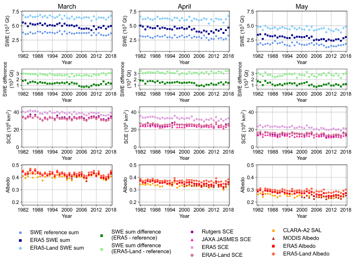
295 Figure 2. Timeseries in the whole study area in (left) March, (middle) April, and (right) May for SWE sum (top row), difference in SWE sum (second row), SCE (third row), and albedo (bottom row).
