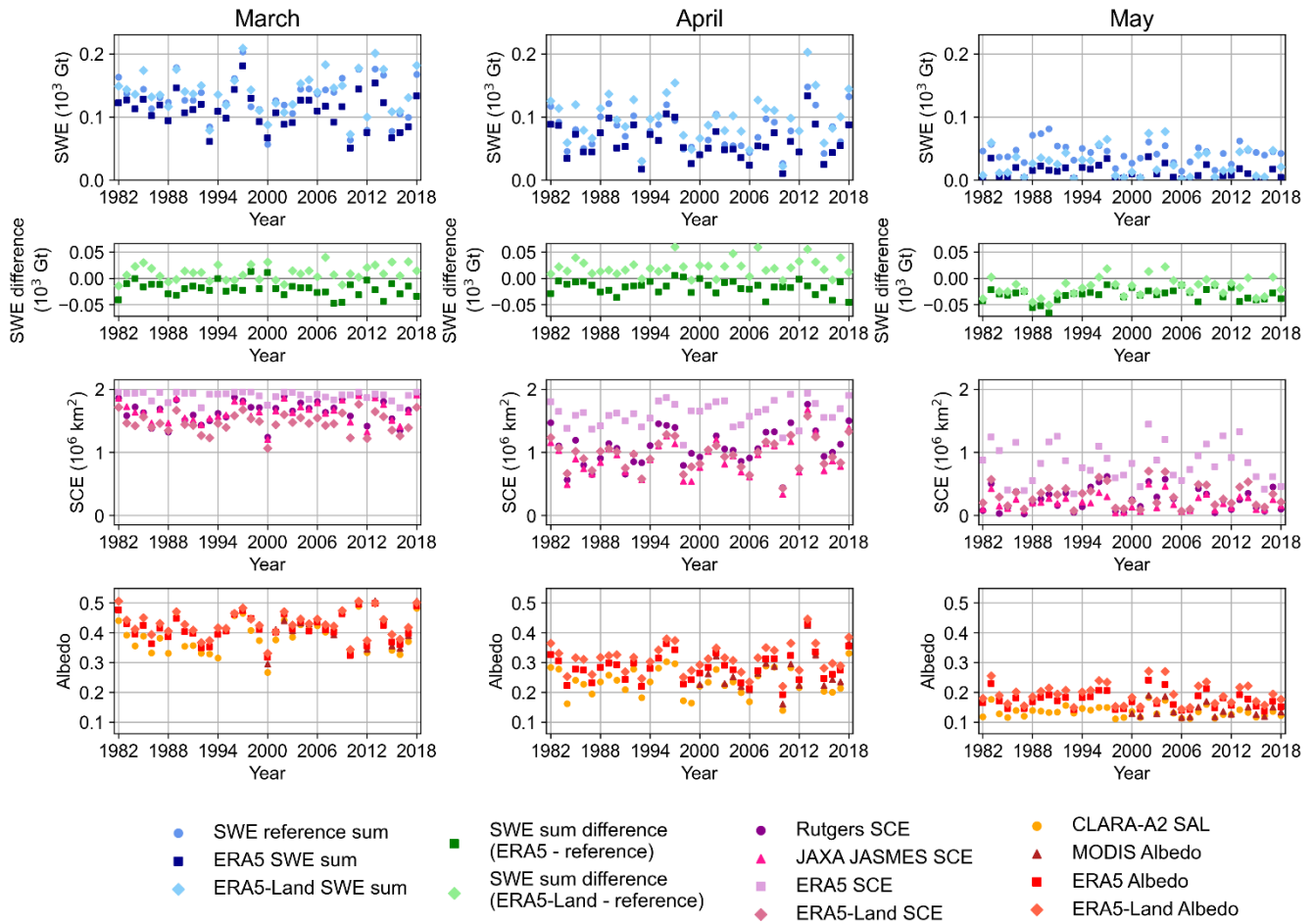
Figure 11. Timeseries in Canadian Prairies in (left) March, (middle) April, and (right) May for SWE sum (top row), the difference in SWE sum (second row), SCE (third row), and albedo (bottom row). The area is marked in Figs. 8 and 9.
