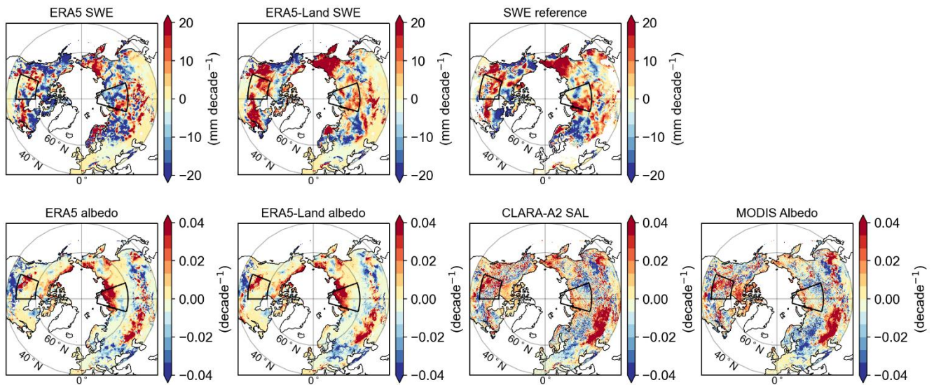
Figure 9. (top row) SWE trends in March 2000-2018. (bottom row) Albedo trends in March 2000-2018.
