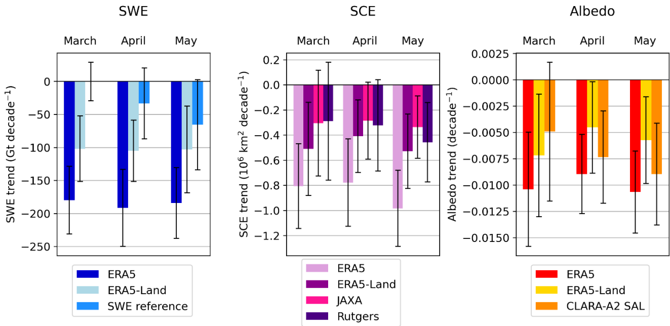
Figure 7. Trends in Eurasia in 1982-2018. The error bars represent the 95% confidence intervals.
