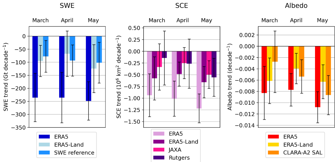
Figure 3. Trends in the Northern Hemisphere in 1982-2018. The error bars represent the 95% confidence intervals.
