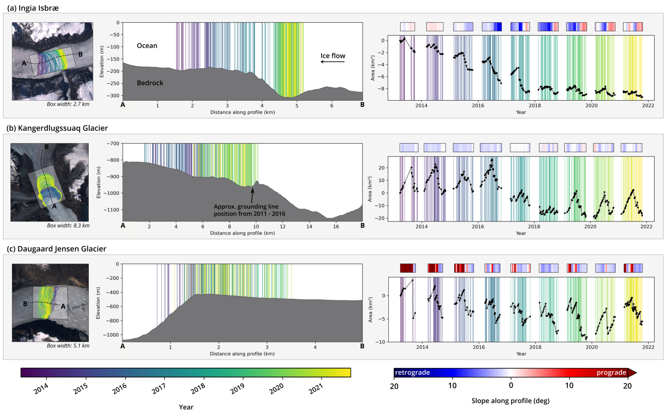
Figure 10. Effect of bedrock topography of calving front variation for (a) Ingia Isbræ, (b) Kangerdlugssuaq Glacier and (c) Daugaard Jensen Glacier. Shown are (from left to right) a satellite image with calving front trajectories as well as a marked profile, bedrock topography and color-coded calving front positions along this profile and the corresponding time series of calving front variation. Note that the axes are scaled differently for each glacier. Landsat-8 imagery courtesy of the U.S. Geological Survey.
