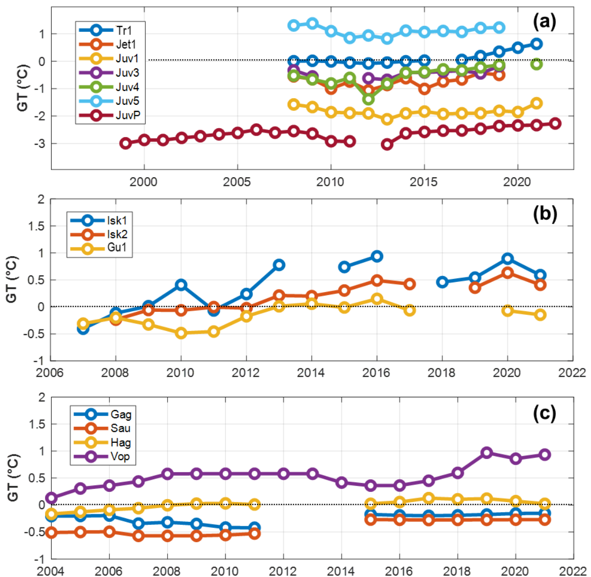
Figures 3: Ground temperature (GT) development in time at 10 m depth at selected sites calculated over a hydrological year in (a) Southern Norway, (b) Northern Norway and (c) Iceland. At Vopnafjörður in Iceland, GT = 20 m.
