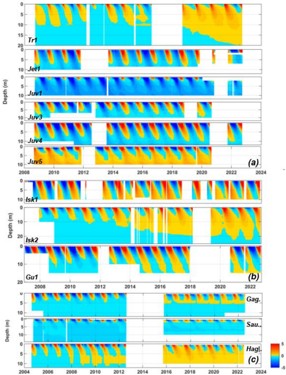
580 Figure B2: Time-depth temperature plots for all measurement sites. (a): Sites in southern Norway, (b) Northern Norway and (c) Iceland.
