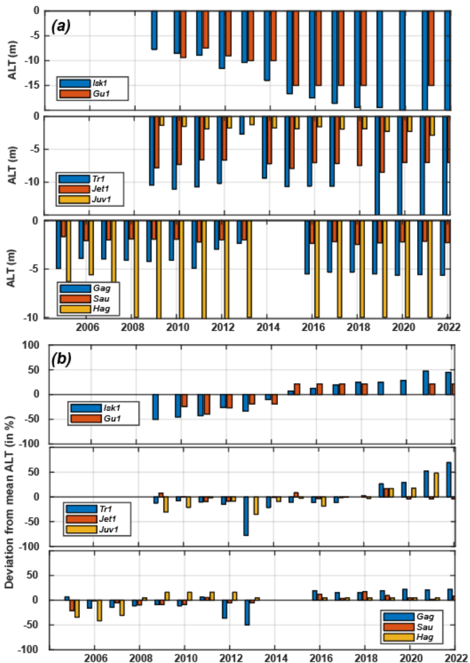
570 Figure B1: (a) Active layer thickness development at selected boreholes at the permafrost observatories. ALT exactly at -15 m or -10 m denotes thaw in the entire borehole length and normally talik development (Figure 5). (b): Normalised active layer thickness change in relation of overall average during the measurement period in percent. In northern Norway a steady
