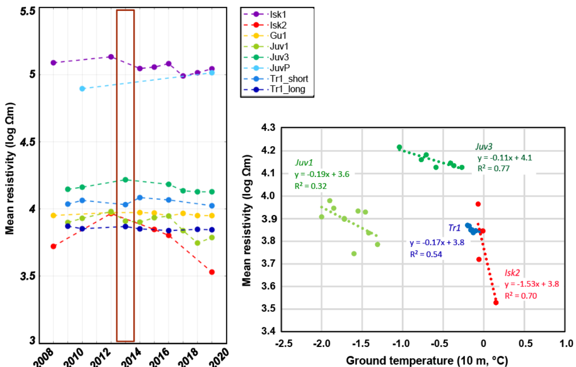
365 Figure 6 (a) Development of specific resistivity at borehole locations at the sites where multi-temporal ERT surveys were measured. The values are calculated as a spatial mean over an area (the so-called zone-of-interest, ZOI), mostly 10-20 m wide and a couple of meters deep. This ZOI is considered as a representative permafrost zone below the active layer, at least during the first part of the measurement period. The box indicates the cold period around 2013. (b): Average specific resistivity as in (a), plotted against the average ground temperature at the date of the ERT
