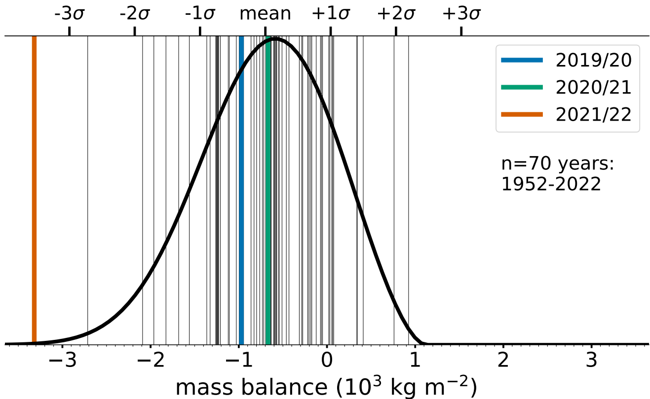
Figure 1. The annual mass balance observations of Hintereisferner (in 10^3 \text{ kg m}^{-2} ) over the full 70 years record are depicted as vertical lines. A fitted normal-generalized extreme value distribution of these observations is added to emphasize the extremity of the year 2021/22. The hydrological years used in this study are given in blue (2019/20), green (2020/2021) and red (2021/2022). The idea of this figure was inspired by a Twitter post from Matthias Huss ( https://twitter.com/matthias_huss/status/1575539821493293058 ).
