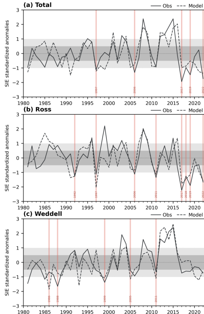
Figure 1: Standardized SIE anomalies in JFM computed over (a) the total SO domain (b) the Ross region (c) the Weddell region. Comparison 170 between observations (solid line) and model (dashed line). Dark and light grey shadings indicate the \pm 0.5 and \pm 1\sigma , respectively. Years with a minimum SIE are marked in red.
