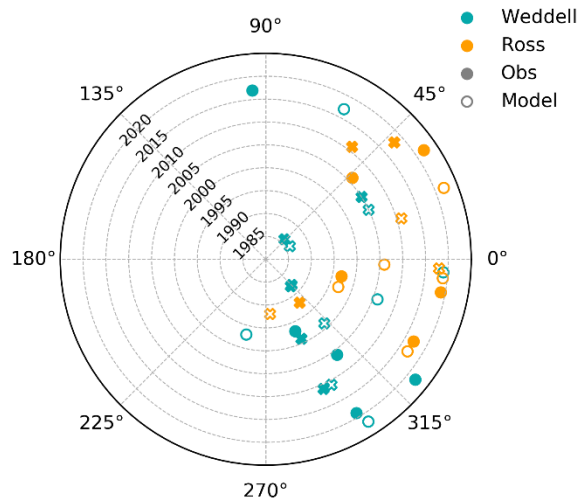
Figure 6: Average OND 10-m wind direction for all extreme years in the observations (full points) and model (empty points). Circles indicate total minima, while crosses are for regional ones. The values indicate the angle of the wind vectors with respect to the zonal axis: 0° = pure westerly winds, 90° = pure southerly, 180° = pure easterly, 270° = pure northerly. See main text for details.
