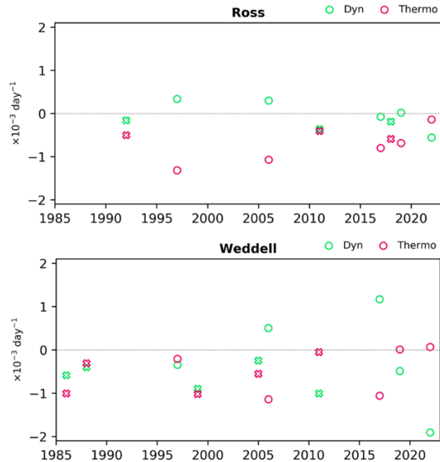
Figure 7: Average anomalous dynamic (green) and thermodynamic (magenta) contributions to the sea ice budget in NDJ for the (a) Ross and (b) Weddell regions. Circles indicate total minima, while crosses are for regional ones. See main text for details.
