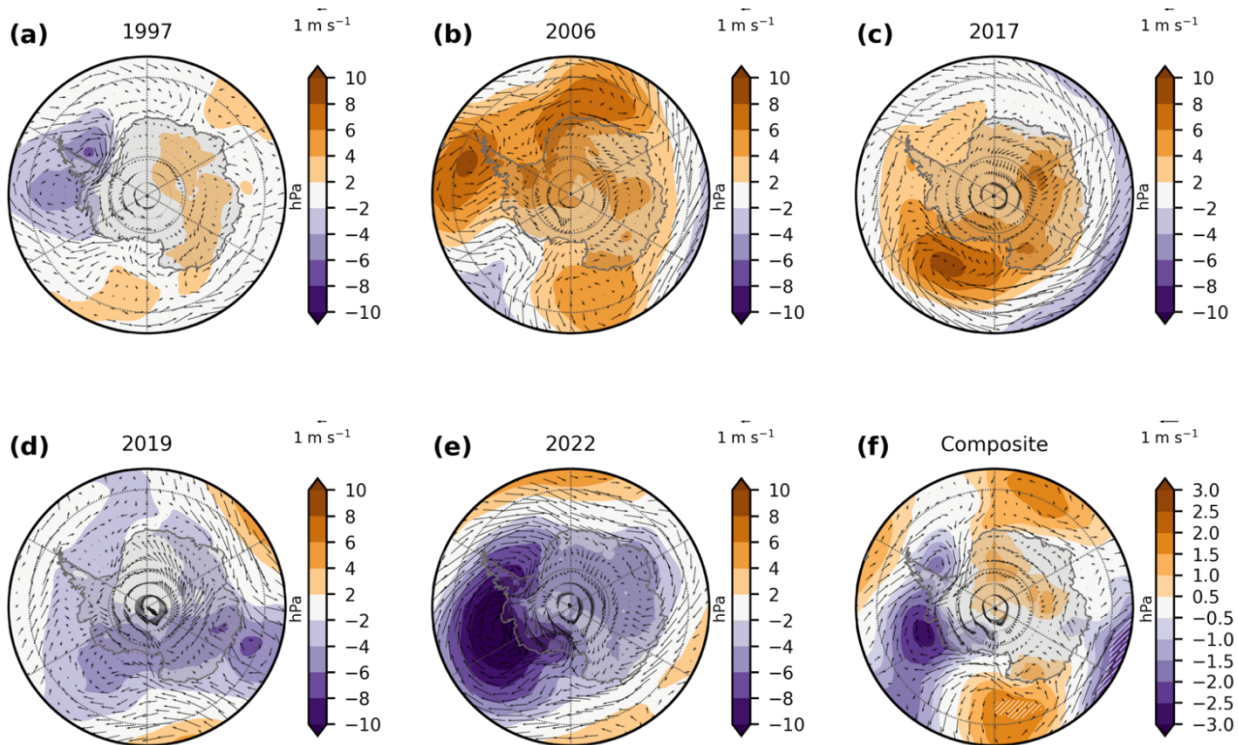
320 Figure 5: SLP (shading) and 10-m wind (arrows) anomalies in the years with total SIE minima (panels a-e) and their composite (panel f) during the previous spring (OND). Hatching in the composite map indicates statistically significant SLP values.
