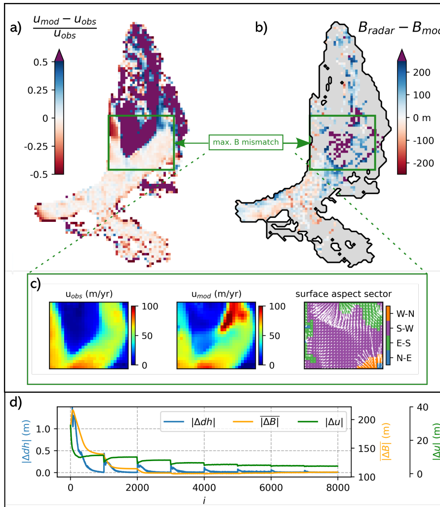
Figure 6. Raw output of Kronebreen inversion. a) Velocity misfit with purple color indicating where modelled velocities exceed observed velocities by more than 50%. b) Difference between radar-derived and modelled bed elevation. c) Zoom into area with largest bed deviations for observed velocities, modelled velocities and surface aspect (with arrows denoting downhill direction, and colors showing into which sector the ice surface is sloping). d) dh/dt (eq. (5)), bed (eq. (7)) and velocity misfit (eq. (6)) per iteration.
