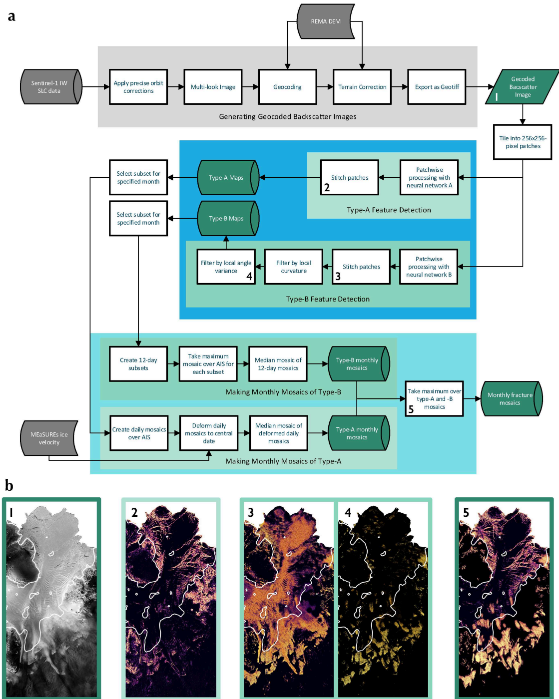
Figure 2. Outline of the processing chain that takes a month of Sentinel-1 IW SLC data and produces a fracture mosaic. (a) shows a flow diagram representing the process. (b1-5) show different stages of processing for an example SAR image over the Crosson Ice Shelf. In each panel b2-5, features that appear brighter are more likely to be crevasses according to the latest processing step. Numbers in the top-left corner correspond to the stages of processing that match the numbers in the flow diagram (a). (b1) A 50 m resolution SAR backscatter image from 01/06/2021. (b2) The image after processing with the neural network N_A ; showing type-A features. (b3) The image after processing with the neural network N_B . This displays type-B features along with a considerable noise on the floating ice. (b4) The result of applying the type-B filtering algorithm to (b3). Most of the noise is seen to be removed, leaving type-B features visible from that particular look angle. (b5) A mosaic for the month of June 2021, from images like those displayed in (b2) and (b4). The superimposed white lines show the MEaSURES grounding line (Rignot et al., 2016).
