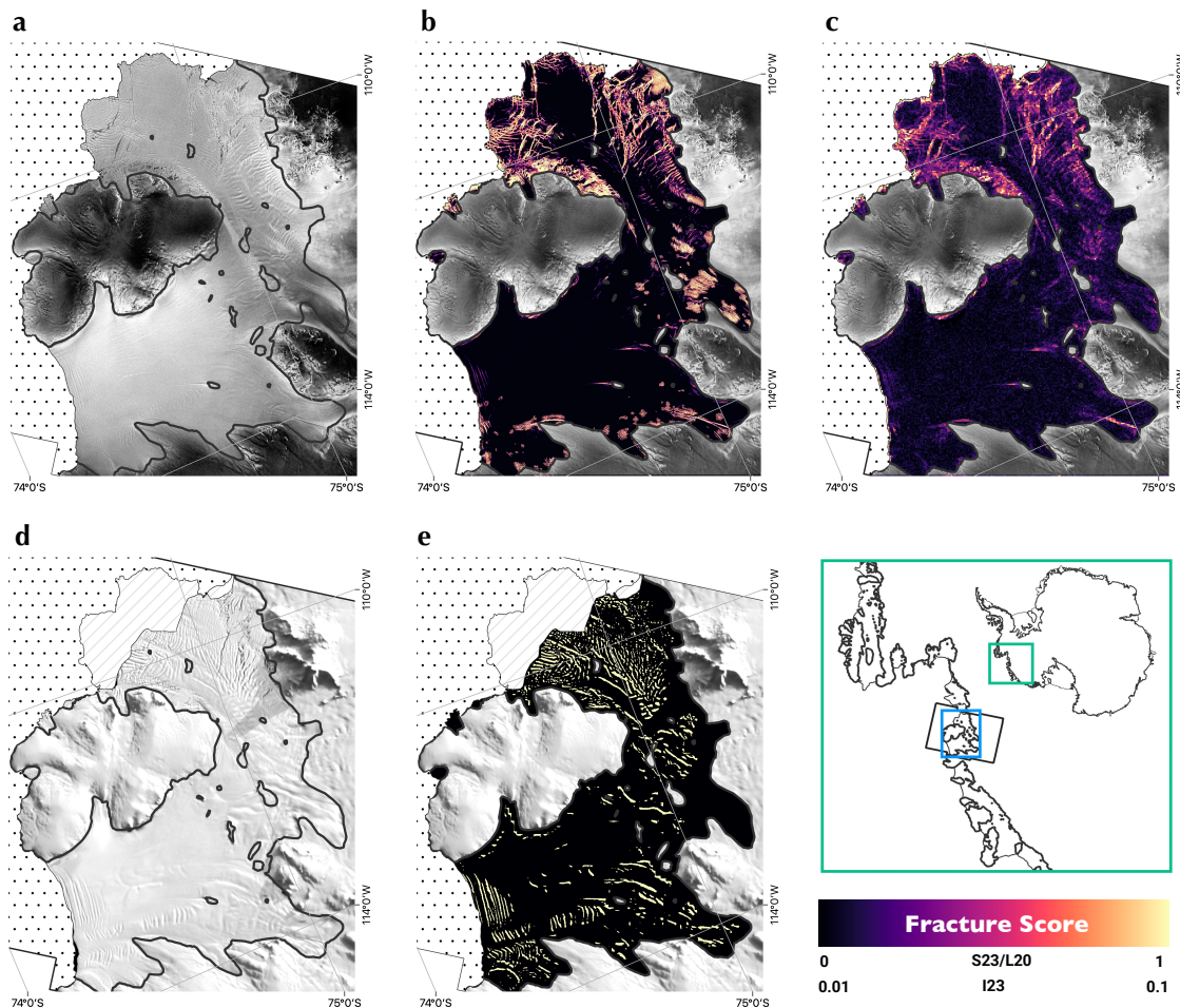
Figure 10. A comparison of fracture maps generated using our method (“S23”) versus two existing methods (Lai et al. (2020), Lai et al. (2020) “L20” and Izeboud and Lhermitte (2023) Izeboud and Lhermitte (2023) “I23”), over the Crosson and Dotson Ice Shelves. (a) Sentinel-1 backscatter image at 50 m resolution, ESA TFPF: 7/913, dated 20210607, used for the S23 and I23 crevasse maps. (b) June 2021 crevasse mosaic using S23 restricted to the floating ice. (c) Result of application of I23 to the SAR backscatter image shown in (a); with the colourmap showing the range 0.01 to 0.1. Grounded ice in (b-c) is masked by the SAR backscatter image shown in (a). (d) MODIS Mosaic of Antarctica (Haran et al., 2021) (Haran et al., 2014) restricted to the geometry of the SAR backscatter image shown in (a). (e) Crevasse map from L20, with the grounded ice masked by the MODIS MOA shown in (d). The area outside of the bounds of the SAR backscatter image shown in (a) are masked in (a-e). Grounding lines are as given by Rignot et al. (2016), and is shown as with a black line. The difference between the June 2021 Crosson Ice Shelf extent and the edge of the L20 dataset is shown in (d-e) as the striped region. The sea is shown as the spotted region. The blue box on the map in the bottom right shows the extent of the region shown in (a-e). This lies on a black outline showing the bounds of the SAR backscatter image shown in (a). Inset is a map of Antarctica showing the location of the blown-up region. For S23 and L20, the colourmap displays the range 0-1, while for I23, it displays the range 0.01-0.1.
