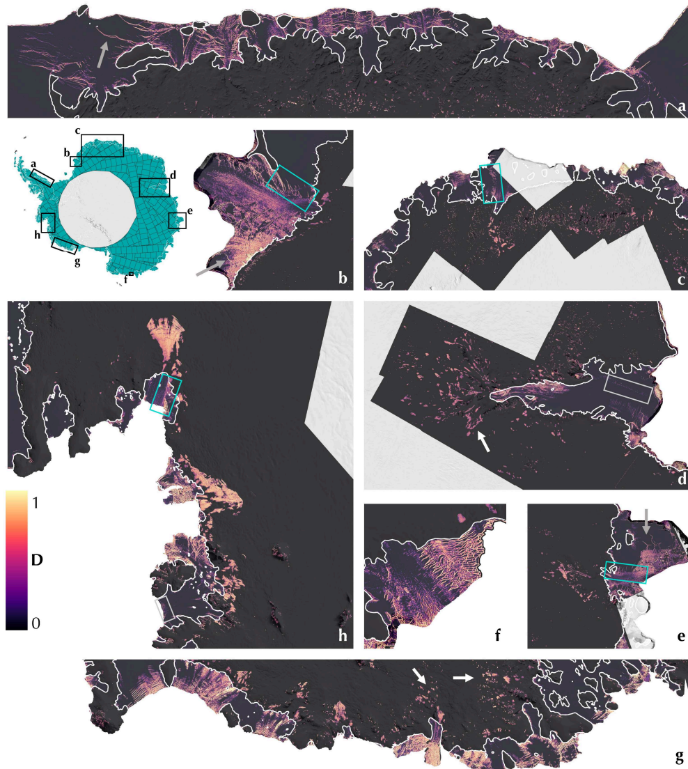
Figure 4. Fractures in Antarctica: April 2022. Results at different scales from a pan-continental fracture mosaic. D \in (0,1) D \in [0,1] is a normalised score with 1 indicating ‘fracture’ and 0 indicating ‘no-fracture’ for each pixel. The labelling of subfigures corresponds to a clockwise ordering around the Antarctic coastline starting from the Eastern Antarctic Peninsula. (a) The Larsen-D Ice Shelf. (b) The Brunt-Stancomb-Wills Ice Shelf. (c) Dronning-Maud Land including Fimbul Glacier and Ice Shelf. (d) The Améry-Amery Ice Shelf and its basin - including Lambert Glacier. (e) Shackleton Ice Shelf and Denman Glacier. (f) Cook Ice Shelf. (g) The coastline between West Getz (left) and Salzburger (right) Ice Shelves, with the Land Ice Tongue in the centre. (h) The Amundsen Sea Embayment, including, from top to bottom, Pine Island Glacier, Thwaites Glacier, Crosson Ice Shelf and its tributary glaciers, and Dotson Ice Shelf. The top-left inset shows the Antarctic Ice Sheet with locations of the images (a-h) identified with black boxes. These give a sense of the different scales at which crevasses can be seen. In teal, we show the total extent of all Sentinel-1 acquisitions over the AIS so far. The white line shows the MEaSUREs grounding line (Rignot et al., 2016).
