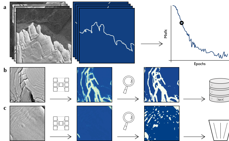
Figure 3. Bootstrapping partially trained neural network N_A . (a) Example input/target pairs for the initial phase of training of the randomly initialised network. Training is was stopped well before parameter convergence. (b-c) (b-c) (e) Bootstrapping. The network is was applied to unseen images and the outputs are were visually inspected. If the outputs can could be thresholded to look like a plausible target image (b), that threshold is was applied before the input/output pair is was added to a new training dataset. If not, (c) that input/output pair is was discarded.
