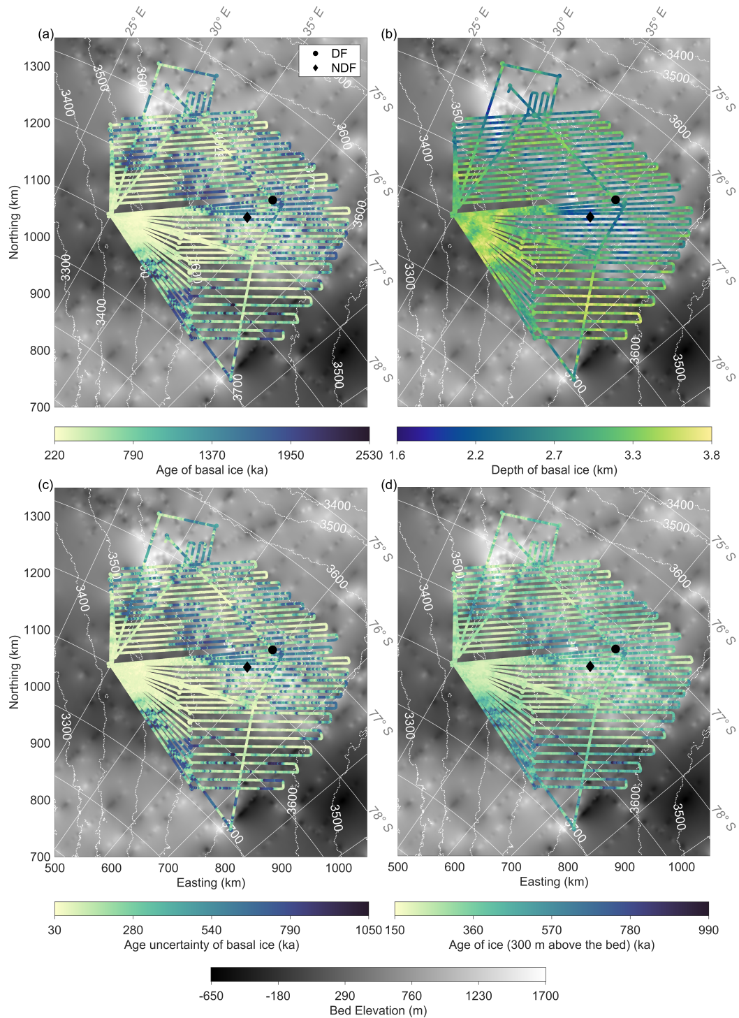
Figure 4. (a) Modeled age of basal ice at a maximum age density of 20 \text{ ka m}^{-1} . (b) Depth of the basal ice at a maximum age density of 20 \text{ ka m}^{-1} . (c) Modeled age uncertainty of the basal ice. (d) Modeled age of the ice at a height of 300 m above the bed.
