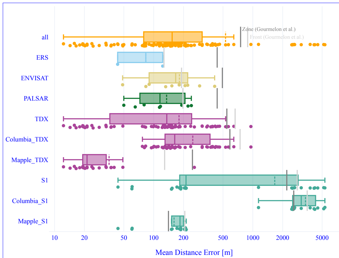
Figure 12. MDE on the test set grouped by satellites. The dark grey line shows the baseline of the zone prediction, and the light grey line shows the baseline of the front prediction from (Gourmelon et al., 2022). The images from ERS (light blue), ENVISAT (yellow), and PALSAR (green) only capture the Mapple Glacier. The MDE from TDX (pink) and S1 (turquoise) is subdivided into the two glaciers of the test set. The ensemble model was trained with the fusion of zone and front labels. The y-axis has a logarithmic scale. The median is the middle line in the rectangle, and the dashed line represents the mean. The x-axis has a logarithmic scale. Otherwise, the outliers would dominate the plot. The rectangle reaches from the first quartile to the third quartile.
