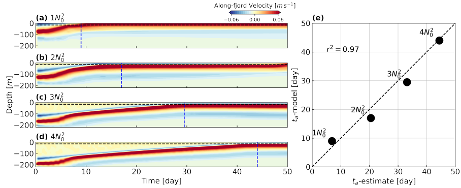
Figure 9. Ascending time ( t_a ) of the plume with increasing initial stratification. (a)-(d): Evolution of the vertical structure of along-fjord velocity near the glacier front, with positive values toward the fjord mouth. Horizontal dashed black lines show the maximum sill height ( h_s/h_f = 0.04 ), and vertical dashed blue lines indicate the estimated time for the plume rising from its initial height to the level of the sill crest. (e): A comparison between the plume ascending time estimated from theory and the model output.
