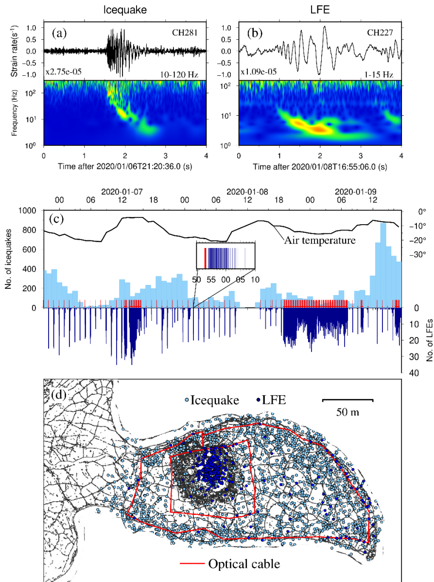
450 Figure 2: Typical passive signal waveforms, temporal and spatial distributions. (a) Icequake wave recorded by channel 281. The waveform is bandpass filtered in the frequency band of 10-120 Hz. (b) LFE waveform by channel 227. The waveform is bandpass filtered in the frequency band of 1-15 Hz. (c) temporal distributions for icequakes (light blue) per hour and LFEs (dark blue) per minute and the local air temperature (black curve). The temperature data is from European Centre for Medium-Range Weather Forecasts ( https://www.ecmwf.int/ ). The time of AGE is marked with red arrow. The inset picture shows a window of 20 minutes with an AGE (red line) and following LFEs (black lines). The air temperature is denoted with black curve. (d) spatial distribution for icequakes (light blue) and LFEs (dark blue).
