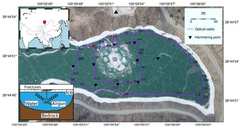
460 Figure 1: The experimental setting. The instrumented frozen lake is at Xiliushui Reservoir in Gansu Province, China (red rectangle in the inset). The optical fibre is marked with purple lines with channel number between 51-645 with gauge length of 10 m and a sampling rate of 1000 Hz. The airgun floating platform is at the centre of the lake. A reference broadband seismic station is marked with a triangle. Hammering points are marked with inverted triangles. The red triangle shows the one we use to measure the dispersion curve of flexural-gravity wave.
