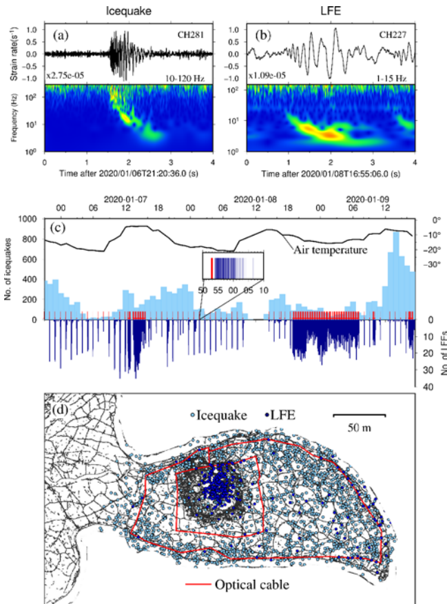
Figure 2: Typical passive signal waveforms, temporal and spatial distributions. (a) Icequake wave recorded by channel 281. The waveform is bandpass filtered in the frequency band of 10-120 Hz. (b) LFE waveform by channel 227. The waveform is bandpass filtered in the frequency band of 1-15 Hz. (c) temporal distributions for icequakes (light blue) per hour and LFEs (dark blue) per minute and the local air temperature (black curve). The temperature data is from European Centre for Medium-Range Weather Forecasts ( https://www.ecmwf.int/ ). The time of AGE is marked with red arrow. The inset picture shows a window of 20 minutes with an AGE (red line) and following LFEs (black lines). The air temperature is denoted with black curve. (d) spatial distribution for icequakes (light blue) and LFEs (dark blue).
