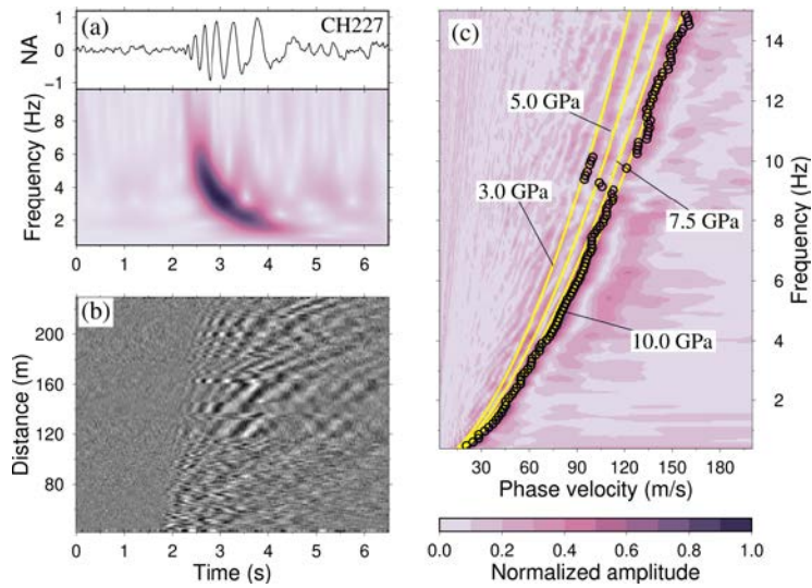
475 Figure 3: Dispersion analysis of LFEs. (a) Stacked LFE waveform and spectrogram of channel 227. The black curve is the stacked waveform with 272 LFE traces. It is bandpass filtered in the frequency band 1-15 Hz. The color denotes the normalized amplitude. (b) The record section of stacked waveform of all LFE events assuming all LFEs are originated at the AGE platform. (c) The measured phase velocity (circles) and predicted velocities (yellow curves) with different Young's modulus (3-10 GPa). The color means the dispersion spectra of stacked LFE traces in (c).
