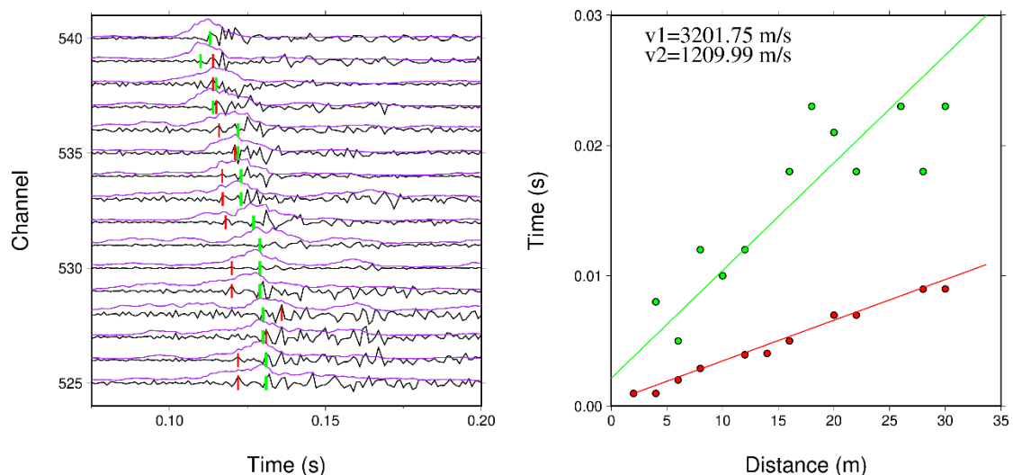
Fig. S3 Velocity measurement with hammering signal. Left: Waveform of hammering event (black curves), STA/LTA waveform (purple). The
