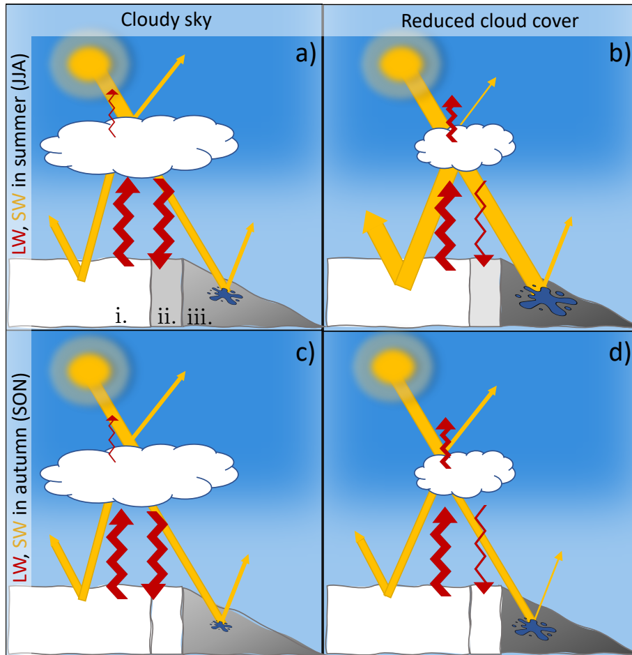
Figure 8. Schematic radiative energy flows over the GrIS in CMIP5 and CMIP6 Schematic radiative energy flows over the GrIS in CMIP5 'Cloudy sky' and CMIP6 'Reduced cloud cover' . Simplified schematic representation of the radiative energy flows over the Greenland ice sheet for cloudy sky condition (left panel) and reduced cloud condition (right panel), for summer (JJA) SW radiation (a-b) , summer (JJA) LW radiation (c-d) , and autumn (SON) SW and LW radiation (e-f, c-d) . All fluxes are positive downwards. The ice sheet is divided into three different zones i) the accumulation zone, ii) the percolation zone, iii) the ablation zone.
