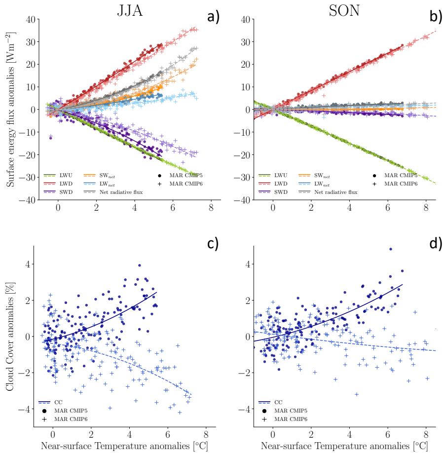
Figure 2. Radiative SEB component anomalies [ \text{Wm}^{-2} ] and total cloud cover anomalies [%] as a function of the near-surface air temperature anomalies [°C]. a) Seasonal (JJA) radiative SEB component anomalies [ \text{Wm}^{-2} ] over the GrIS according to near-surface air temperature anomalies [°C] from MAR CMIP5 (dots) and MAR CMIP6 (crosses), with regression drawn in solid lines for MAR CMIP5 and dashed lines for MAR CMIP6. It includes the radiative energy fluxes of longwave down (LWD), longwave up (LWU), shortwave down (SWD), net longwave radiation ( \text{LW}_{net} ), net shortwave radiation ( \text{SW}_{net} ), and Net radiative flux. Positive direction towards the surface. b) same as a), but for autumn (SON). c) same as a), but for the variable of cloud cover [%]. d) same as c), but for autumn (SON).
