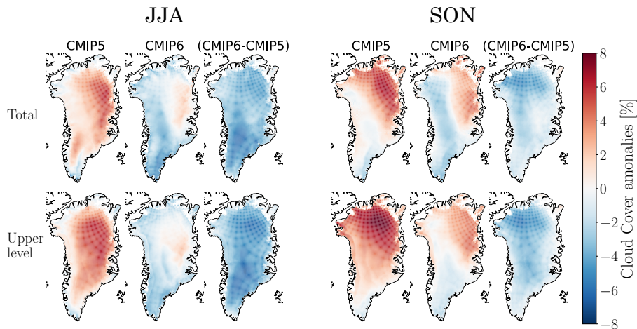
Figure 4. Cloud cover anomalies [%] for MAR CMIP5 and MAR CMIP6 simulations ( + 4^{\circ}\text{C} \pm 10 years) for summer (JJA) and autumn (SON). Twenty-year average ( 4^{\circ}\text{C} \pm 10 years) of the cloud cover [%] over the GrIS for summer (JJA, left) and autumn (SON, right). The two rows indicate the total (upper row) and upper level cloud cover ( < 44000\text{-Pa} 440 hPa , bottom row). Each season has three columns — the first indicates the cloud cover anomalies for MAR CMIP5, the second for MAR CMIP6, and the third the difference between the two (CMIP6-CMIP5). For MAR CMIP5 and MAR CMIP6 a positive value (red) indicates an increase in cloud cover, and a negative value (blue) a reduction in cloud cover compared to the reference period. For the difference (CMIP6-CMIP5) a positive value (red) indicates more positive cloud cover anomaly, and negative values (blue) indicate a more negative cloud cover anomaly in MAR CMIP6 compared to MAR CMIP5.
