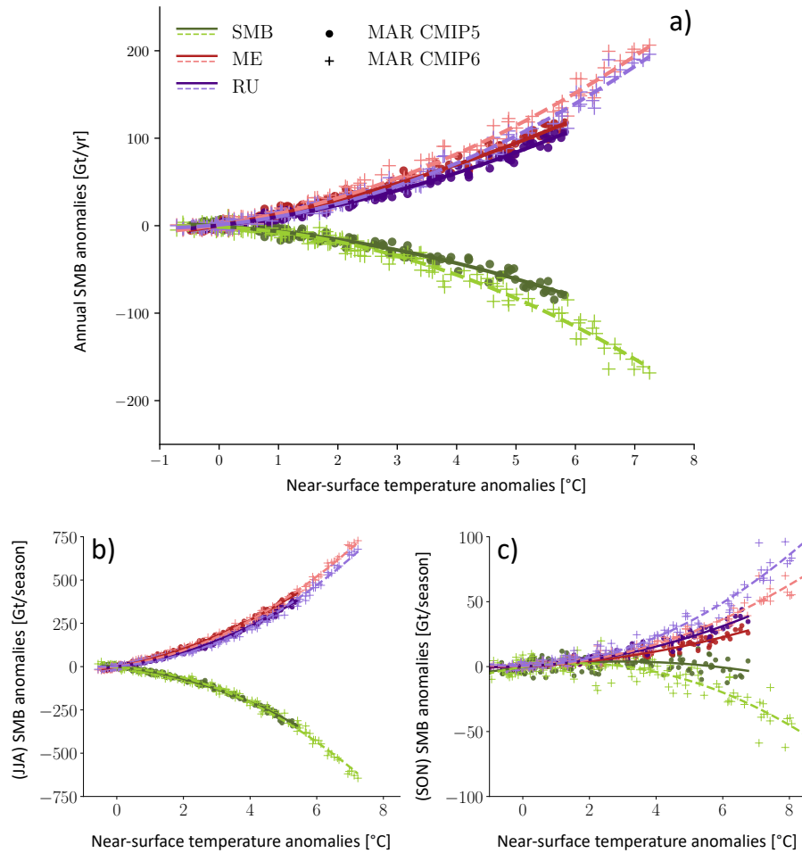
Figure 1. SMB, melt and runoff anomalies over the GrIS as a function of Greenland near-surface temperature anomalies °C. SMB, melt and runoff anomalies [Gt/yr] over the GrIS as a function of Greenland near-surface temperature anomalies [°C]. a) Annual SMB, melt- (ME), and runoff anomalies (RU) [mmWE Gt/yr] over the GrIS as a function of annual near-surface temperature anomalies [°C] over Greenland from MAR CMIP5 (dots) and MAR CMIP6 (crosses), with regression drawn in solid lines for MAR CMIP5 and scattered lines for MAR CMIP6. All anomalies are related to the thirty-years averaged reference period (1961–1990). b) and c) same as a) , but for a seasonal mean of summer (JJA) and autumn (SON), respectively.
