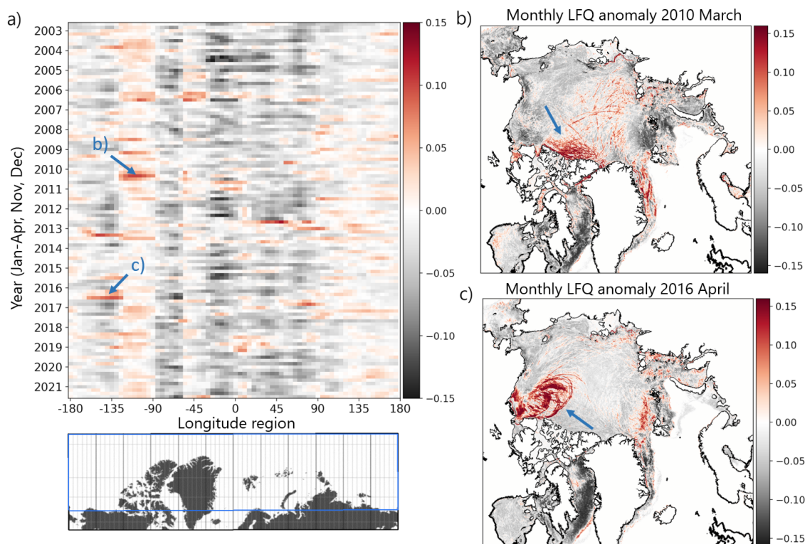
Figure 3. a) Latitude-averaged ( 70 - 90^\circ N) monthly LFQ anomalies in 5^\circ longitude bins for Nov 2002 to April 2021. Only the months Nov, Dec, Jan, Feb, Mar and Apr are shown, b) monthly lead frequency (LFQ) anomaly for 2010, Mar, with a very strong positive lead anomaly north of the Canadian Archipelago and c) monthly LFQ anomaly for 2016, April, underpinning the strong positive lead anomaly in the Beaufort Sea that is also given in the overview in a). Anomalies are calculated relative to the climatological monthly means.
