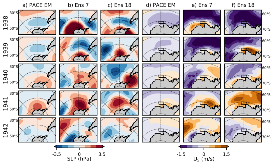
Figure 5. (a-c) Modeled SLP and (d-f) U_s anomalies from 1938 to 1942 in the tropical Pacific pacemaker ensemble of simulations. The ensemble mean, ensemble 7, and ensemble 18 of the Pacific pacemaker ensemble is shown. Anomaly reference period is 1961 to 1990.
