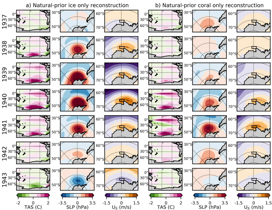
300 Figure 4. Same as in Figure 3, but with the natural-prior and only ice cores assimilated (a) and only corals assimilated (b). The same figure using the anthro-prior is shown in Figure A2.
