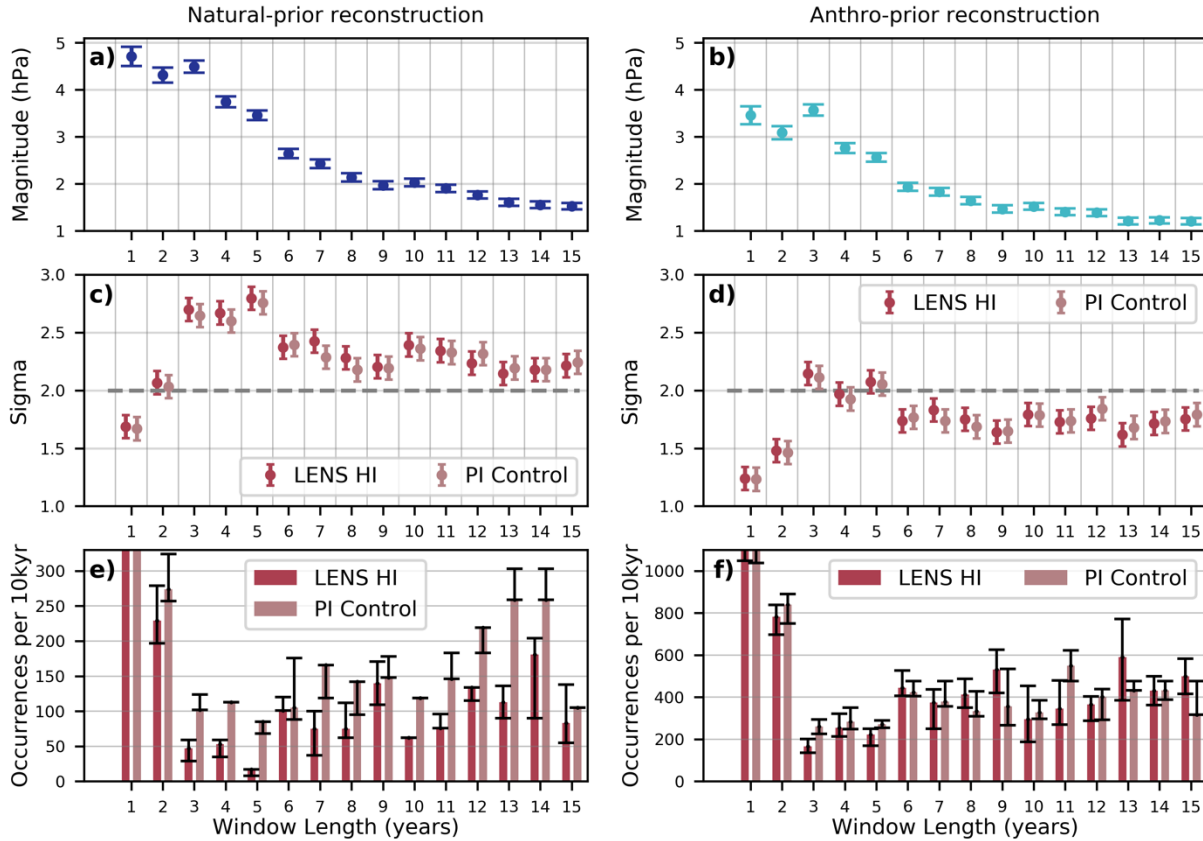
Figure 7. Magnitudes of the 1940s SLP event based on 1-to-15-year averaging windows centered around 1940/41, calculated using (a) the natural-prior reconstruction and the (b) anthro-prior reconstruction (in anomalies relative to 1961 to 1990). The circles represent the mean magnitudes and the error bars represent the 95% confidence intervals. (c, d) Sigma levels of each reconstructed magnitude in panels (a) and (b) relative to two climate model simulations: the Preindustrial Control simulation (PI Control) and the internal component of the LENS Historical simulation (LENS HI). The dashed line highlights the 2-sigma level. (e, f) Histograms of the frequency of the 1940s event based on each averaging window, reported as occurrences per 10kyr (using the magnitudes in (a) and (b)) found in the two climate simulations. The error bars represent occurrences based on the upper and lower bounds of the confidence intervals in (a). The y-axes are selected to highlight the rarest events and differ between (e) and (f); the values for all events can be found in Table 1.
