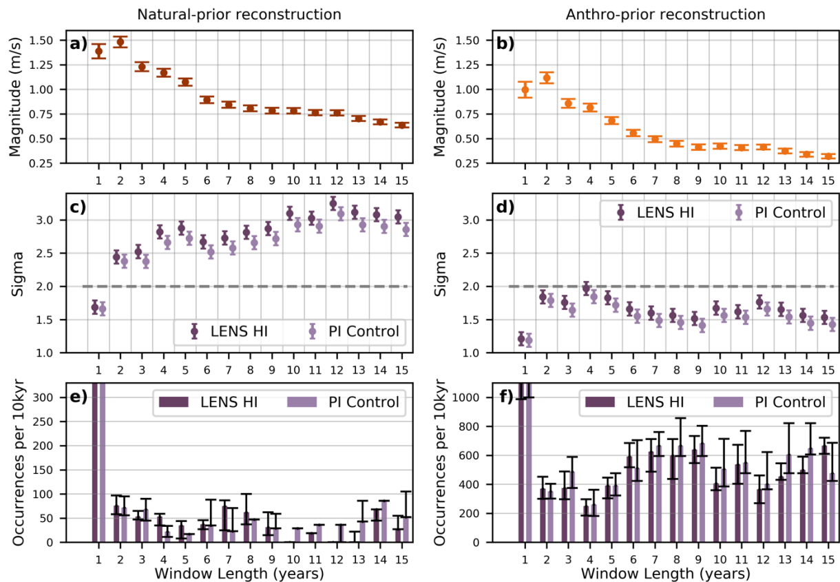
495 Figure 8. Same as in Figure 7, but for reconstructions of U_s (geostrophic winds are used for the anthro-prior reconstruction). The values for all events can be found in Table 1.
