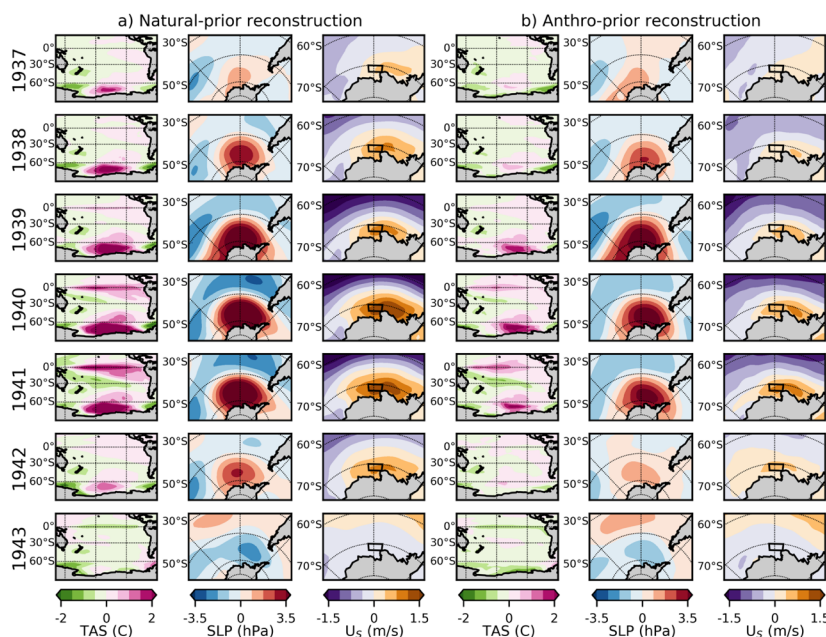
270 Figure 3. (a) Reconstructed anomalies in surface air temperature (TAS), SLP, and U_s in the natural-prior reconstruction (with all proxies assimilated) from the years 1937 to 1943 (the reconstruction ensemble means are shown). (b) Same as in (a) but with the anthro-prior reconstruction. Anomaly reference period is 1961-1990. The black box on the wind panel shows the Amundsen Sea Embayment continental shelf break region.
