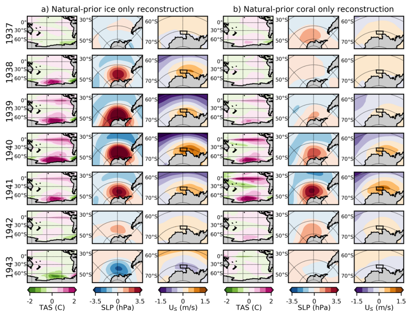
330 Figure 4. Same as in Figure 3, but with the natural-prior and only ice cores assimilated (a) and only corals assimilated (b). The same figure using the anthro-prior is shown in Figure A2.
