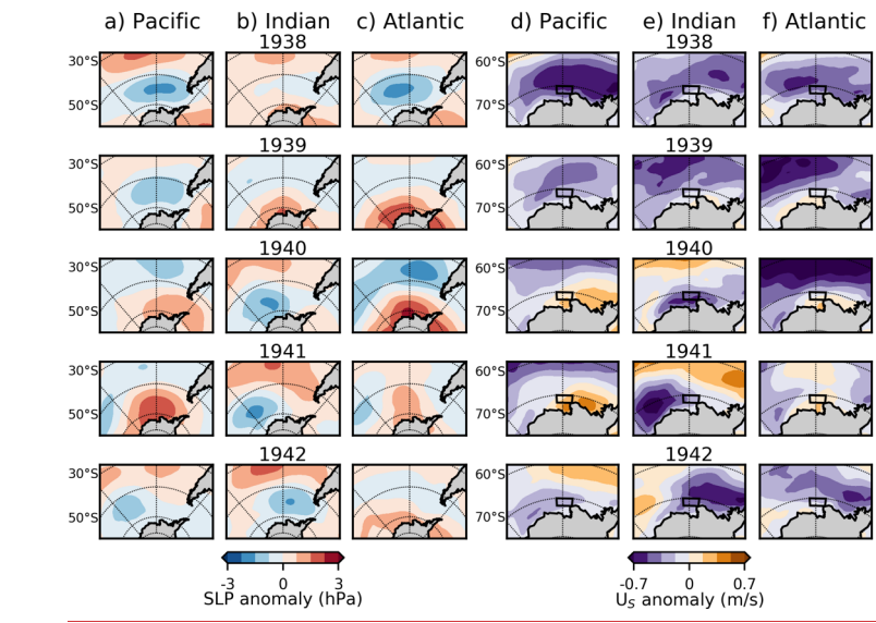
395 Figure 6. Modeled SLP anomalies from 1938 to 1942 in the ensemble mean of the (a) tropical Pacific, (b) Indian Ocean, and (c) North Atlantic pacemaker simulations. (d-f) Same as in a-c, but for U_s anomalies. Anomaly reference period is 1961-1990. We note that the color bar in this figure is smaller than that of Figure 5 due to the smaller
