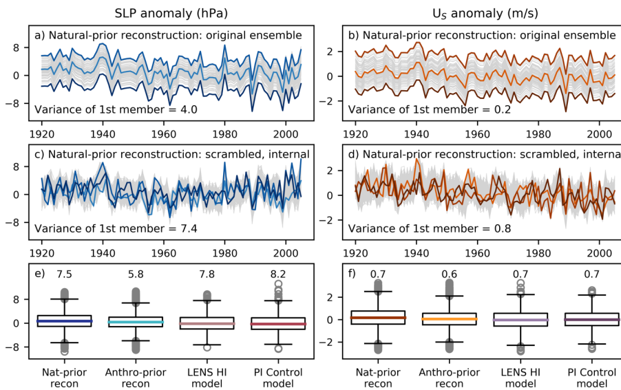
Figure 2. Reconstructed and simulated anomalies in SLP (left panels) and U_s (right panels). (a, b) The original 100 ensemble members in the natural-prior reconstruction. (c, d) The 300 ensemble members in the natural-prior reconstruction ensemble, after scrambling the members and isolating the internal component. All timeseries are in anomalies relative to 1961 to 1990. Only three members in each ensemble are plotted in color to highlight the variability of each member (the members containing the minimum, maximum, and median value during 1940); all other members are plotted in gray. (e, f) Box and whisker plots of all data used to calculate the rarity of the 1940s event: two reconstructions (using the internal component of the scrambled ensembles) and two climate model simulations (the internal component of the LENS historical ensemble (LENS HI) and the Preindustrial Control simulation (PI Control)). The colored lines show the medians, the boxes show the inner quartiles, and gray circles show outliers. The variances of each dataset are shown above each boxplot. The corresponding time series of all datasets are shown in Figure A4.
