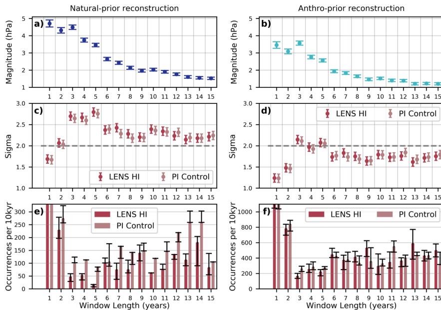
470 Figure 7. Magnitudes of the 1940s SLP event based on 1-to-15-year averaging windows centered around 1940/41, 475 calculated using (a) the natural-prior reconstruction and the (b) anthro-prior reconstruction (in anomalies relative to 1961 to 1990). The circles represent the mean magnitudes and the error bars represent the 95% confidence intervals. (c, d) Sigma levels of each reconstructed magnitude in panels (a) and (b) relative to two climate model simulations: the Preindustrial Control simulation (PI Control) and the internal component of the LENS Historical simulation (LENS HI). The dashed line highlights the 2-sigma level. (e, f) Histograms of the frequency of the 1940s event based on each averaging window, reported as occurrences per 10kyr (using the magnitudes in (a) and (b)) found in the two climate simulations. The error bars represent occurrences based on the upper and lower bounds of the confidence intervals in (a). The y-axes are selected to highlight the rarest events and differ between (e) and (f); the values for all events can be found in Table 1.
