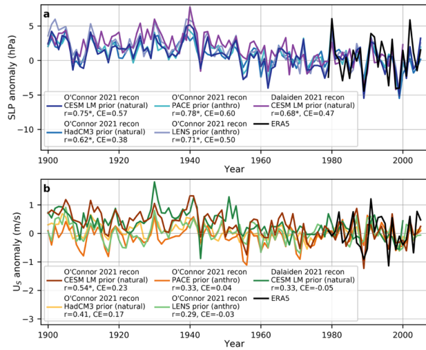
840 Figure A1. SLP and U_s anomalies in the four reconstructions from O'Connor et al. (2021a), the reconstruction from Dalaiden et al. (2021), and ERA5, all averaged over the ASE continental shelf break box shown in Figure 1. For each reconstruction, the climate model simulation used as the data assimilation prior (and whether it include natural or anthropogenic forcing) is shown in the legend. The two reconstructions used in this study are the O'Connor et al. (2021a) CESM LM prior reconstruction (referred to as the natural-prior reconstruction) and the tropical Pacific 845 pacemaker (“PACE”) prior reconstruction (referred to as the anthro-prior reconstruction). Correlation and CE values compared to ERA5 for the period 1979-2000 are also shown in the legend. The anomaly reference period is 1979- 2000 (the period of overlap).
