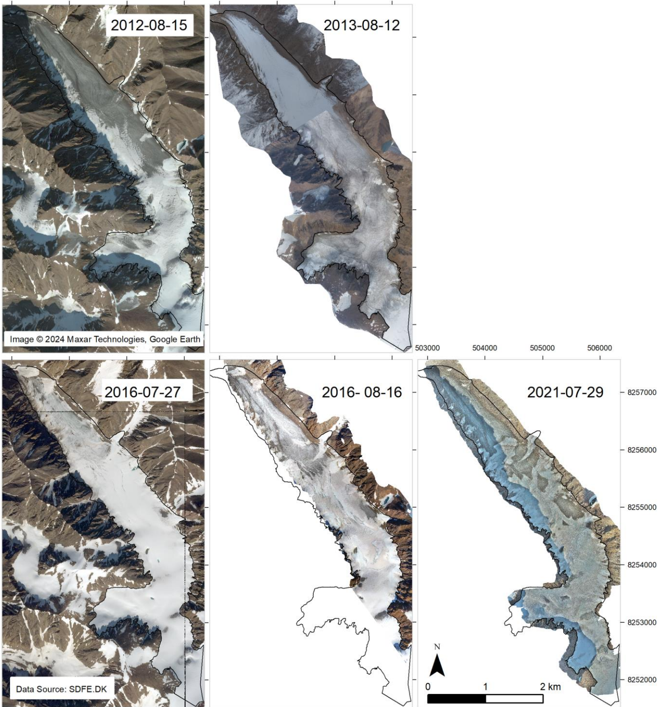
Fig. 10: Orthophotos of Freya Glacier in 2012, 2013, 2016 and 2021.
