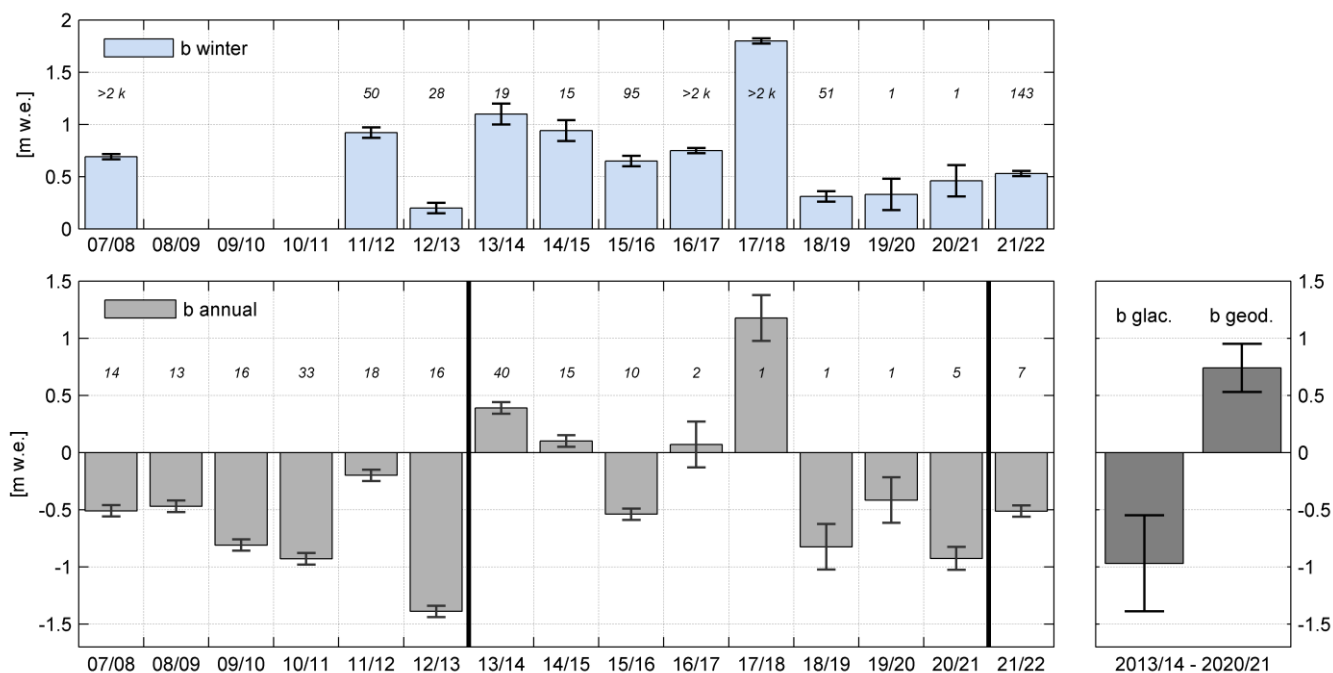
535 Figure 12: Left panels: Time series of specific winter mass balances (top), and specific annual mass balances (bottom) with their estimated uncertainties. The number of point observations available for the mass balance calculation of individual years (winters) is shown as italic numbers. E.g. winter mass balance 2017/18 is based on more than 2000 point observations, while annual balance 2017/18 is based on one point observation only. Right panel: Comparison of the cumulative glaciological and geodetic mass balance 2013/14 – 2020/21 and their related uncertainties.
