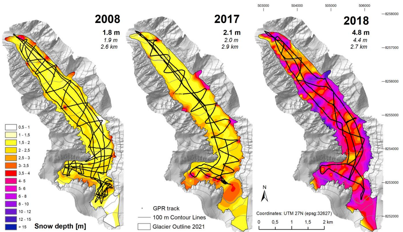
Fig 9: End of winter snow depth maps in years with a detailed GPR survey. Mean snow depth of the interpolated grid is given in bold, arithmetic mean of the individual GPR snow depth points is given in italic. Length of the GPR track is given in km.
