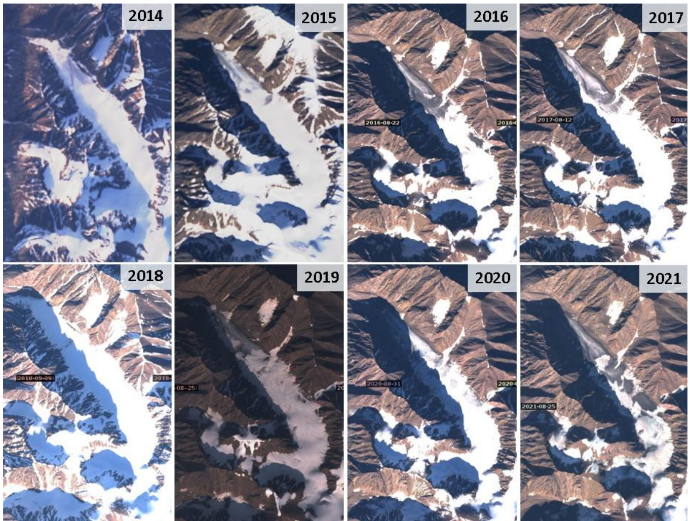
Figure 11: Sentinel 2 (2016-2021) and Landsat (2014-2015) images close to the end of the ablation season show snow cover extent and avalanche affected areas at the end of summer. Landsat images 2014 and 2015 are courtesy of the U.S. Geological Survey. Copernicus Sentinel 2 data 2016-2021, processed by ESA were retrieved from Sentinel Hub.
