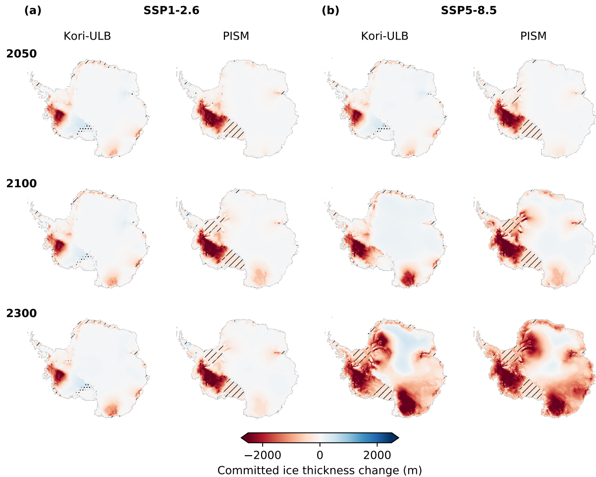
Figure 6. Committed ice-sheet response to changing climate conditions under emission pathways SSP1-2.6 (a) and SSP5-8.5 (b). Shown is the mean ice-thickness change in the year 7000 when stabilizing climatic boundary conditions in the years 2050, 2100 and 2300 (from top to bottom), as determined by the ice-sheet models Kori-ULB (left column) and PISM (right column). For each ice-sheet model, the ice-thickness change is averaged across the applied CMIP6 GCMs and the respective ice-sheet model configurations (Tab. S2). A potential loss of ice shelves is indicated by hatches. Dots mark areas of potential ice-sheet advance.
