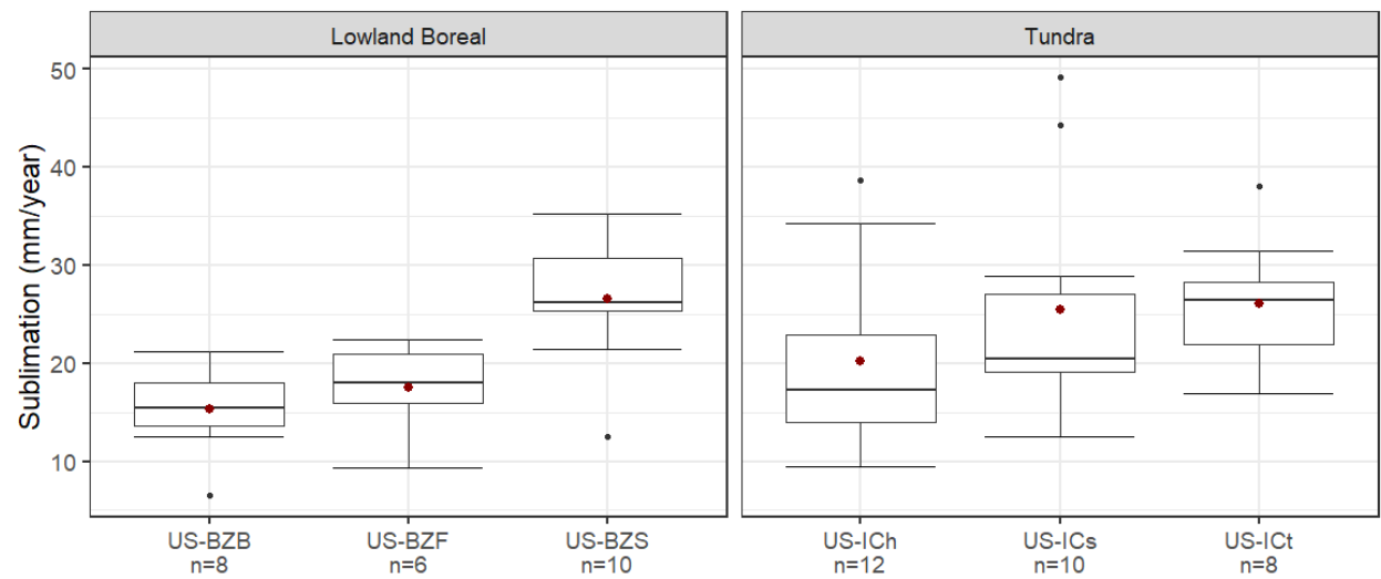
Figure 5: Annual sublimation by site. Red dots represent the mean, boxes enclose the 1 st and 3 rd quartiles, horizontal line within the box is the median, whiskers denote the minimum value below the closest quartile \pm 1.5 \times interquartile range, and points outside the whisker are considered outliers. US-BZB sublimation is significantly different from US-BZS and US-ICt.
