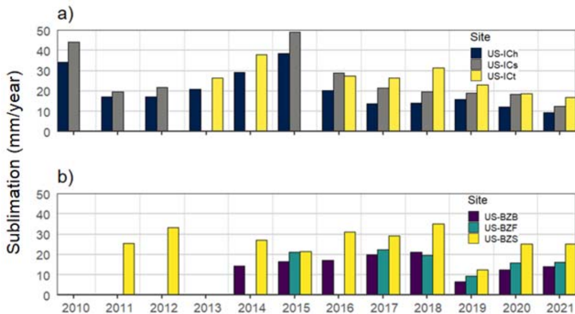
Figure 4: Annual sublimation by water year at tundra sites (a) and lowland boreal forest sites (b).
