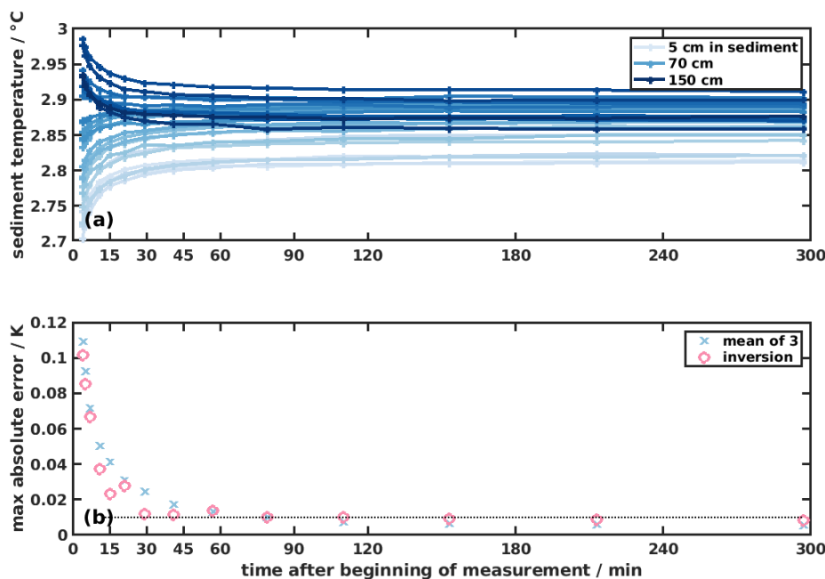
Figure 2. (a) Temperature over time after the beginning of the measurement at Tvillingvatnet , Svalbard, for all sensors. The shade of blue indicates the depth of the sensor in the sediment, with lighter shades at the water-sediment interface and darker shades towards 1.5 m deep in the sediment. Measurements were taken every 60 s. The 14 highlighted points in time (+) indicate the timing of the time periods for which we employed the inversion algorithm. (b) Maximum temperature difference over all sensors for results at different times after the beginning of the measurement. The mean over three measurements after 12 h is assumed as the in-situ temperature, i.e. the reference temperature that the results are compared to. The results from the inversion algorithm are shown in pink circles, means over three measurements are shown in blue crosses, the dotted line indicates the sensor accuracy of 0.01 K.
