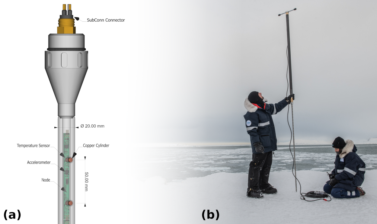
Figure 1. (a) Technical drawing of the head of the temperature lance. A string of 15 nodes is housed inside the lance, with copper cylinders protruding the stainless steel body, connecting the temperature sensors with their surroundings. Two temperature sensors are mounted on each node; on two nodes (at the top and in the middle of the lance) an additional accelerometer is mounted. (b) The temperature lance assembled with one carbon fiber extension for deployment in up to 1.5 m deep water, and connected with a water-proof cable to the logger unit.
