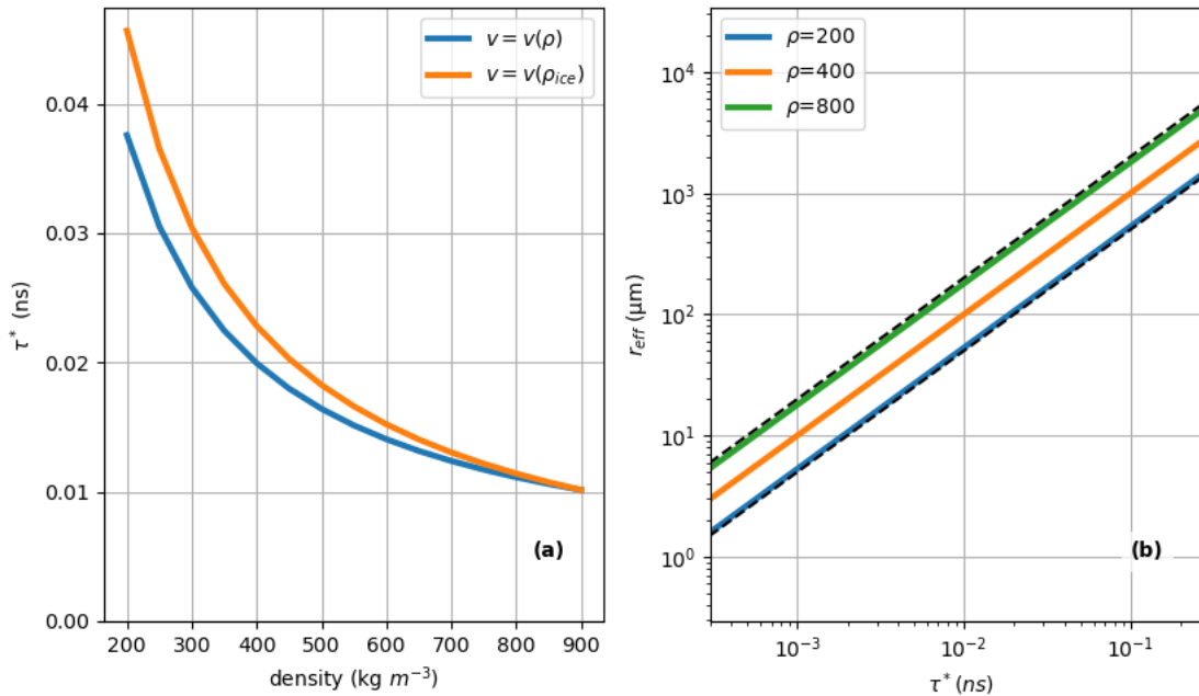
Figure 1. Relation between scattering time, density, and effective grain size. Panel A) shows the relation between scattering time and density for a constant grain size of 200 μm, using a mixing law to calculate the velocity, and using a constant velocity appropriate to solid ice. Panel B) shows the relationship between scattering time and grain size, for three different densities. The dashed black lines show double and half the effective radius for \rho = 400 kg m -3 .
