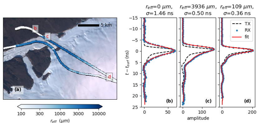
510 Figure 6. Grain size and waveforms. (a) True-color (bands 4, 3, and 2) Landsat image of the Northeast Greenland ice sheet near Leidy Glacier from 6 September, 2019, with estimated effective grain size ( r_{eff} ) from ATM data collected 4 September 2019. For the ATM data, we plot the results of a 100-m blockmedian applied to r_{eff} , and draw the outline of the swath in black. Panels (b), (c), and (d) show measured (RX) and best-fit modeled waveforms (fit), for three locations, as well as the input transmitted pulse (TX), scaled to match the amplitude of the received pulse. Bounding coordinates for panel (a) are presented in table S1. Landsat-8 image courtesy of the U.S. Geological Survey.
