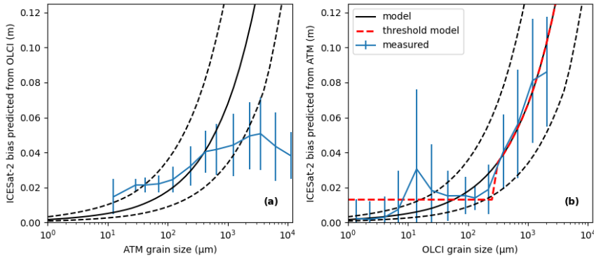
635 Figure 12. Range biases as a function of snow grain-size estimates for the complete 2017-19 dataset. (a) shows range biases predicted from OLCI grain-size estimates as a function of ATM grain size, (b) shows range biases estimated from ATM grain sizes as a function of OLCI grain-size estimates. For each panel, the vertical bars show the standard deviation of the range bias estimates for each grain size value, the black solid curve shows the modeled range bias as a function of grain size, and the dashed lines show the factor-of-two uncertainties in the model related to surface density. The dashed red line in (b) indicates the best fitting threshold model (Eq. 9).
