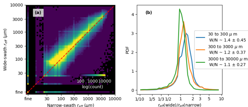
540 Figure 7. Recovered snow grain sizes from two ATM systems from the Summer 2019 campaign. Panel a shows the density of measurements as a function of recovered r_{eff} values from the narrow and wide-scan ATM systems (lighter colors represent a higher density of measurements). Points for which one of the systems found a best match with a scattering-free model waveform are reported along the rows/columns marked ‘fine’. Panel b shows the distribution of wide-to-narrow r_{eff} ratios for different ranges of narrow-swath r_{eff} . The legend for panel b gives the median and robust spread of the ratios for each range.
