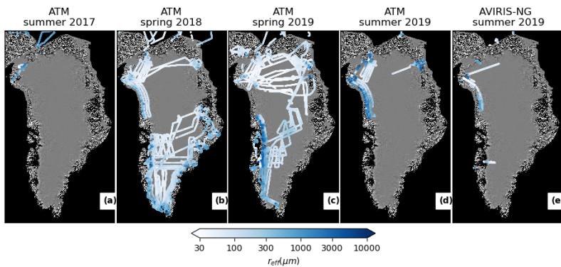
490 Figure 5. Recovered snow grain sizes from ATM and AVIRIS-NG. Colored points indicate recovered grain sizes for four ATM 495 campaigns (a-d) and for AVIRIS-NG (e). Each color-coded points indicates a 1-km block median of recovered grain sizes, and the points have been plotted in order of grain size, so that coarser grain sizes overprint finer grain sizes. Background is the Mosaic of Greenland from 2015 (Haran et al., 2018).
