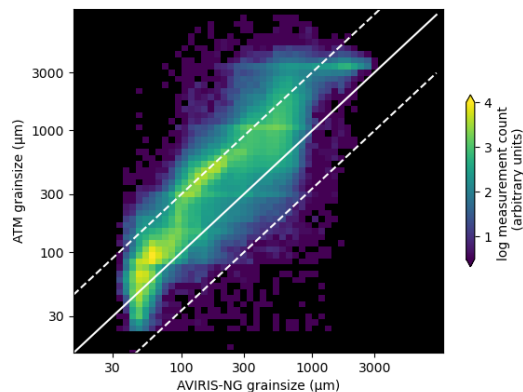
585 Figure 9. [Two-dimensional histogram comparing AVIRIS-NG-derived grain size with narrow-swath ATM-derived grain size, with cells colored by the number of points observed. The solid white line shows the 1:1 relationship between the two datasets]. To help illustrate the magnitude of the difference between the datasets, we plot two dashed lines that show the ATM : 3 x AVIRIS-NG (upper) and ATM : 1/3 x AVIRIS-NG (lower) relationships.
