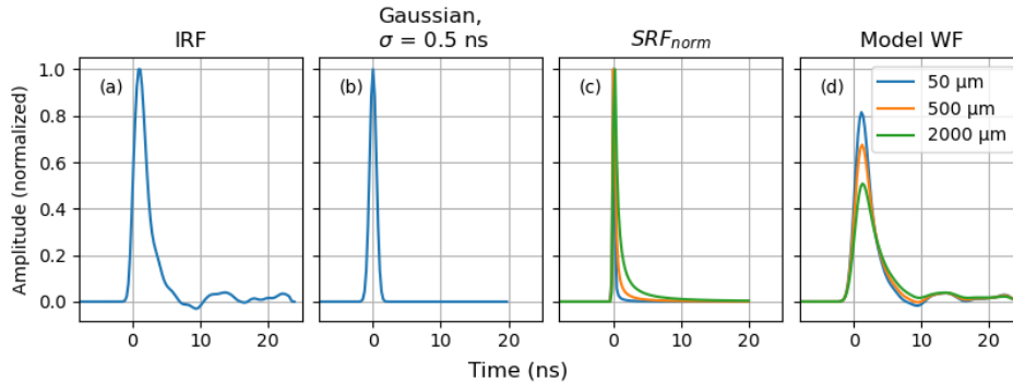
320 Figure 2. Components of the waveform model. The ATM IRF (a) is convolved with a Gaussian function representing surface roughness (b) and the surface response function (c) to produce the model waveform (d). Three SRFs and corresponding waveforms are shown in (c) and (d), for r_{\text{ref}}=50, 500, and 2000 \mu\text{m} . Curves in (a-c) are normalized to unit amplitude, curves in (d) are based on an IRF with with unit amplitude.
