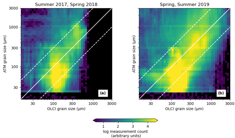
615 Figure 11. Comparison between narrow-swath-ATM-derived and OLCI-derived grain-size estimates. Panel A shows the distribution for the summer (July) of 2017 and the spring (March-May) of 2018, Panel B shows the distribution from the spring (April-May) and summer (September) of 2019. In both plots, the ATM grain sizes are derived from a 10-meter blockmedian of the data, and only those points for which the time difference between the OLCI measurement and the ATM measurement was less than 3 days are included. The solid lines indicates the 1:1 relationship between the datasets, the dashed lines indicate the 1:3 and the 3:1 relations. 620
