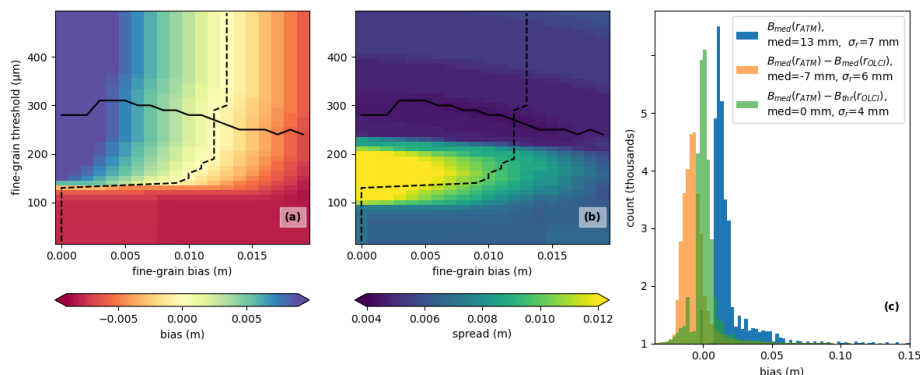
730 Figure 13. Tuning the threshold correction for ATM-based ICESat-2 bias estimates. Panels (a) and (b) show the median and robust spread of the distribution of ATM-derived ICESat-2 bias estimates corrected with the threshold model (Eq. 9) for different values of the fine-grain bias ( B_0 ) and fine-grain threshold ( r_{thr} ). The dashed curves show the fine-grain bias corresponding to the minimum absolute value of the median for each value of the threshold, and the solid lines show the fine-grain threshold corresponding to the minimum value of the spread for each value of the fine-grain bias. Panel (c) shows histograms of uncorrected bias estimates, bias estimates corrected based on B_{med}(r_{OLCI}) (Eq. 8) and bias estimates corrected based on B_{thr}(r_{OLCI}) (Eq. 9) for the optimum parameters, B_0=0.012 m, r_{thr}=270 \mu\text{m} . The median and robust spread of each distribution is given in the legend.
