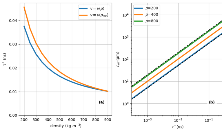
250 Figure 1. Relation between scattering time, density, and effective grain size. Panel A) shows the relation between scattering time and density for a constant grain size of 200 \mu\text{m} , using a mixing law to calculate the velocity, and using a constant velocity appropriate to solid ice. Panel B) shows the relationship between scattering time and grain size, for three different densities. The dashed black lines show double and half the effective radius for \rho = 400 \text{ kg m}^{-3} .
