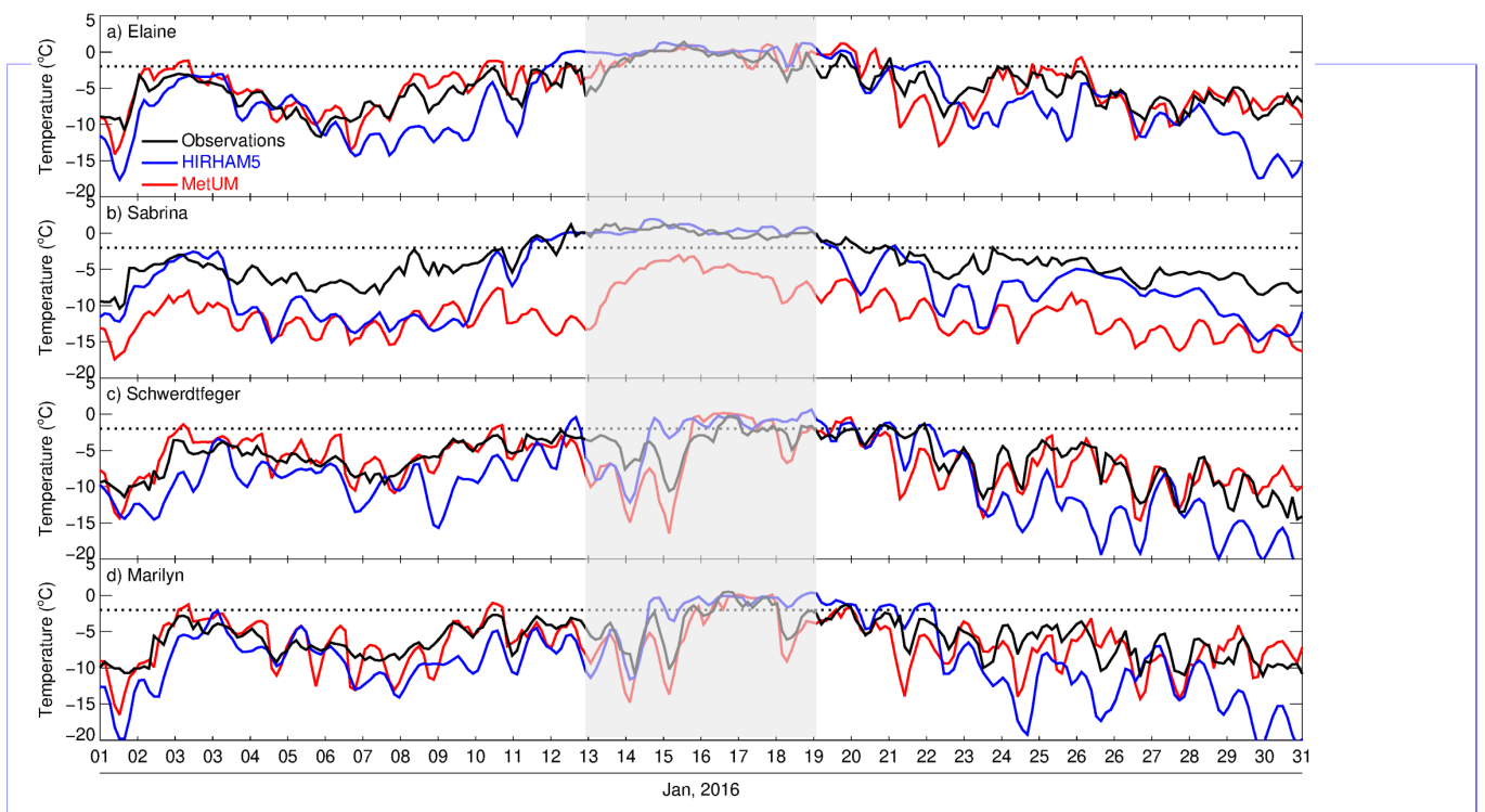
Figure 4. Timeseries of near-surface air temperature ( ^{\circ}\text{C} ) from the 1 st to 31 st of January 2016 from AWS measurements (black line), HIRHAM5 output (blue line), and MetUM output (red line) at (a) Elaine, (b) Sabrina, (c) Schwerdtfeger, and (d) Marilyn. The period of special interest from 13 th to 18 th of January is highlighted by the semi-transparent shaded region. The date shown is in UTC, with local time for the Ross Ice Shelf 12 hrs ahead of UTC. The horizontal dotted line shows temperatures at -2^{\circ}\text{C} , which Nicolas et al. (2017) suggests is the threshold for melting for this particular event.
