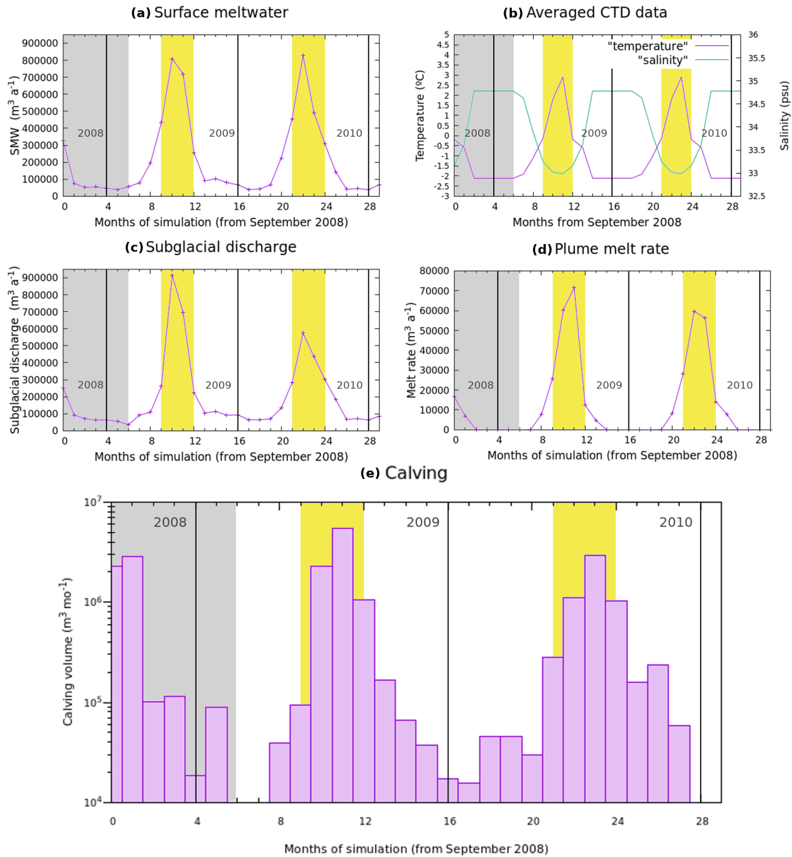
Figure 4. Temporal evolution of: (a) surface meltwater (SMW), (b) average temperature and salinity of the fjord water near the calving front , (c) subglacial discharge produced by surface and basal melt for every month of the simulation , (d) total melt rate produced by plume activity computed on the first day of every month of the simulation and (e) the number of calving events volume produced by the model at for every month of the simulation (log scale) . The shaded areas correspond to the initialization period . The yellow areas indicate the summer periods (June to September 2009 and 2010) and the black vertical lines separate the different years.
