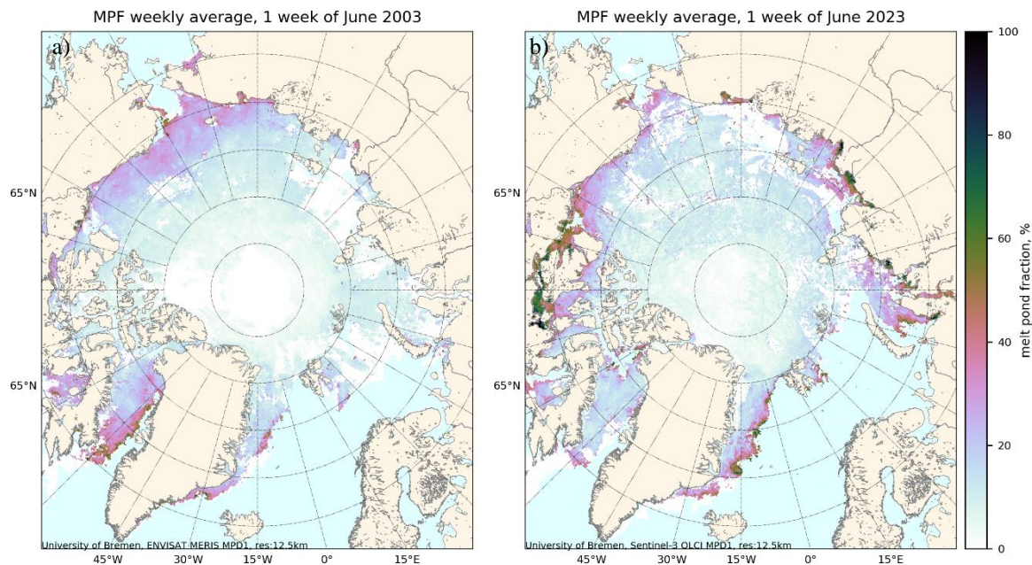
Figure 9: Weekly averages for (a) the first week of June 2003, MERIS MPD and (b) the first week of June 2023, OLCI 410 MPD. Note the MPF differences in the Canadian Arctic Archipelago and Kara and Laptev Sea.
