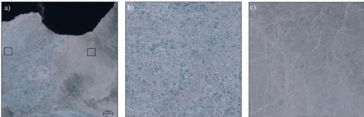
295 Figure 5: (a) RGB of the second full-resolution comparison case on 01.06.2021, MSI tile T53XMD, UTC Time 03h35'39", relative orbit = R004. (b) RGB subset for the left square on (a), (c) RGB subset for the right square on (a).
