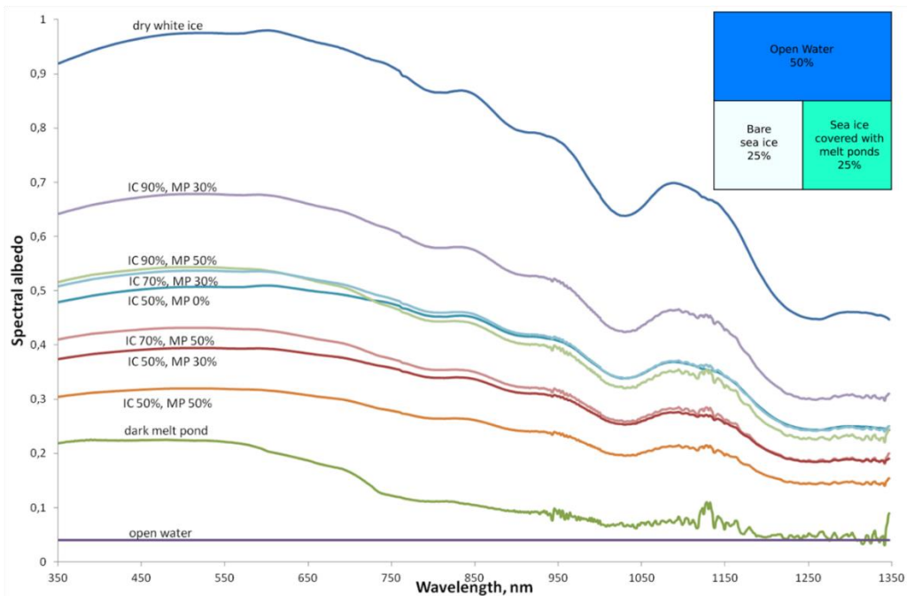
Figure 8: Linear mixture of in situ measured spectra of white ice and dark melt pond as the most frequent Arctic scenario. Moderate resolving spectroradiometers with optical and NIR bands will not be able to distinguish the influence of MPF from the influence of open water (OW) for ice concentrations (IC) < 90 %. Spectral data for dark melt pond and dry white ice is taken from Istomina et al. (2016), open water is assumed to have a constant spectral albedo of 0.04.
