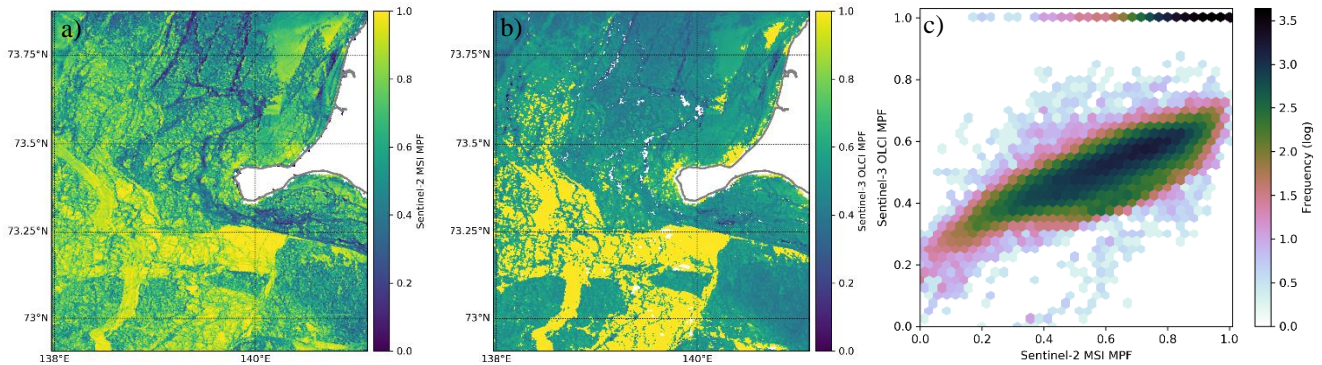
Figure 4: (a) MSI MPF for the case in Fig. 3a, (b) corresponding OLCI MPF, OLCI granule from 01.06.2021, time UTC 01h31'48", cycle number 072, relative orbit 231, 300m resolution, (c) density plot of OLCI MPF correspondence to MSI MPF. Note the bimodal OLCI MPF for MSI MPF = 1.
