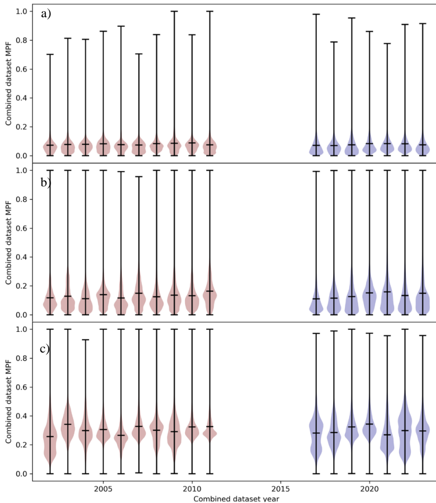
430 Figure 10: MPF distributions of the hemispheric weekly averages for (a) the first week of May, (b) the first week of June, 435 (c) first week of July of the combined MERIS (red) and OLCI (blue) dataset. The histogram of the data is shown by the color thickness.
