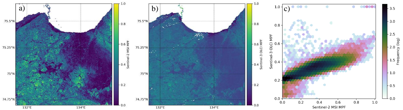
Figure 6. (a) MSI MPF for the case in Fig. 5a, (b) corresponding OLCI MPF, OLCI granule from 01.06.2021, time UTC 01h31'48", cycle number 072, relative orbit 231, 300m resolution, (c) density plot of the OLCI MPF correspondence to MSI MPF. Note the bimodal OLCI MPF for MSI MPF < 0.1.
