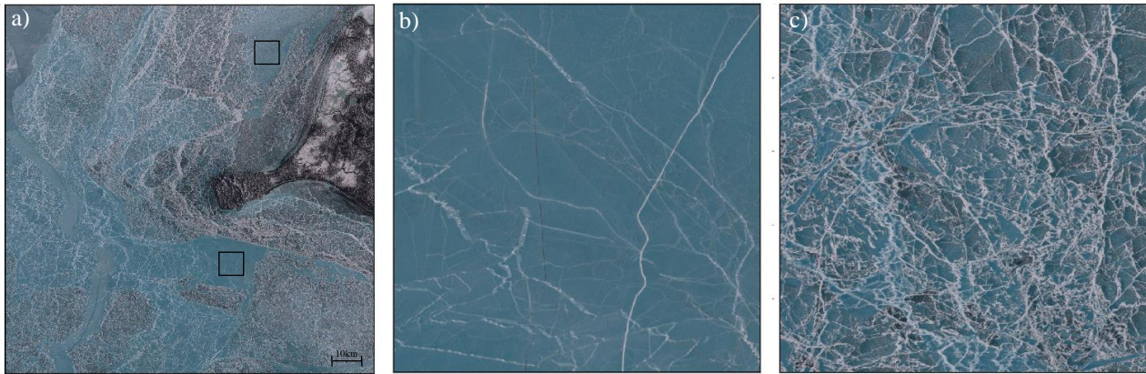
Figure 3: (a) RGB of the first full-resolution comparison case on 01.06.2021, MSI tile T54XVG, UTC Time 03h05'49", relative orbit = R075, at landfast ice in the Laptev Sea, (b) RGB subset for the bottom square on (a), (c) RGB subset for the top square on (a).
