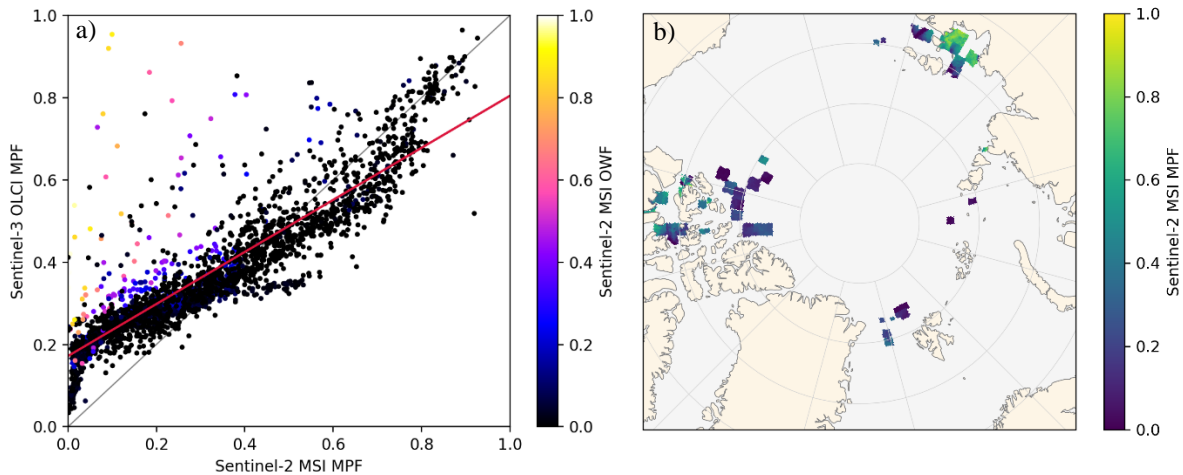
335 Figure 7: Evaluation of the daily gridded OLCI MPF dataset. (a): the comparison of the MSI MPF to OLCI MPF in relation to the fraction of open water as seen by MSI, R = 0.86 , N = 3152 , RMSD = 0.13 , intercept = 0.17, slope = 0.63. (b): the spatial distribution of the MSI validation data used in (a), sensing time 2017–2023, see Table 2 for details on the used MSI dataset.
