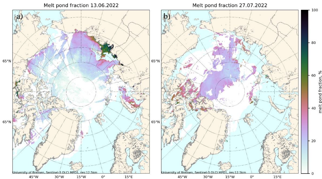
205 Figure 2: Example of the daily gridded MPD product for the 13.06.2022 and the 27.07.2022. Note the variable MPF on 13.06.2022 during the melt onset and the uniform MPF during the evolution of melt on 27.07.2022. The white areas depict the cloud covered sea ice where no MPF retrieval is possible. Sea ice coverage is given by ARTIST Sea Ice (ASI) PM sea ice concentration product (Spreen et al., 2008).
