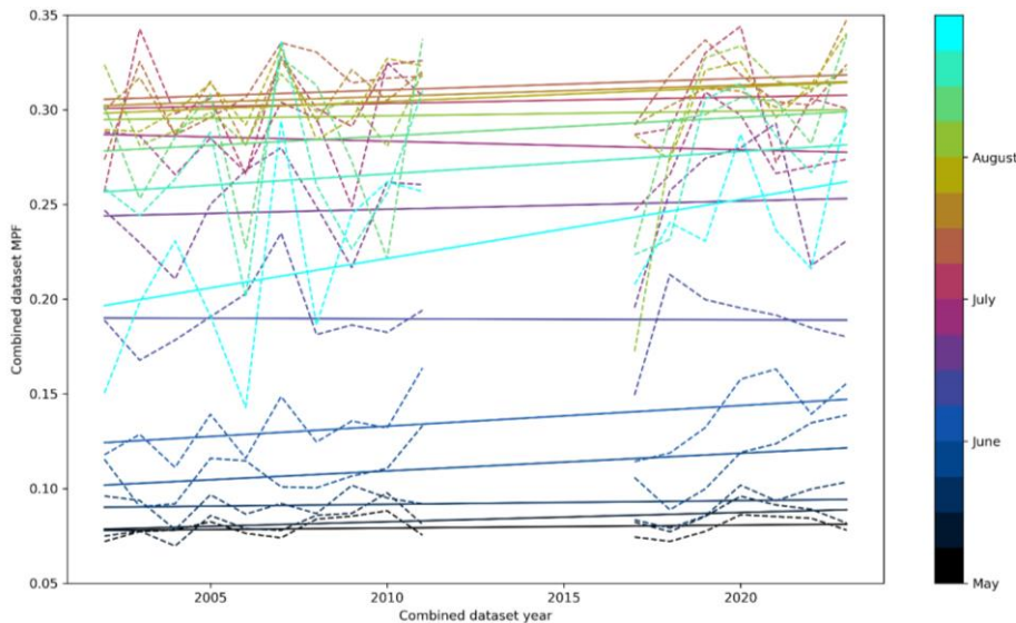
Figure 12: Weekly hemispheric MPF trends of the combined MERIS and OLCI dataset.
