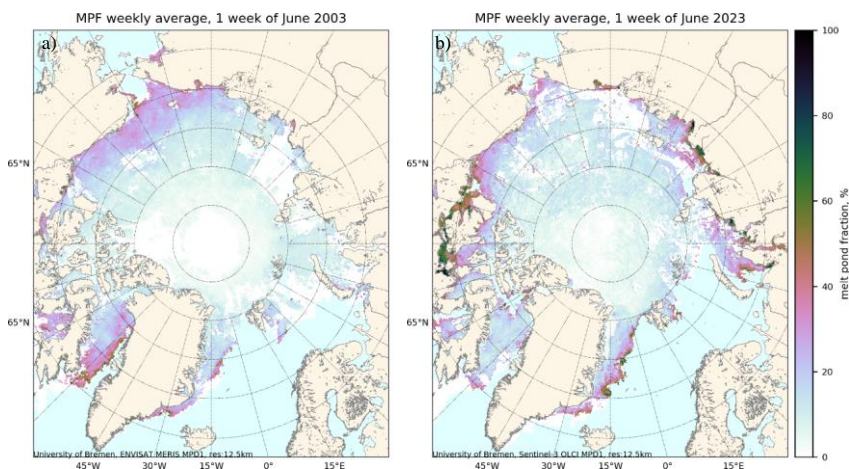
415 Figure 8: Weekly averages for (a) the first week of June 2003, MERIS MPD and (b) the first week of June 2023, OLCI MPD. Note the MPF differences in the Canadian Arctic Archipelago and Kara and Laptev Sea.
