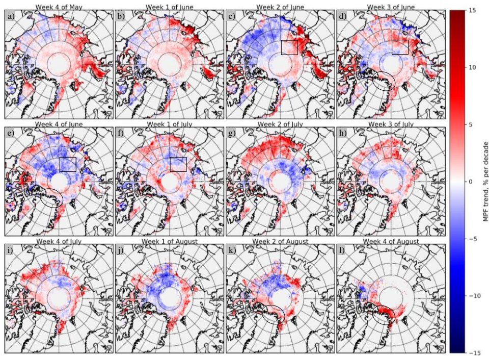
485 Figure 10: Weekly MPF trends of the combined MERIS and OLCI dataset 2002–2023 (data 2012–2016 not available).
