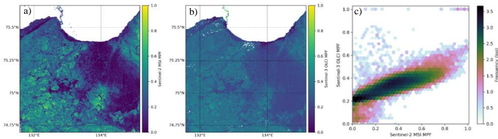
300 Figure 5: (a) MSI MPF for the case in Fig. 4a, (b) corresponding OLCI MPF, OLCI granule from 01.06.2021, time UTC 01h31'48", cycle number 072, relative orbit 231, 300m resolution, (c) density plot of the OLCI MPF correspondence to MSI MPF. Note the bimodal OLCI MPF for MSI MPF < 0.1.
