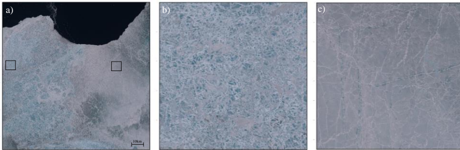
295 Figure 4: (a) RGB of the second full-resolution comparison case on 01.06.2021, MSI tile T53XMD, UTC Time 03h35'39", relative orbit = R004. (b) RGB subset for the left square on (a), (c) RGB subset for the right square on (a).
