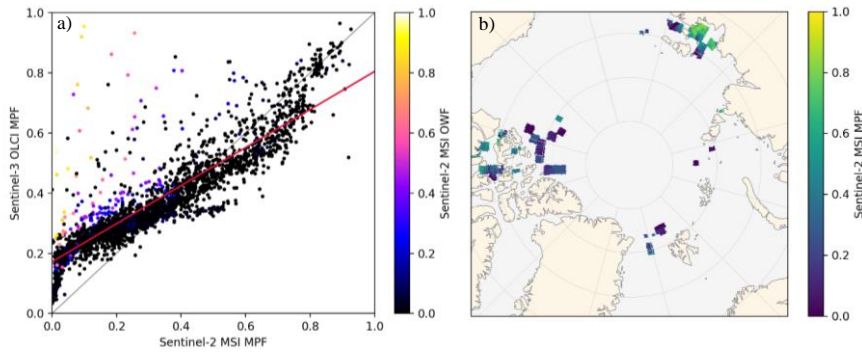
340 Figure 6: Evaluation of the daily gridded OLCI MPF dataset. (a): the comparison of the MSI MPF to OLCI MPF in relation to the fraction of open water as seen by MSI, R = 0.86 , N = 3152 , RMSD = 0.13 , intercept = 0.17 , slope = 0.63 . (b): the spatial distribution of the MSI validation data used in (a), sensing time 2017–2023, see Table 2 for details on the used MSI dataset.
