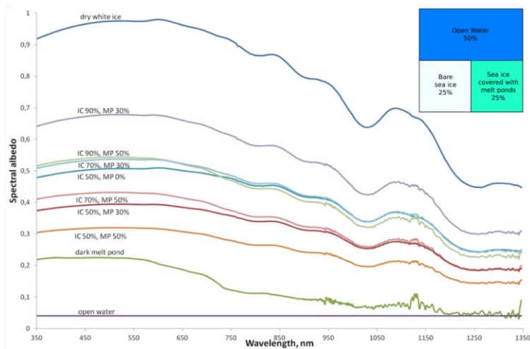
345 Figure 7: Linear mixture of in situ measured spectra of white ice and dark melt pond as the most frequent Arctic scenario. Moderate resolving spectroradiometers with optical and NIR bands will not be able to distinguish the influence of MPF from the influence of open water (OW) for sea-ice concentrations (IC) < 90 %. Spectral data for dark melt pond and dry white ice is taken from Istomina et al. (2016), open water is assumed to have a constant spectral albedo of 0.04.
