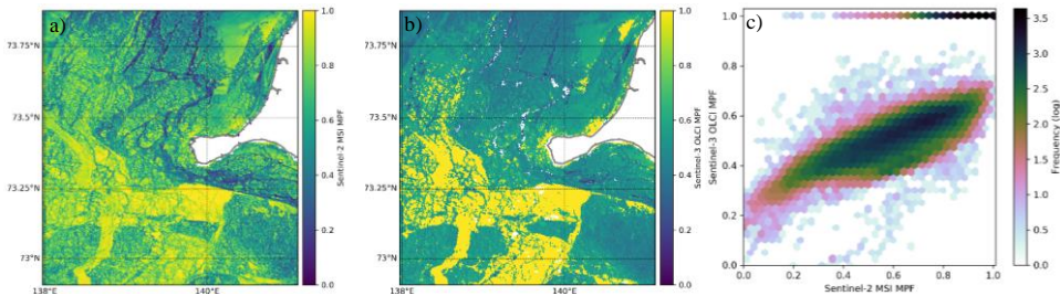
230 Figure 3: (a) MSI MPF for the case in Fig. 2a, (b) corresponding OLCI MPF, OLCI granule from 01.06.2021, time UTC 01h31'48", cycle number 072, relative orbit 231, 300m resolution, (c) density plot of OLCI MPF correspondence to MSI MPF. Note the bimodal OLCI MPF for MSI MPF = 1.
