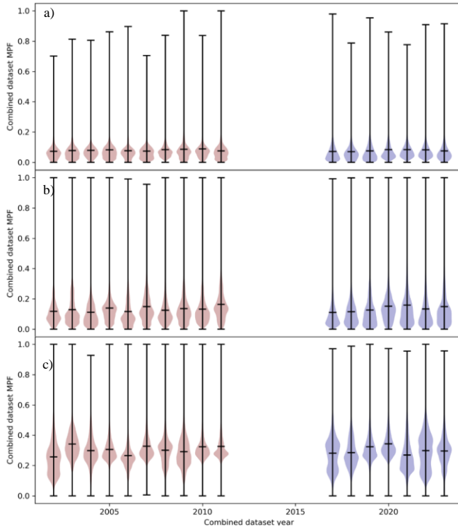
435 Figure 9: MPF distributions of the hemispheric weekly averages for (a) the first week of May, (b) the first week of June, (c) first week of July of the combined MERIS (red) and OLCI (blue) dataset. The histogram of the data is shown by the color thickness.
