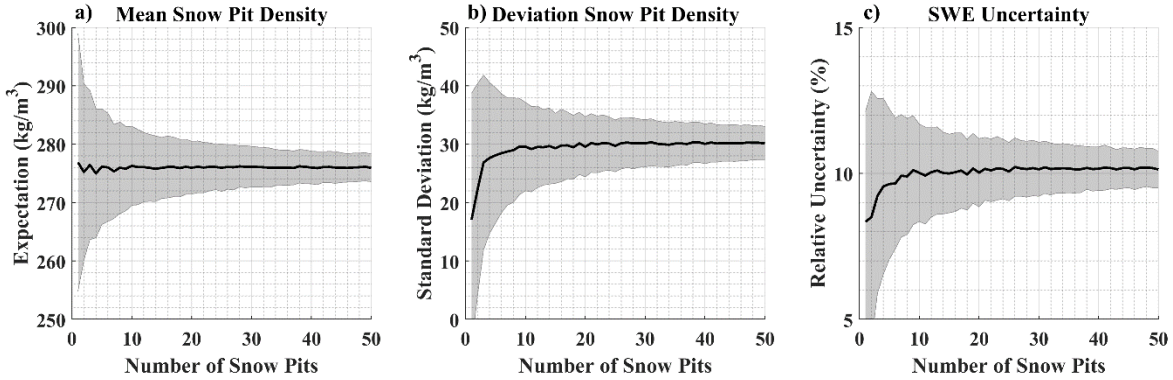
980 Figure B.3: Monte Carlo uncertainty analysis for a) mean snow density, b) standard deviation of snow density, and c) propagated SWE uncertainty as functions of sample size.
