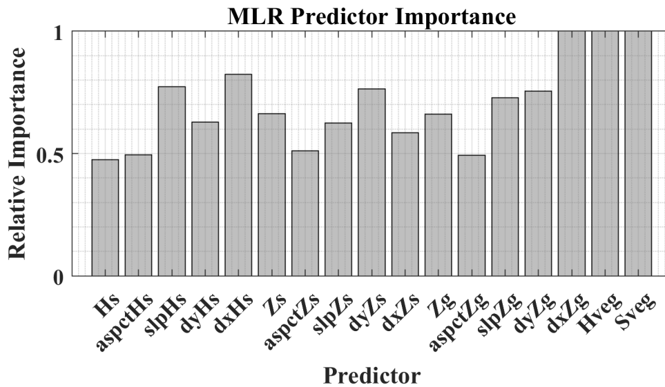
Figure A.1: The relative importance of the LiDAR derived predictors: Hs snow depth, aspectHs aspect of snow depth, slpHs slope of snow depth, dyHs north component of snow depth gradient, dxHs east component of snow depth gradient, Zs the snow surface elevation and derivatives, Zg the ground elevation and derivatives, Hveg vegetation height, and Sveg the distance to vegetation with height greater than 0.5 m. The predictor importance was determined from the top 1 % of models.
