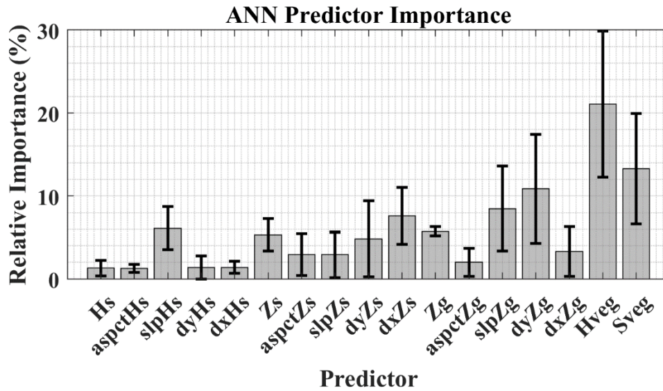
970 Figure A.3: Relative importance of LiDAR predictors within the ANN comprised of two hidden layers.
