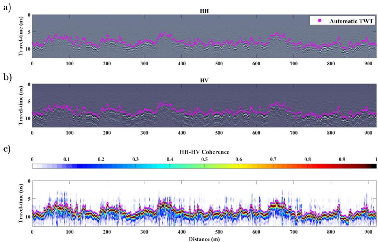
Figure 23: A 900 m GPR transect with autopicks in magenta for a) HH and b) HV profiles of travel time, and c) the coherence of these radargrams (Equations 1, 2).
