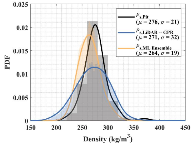
Figure B.12: Histograms of the snow pit measured, LiDAR – GPR inferred retrieved , and regression model ensemble densities.
