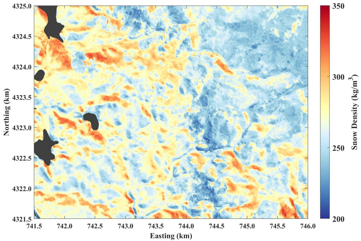
Figure 67: Snow density was distributed spatially using the ML regression ensemble average ( b_{s, LiDAR - \overline{E_{NS}}} ) regression techniques a) MLR, b) RF, and c) ANN based on predictive features that were derived solely from LiDAR information (i.e. snow depth, elevation, slope, aspect, and vegetation) and d) a synthesised random field model from the statistics of in-situ density measurements ( 275 \pm 20 \text{ kg/m}^3 ) and the correlation length of snow density estimated via variogram analysis.
