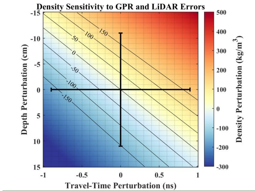
Figure B.13: Perturbations were added to the mean values 8 ns TWT and 96 cm depth then the density was evaluated to estimate potential errors resulting from sensor integration (coloured area and contours). The error bars represent the RMSE of LiDAR evaluated by probing (11 cm) and the RMSD of the GPR TWT crossovers (0.9 ns). At one standard deviation, combined snow density errors of + 150 kg/m 3 can be expected from sensor integration, which are reduced to within + 30 kg/m 3 by outlier filtering.
