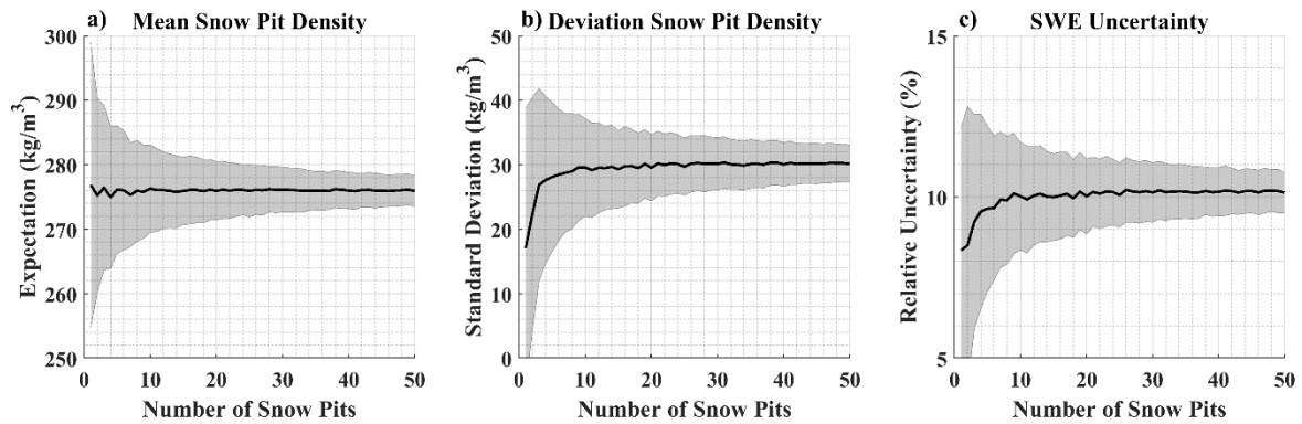
Figure B.32: Monte Carlo uncertainty analysis for a) mean snow density, b) standard deviation of snow density, and c) propagated SWE uncertainty as functions of sample size.
