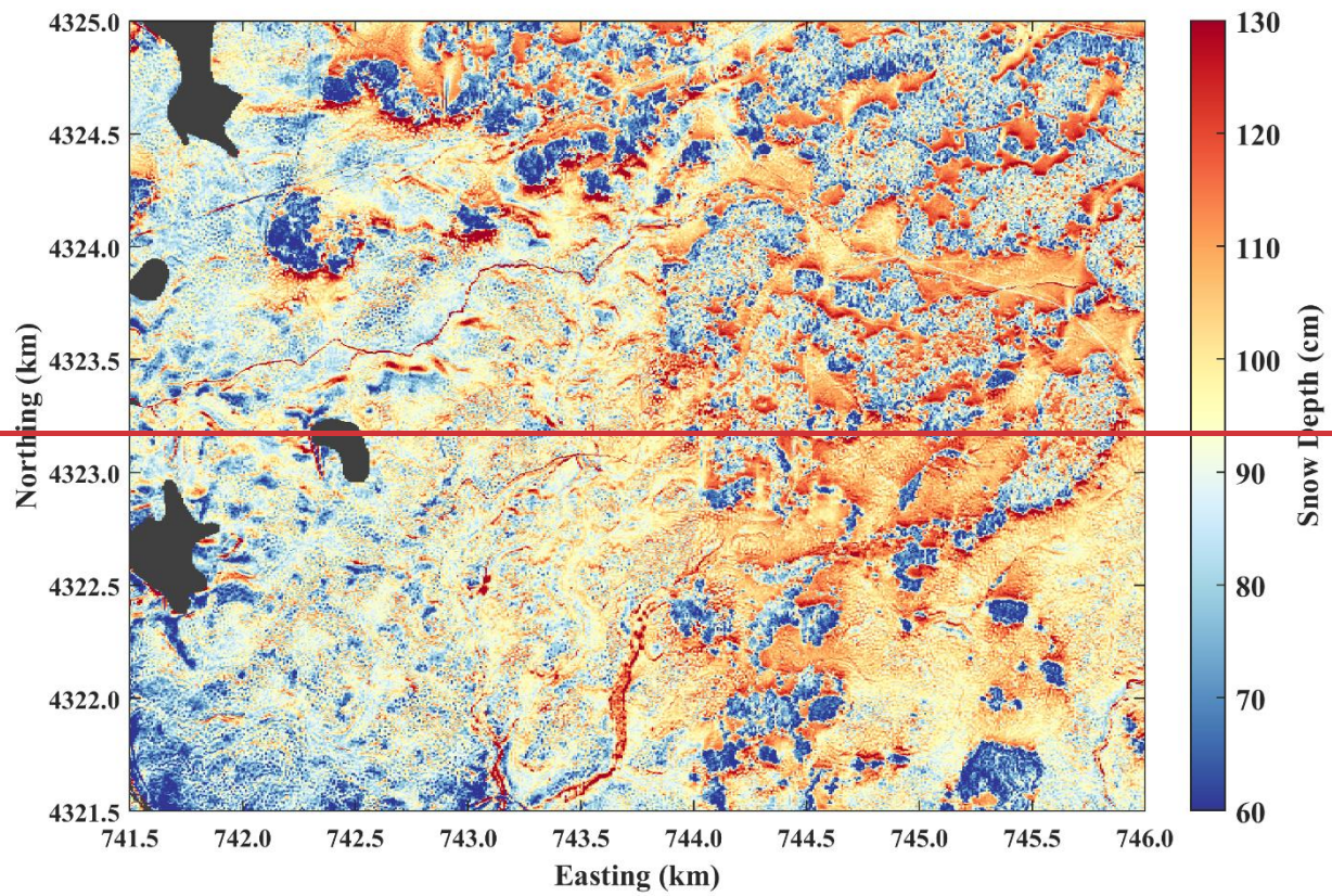
Figure 4: One-metre resolution snow depths from the February 1, 2020 LiDAR flight. The western half of the domain is relatively unforested, shrub steppe (lakes are masked black) while the eastern half has stands of dense forest (see Fig. 1).
