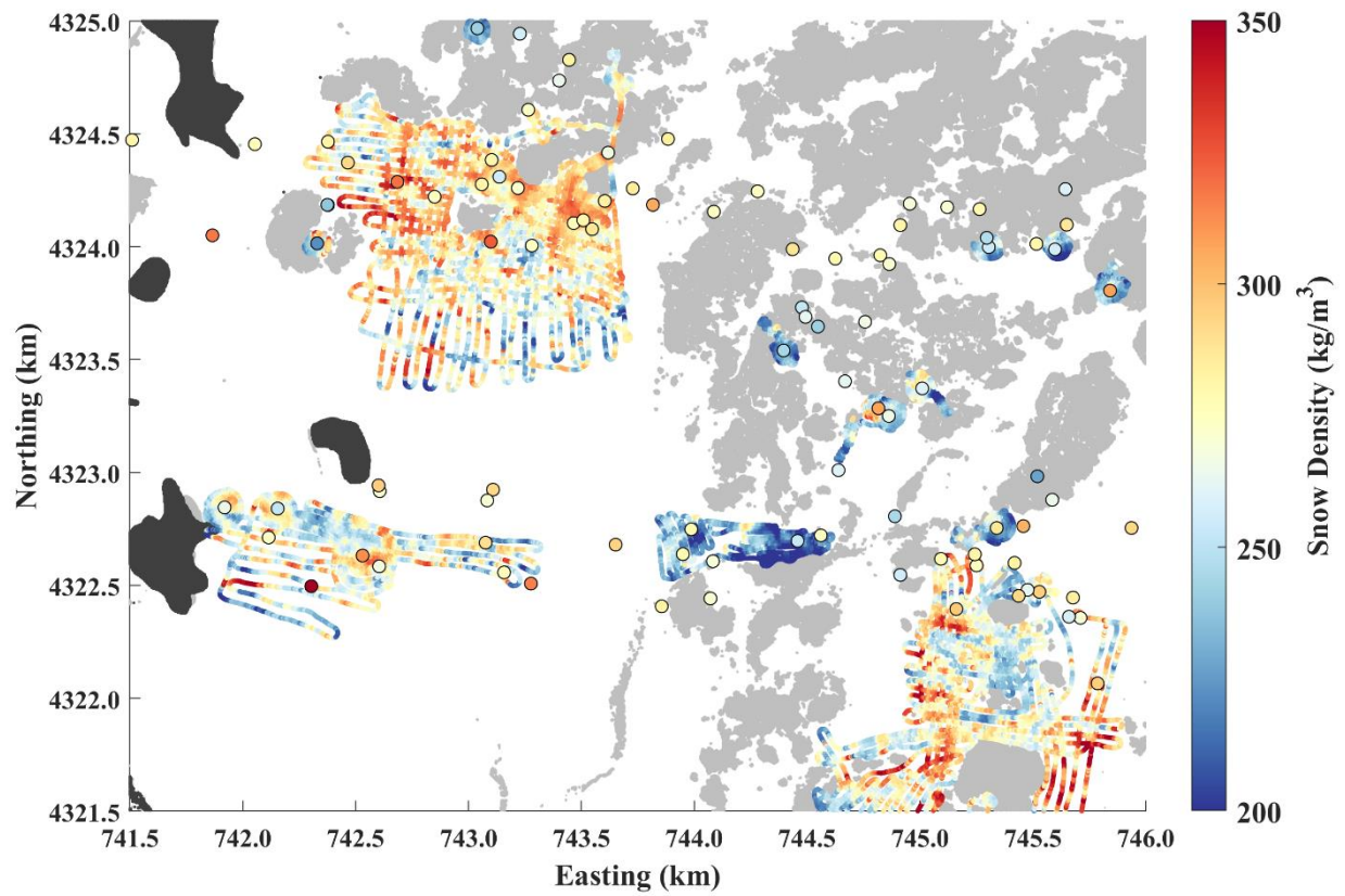
Figure 45: Bulk snow density along radar profiles estimated by combining LiDAR snow depths with GPR TWTs. Average density measured in the 96 snow pits within the LiDAR boundary are overlaid as larger markers. Forested areas (grey) and lakes (black) are shown.
