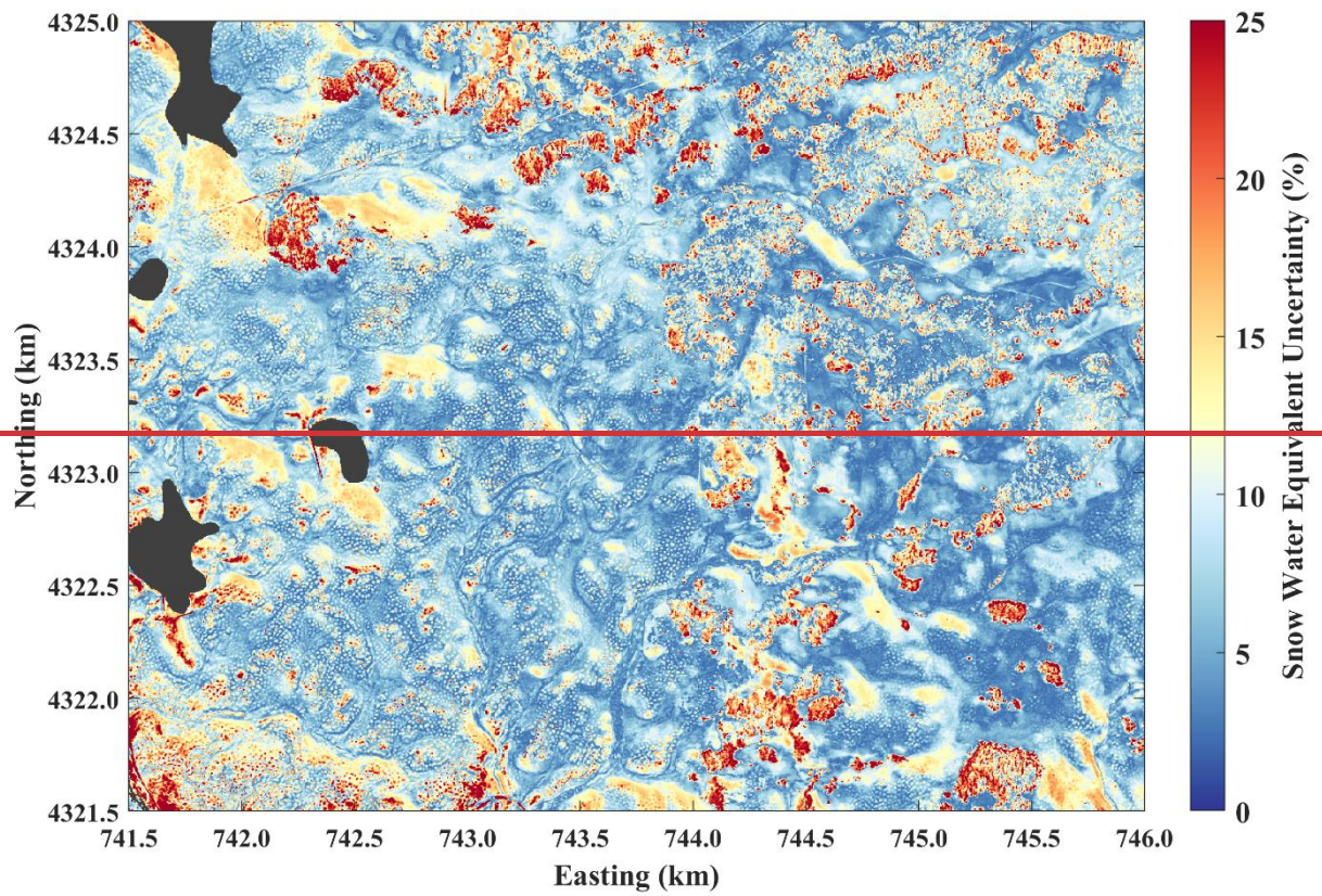
Figure 10: Estimated uncertainty in snow water equivalent from the propagation of errors in snow depth and density. The spatial distribution of uncertainty tends to be greatest in the shallower and lower density snow underneath tree canopies and least in the deepest snow caught in drifts around the perimeters of forest stands.
